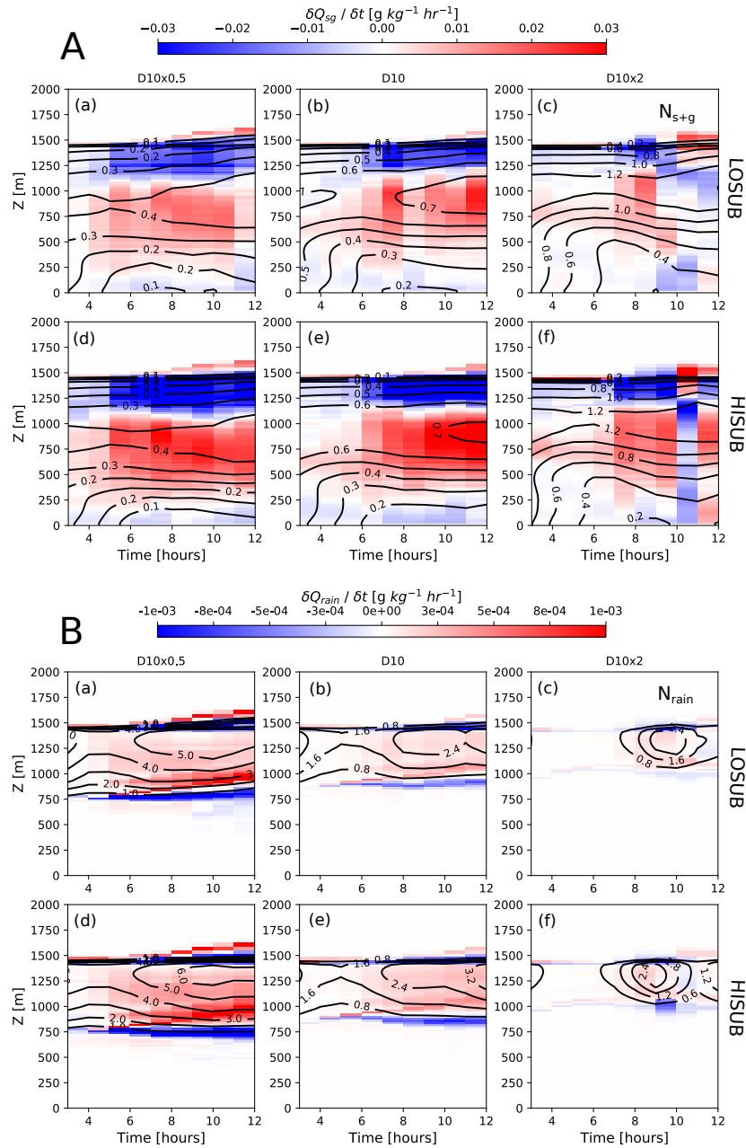
Figure 7. As Fig. 5, instead the ice number concentration is varied (test 3).
