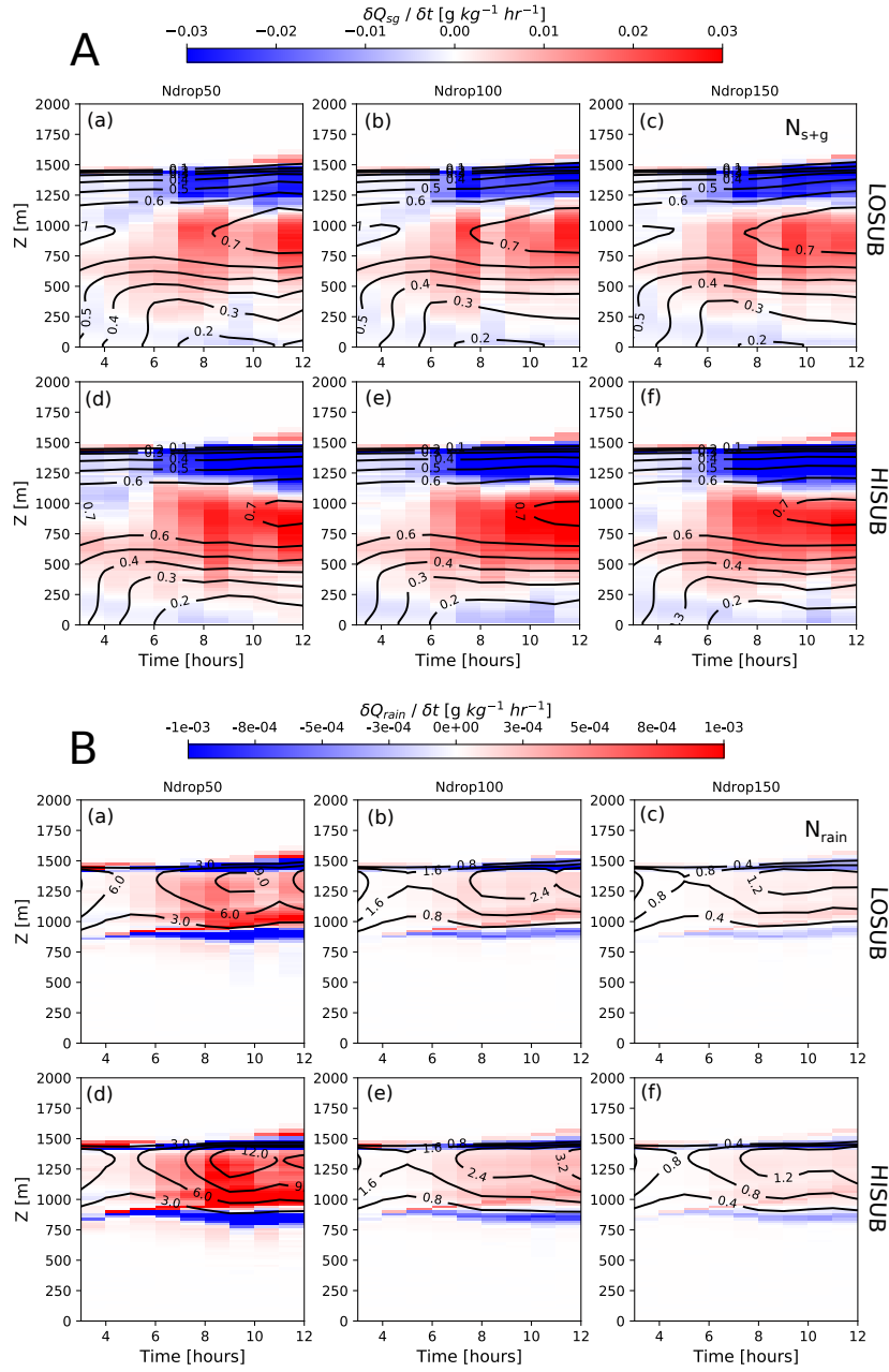
Figure 5. A: Change in \delta Q_{sg}/\delta t [g kg -1 hr -1 ] (shading) between subsidence cases and the corresponding CNTRL simulation for test 2. Red corresponds to increased production, whilst blue shows increased sublimation than the associated CNTRL. N_{sg} [L -1 ] is shown as contours. B: As panel A, instead the change in \delta Q_{rain}/\delta t [g kg -1 hr -1 ] is shown with N_{rain} [L -1 ] as contours. (a-c): LOSUB, (d-f): HISUB.
