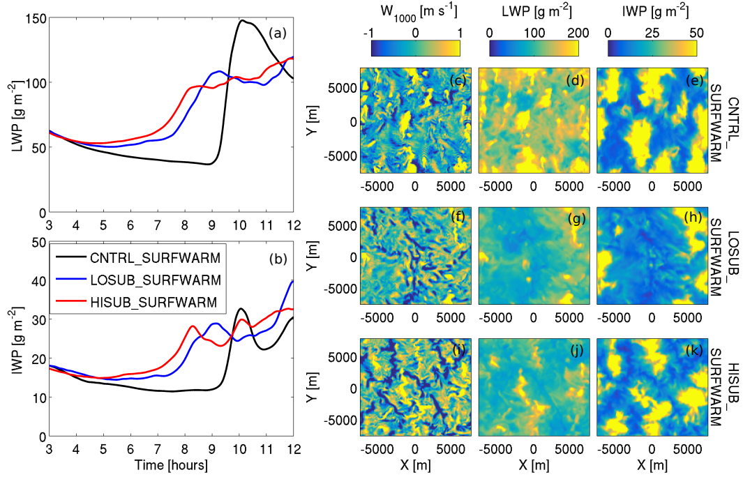
Figure 9. As Fig. 2, with the addition of a warming surface (test 4). Planar views (c–k) are shown at 10 h to capture the bulk cloud structure coinciding with the CNTRL_SURFWARM peak in LWP and IWP shown in panels a and b.
