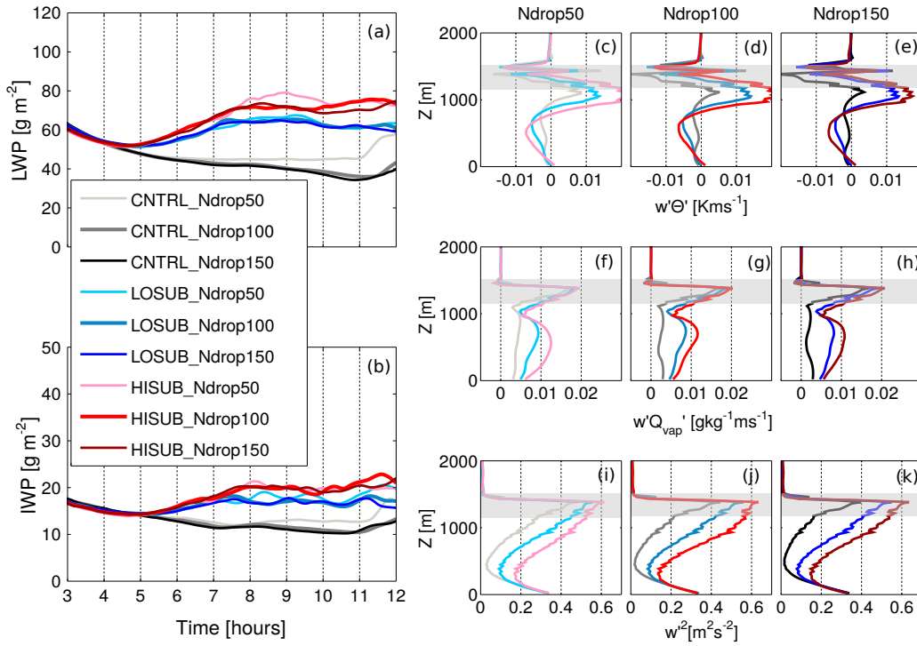
Figure 4. Domain-averaged LWP (a) and IWP (b) time series for simulations with different N_{\text{drop}} while varying the imposed W_{\text{sub}} . Black: Control cases, blue: low W_{\text{sub}} , red: high W_{\text{sub}} . (c-e): buoyancy flux ( w'\Theta' ), (f-h): water vapour flux ( w'Q_{\text{vap}}' ), (i-k): vertical velocity variance ( w^2 ). Vertical profiles shown at 9 h.
