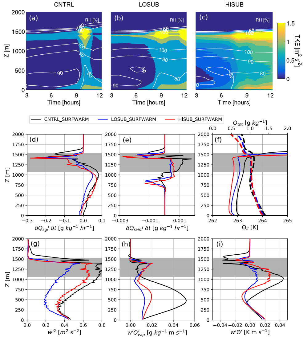
Figure 10. As Fig. 3, with the addition of a warming surface (test 4). Note the different colour scale in panels a–c, and extended x-range over which data is shown in all panels except f, with comparison to Fig. 3. Vertical profiles (panels d–i) are shown at 10h.
