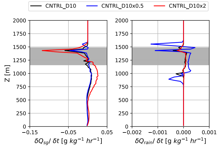
Figure 8. Microphysical tendencies comparison of CNTRL_D10, CNTRL_D10x0.5, and CNTRL_D10x2. Vertical profiles, at 9 h, of solid precipitation (snow + graupel) mass tendency ( \delta Q_{\text{sg}}/\delta t ) and rain mass tendency ( \delta Q_{\text{rain}}/\delta t ) are shown. Area in grey represents CNTRL_D10 cloudy regions.
