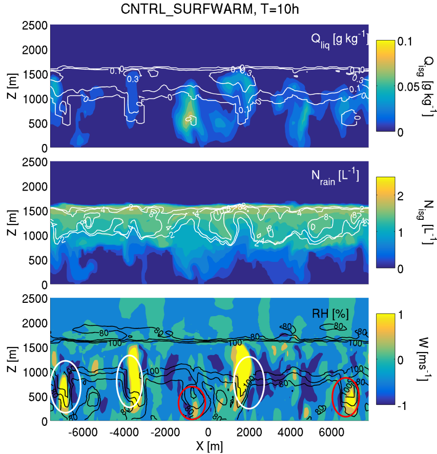
Figure 11. Z-X slices for the CNTRL_SURFWARM case at 10 h. Top row: total ice mass mixing ratio ( Q_{ice} , shading) and liquid water mass mixing ratio ( Q_{liq} , contours). Middle row: total ice number concentration (ice+snow+graupel, N_{ice} , shading) and rain number concentration ( N_{rain} , contours). Bottom row: vertical velocity ( W , shading) and relative humidity (RH, contours). Identified detached below-cloud cumuli are highlighted by red ellipses, and cumuli merged with the Sc are indicated by white ellipses.
