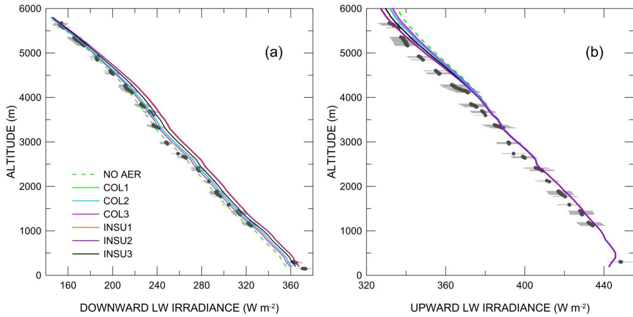
Figure 6: (a) downward and (b) upward LW irradiance profiles for F35. Grey dots are the measurements selected for small pitch and roll angles, with the associated uncertainty (one sigma) in light grey. Simulated profiles with different SDs and RIs are shown in different colours. See text for details.
