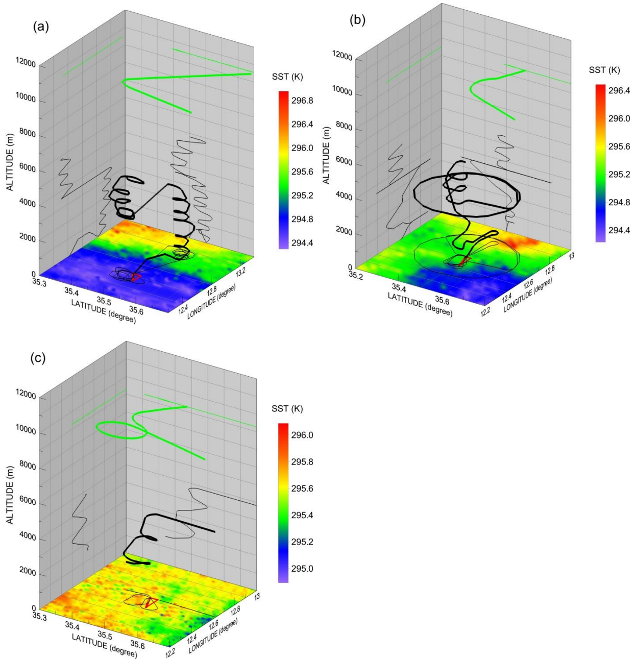
Figure 5: ATR-42 (black curve) and Falcon 20 (green curve) flight paths on (a) 22 June, (b) 28 June, and (c) 3 July, and projections on horizontal and vertical planes. The surface map of the SST from MODIS is shown with the colour scale. A schematic map of Lampedusa contour is shown in red. Please, note that the latitude-longitude and the SST scales are different in each graph.
