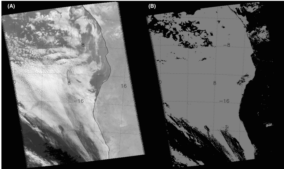
Figure 1. AIRS version 5 visible channel 4 radiance ( 0.49\text{--}0.94\ \mu\text{m} ) at a nadir spatial resolution of 2.28 km (left), and AIRS cloud mask (binary clear and cloudy) determined from visible channel thresholds (right). See Gautier et al. [2003] for more details.
