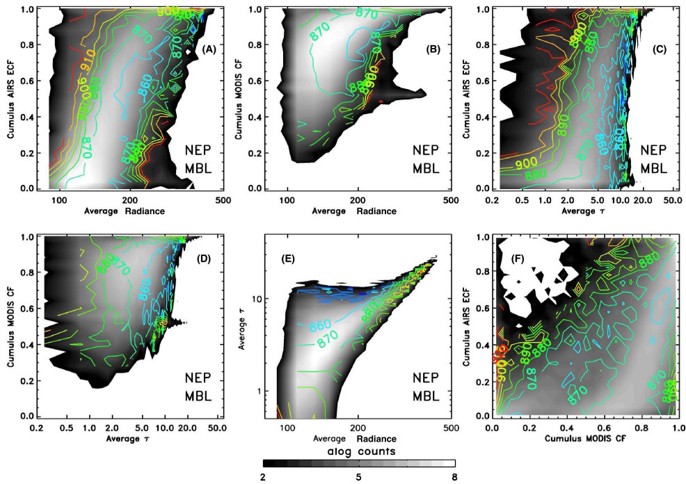
Figure 7. Shown are joint pdfs for six different combinations of variables that are described in Section 4.2: (a) radiance versus AIRS ECF, (b) radiance versus MODIS CF, (c) MODIS \tau versus AIRS ECF, (d) MODIS \tau versus MODIS CF, (e) radiance versus MODIS \tau , and (f) MODIS CF versus AIRS ECF. The grey scale is the natural log of total counts per bin. All values in the pdfs shown are for the cumulus regime. The color contours depict the MBL depth (hPa).
