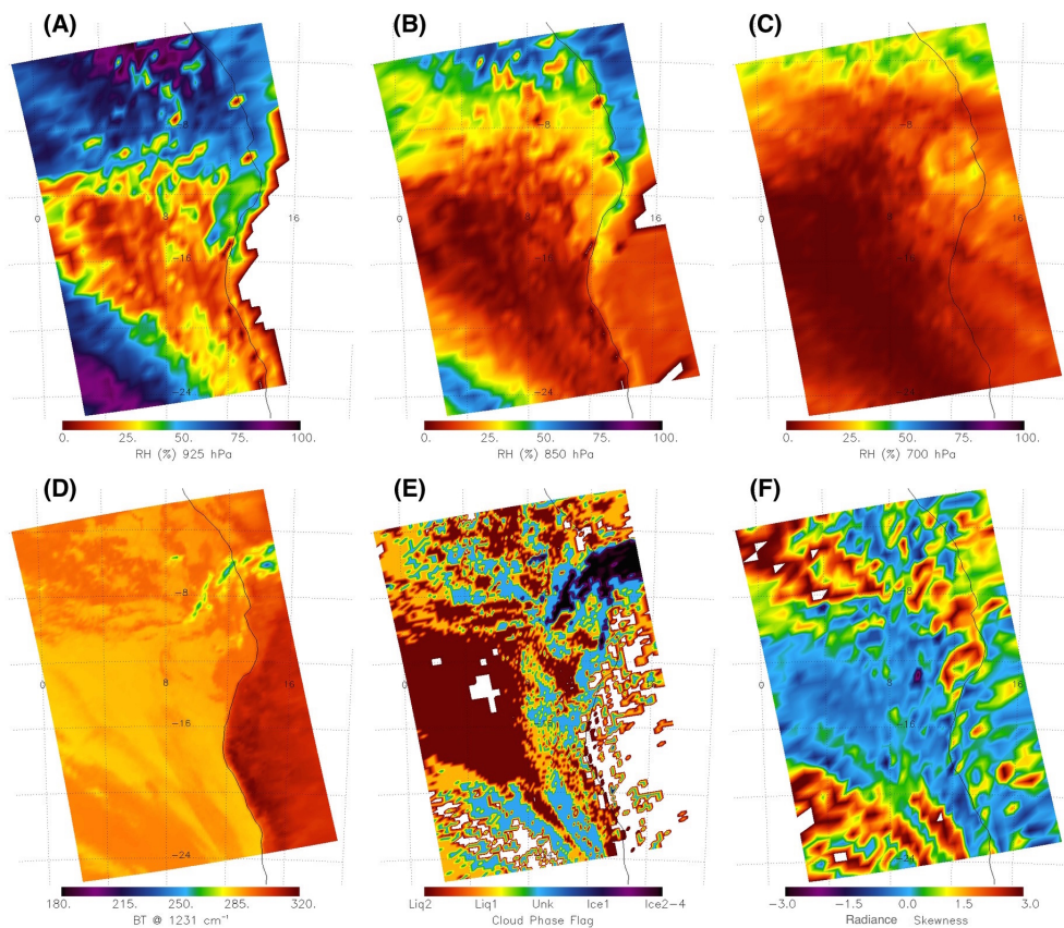
Figure 2. AIRS (a) RH_{925} (%), (b) RH_{850} (%), (c) RH_{700} (%), (d) 1231\text{ cm}^{-1} T_b (K), (e) cloud thermodynamic phase, and (f) radiance skewness from visible channel 4. The granule is identical to the one shown in Fig. 1.
