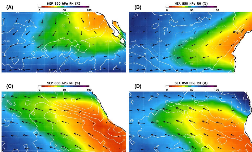
Figure 6. AIRS RH 850 (%) for regions listed in Table 1: (a) NEP, (b) NEA, (c) SEP, and (d) SEA. The MERRA-AIRS RH 850 difference is shown as white contours (solid implies MERRA is moister, and dashed implies AIRS is moister). The length and direction of the arrows depict the 850 hPa wind vectors from MERRA.
