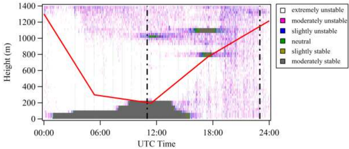
Figure 2. Vertically and temporally resolved atmospheric stability on May 12, 2013 at SGP. The atmospheric stability is classified into extremely unstable (white), moderately unstable (magenta), slightly unstable (blue), neutral (green), slightly stable (brown) and moderately stable (grey) regimes based on Richardson number. The two vertical dash lines represent 06:00 and 18:00 local time, respectively. The red line shows the boundary layer height determined from radiosonde data.
