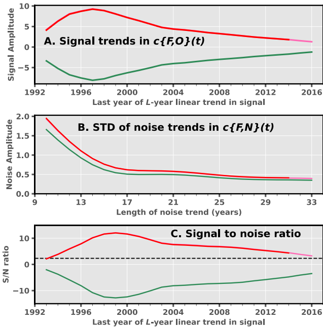
Figure 7: Results from the S/N analysis of simulated and observed changes in zonal-mean upper and lower stratospheric ozone. Signal time-series provide information on the similarity between the time-invariant ODSonly/GHGonly/ALL1 fingerprint pattern and the time-varying observed patterns of stratospheric ozone change. Signal detection relies on both simple linear regression (A-C; “method 1”) and regression between c\{F,O\}(t) and the leading PC of the ODSonly, GHGonly, or ALL1 simulation (D-F; “method 2”). Results are a function of the analysis period L (in years). The L -year trends in the method 1 and method 2 signal time series are plotted in the top row. The year on the abscissa is the end year of the L -length trend beginning in 1984. Noise time series indicate the level of similarity between the searched-for ODSonly, GHGonly, and ALL1 fingerprints and the concatenated CTL, NAT-h, and NAT estimates of natural variability of ozone. The middle panels show the standard deviation of the distribution of maximally overlapping L -year trends in c\{F,N\}(t) . The S/N ratio is shown in the bottom panels. The dashed horizontal line indicates the stipulated significance level of 1% for signal detection.
