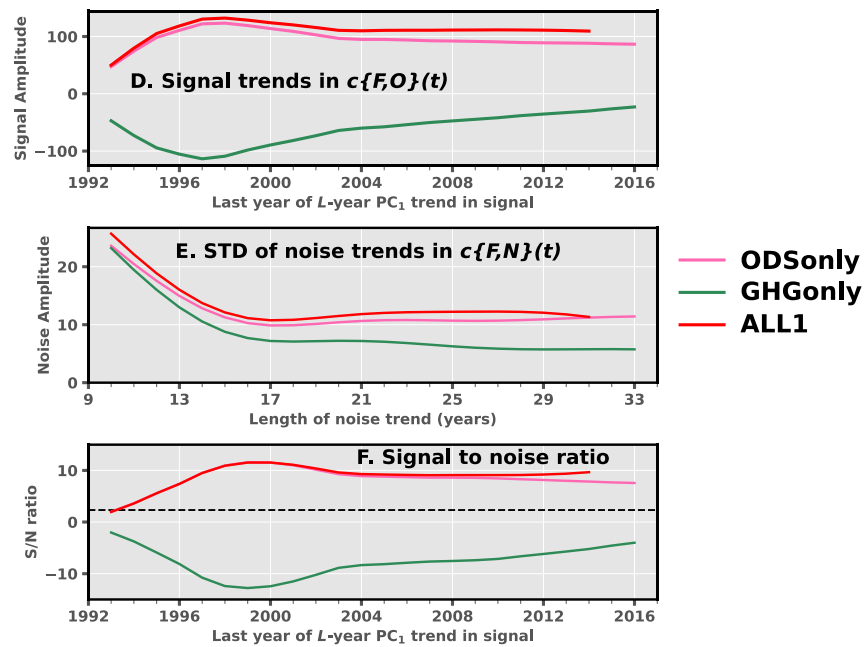
Figure 7: Results from the S/N analysis of simulated and observed changes in zonal-mean upper and lower stratospheric ozone. Signal time-series provide information on the similarity between the time-invariant ODSonly/GHGonly/ALL1 fingerprint pattern and the time-varying observed patterns of stratospheric ozone change. Signal detection relies on both simple linear regression (A-C; “method 1”) and regression between c\{F,O\}(t) and the leading PC of the ODSonly, GHGonly, or ALL1 simulation (D-F; “method 2”). Results are a function of the analysis period L (in years). The L -year trends in the method 1 and method 2 signal time series are plotted in the top row. The year on the abscissa is the end year of the L -length trend beginning in 1984. Noise time series indicate the level of similarity between the searched-for ODSonly, GHGonly, and ALL1 fingerprints and the concatenated CTL, NAT-h, and NAT estimates of natural variability of ozone. The middle panels show the standard deviation of the distribution of maximally overlapping L -year trends in c\{F,N\}(t) . The S/N ratio is shown in the bottom panels. The dashed horizontal line indicates the stipulated significance level of 1% for signal detection.
