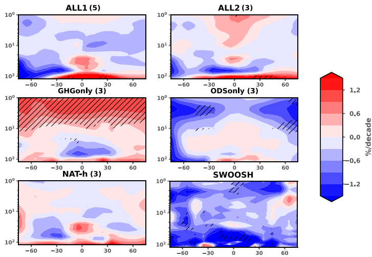
Figure 4: Zonal-mean stratospheric ozone trends estimated using A) linear regression and B) EESC regression of annual-mean anomalies from 1984-2016. For model simulations, trend estimates use the ensemble mean. Hatching indicates significance at the 5% level or better using a two-sided Student's t-test. Figures in brackets indicate the number of ensemble members. All of the trends shown are for 1984-2016, except for ALL1 which is from 1984-2014.
