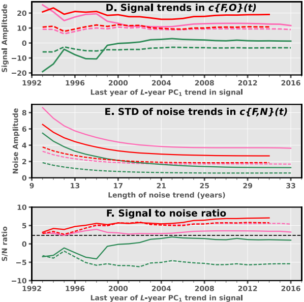
Figure 8: Same as Fig. 7 but for the lower stratosphere. The solid line shows results for the global lower stratosphere, while the dashed lines exclude the tropics (30°S to 30°N).
