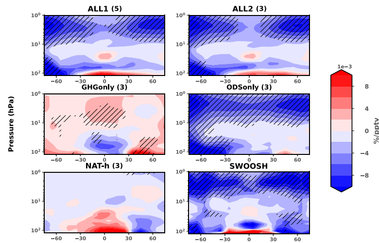
Figure 4: Zonal-mean stratospheric ozone trends estimated using A) linear regression and B) EESC regression of annual-mean anomalies from 1984-2016. For model simulations, trend estimates use the ensemble mean. Hatching indicates significance at the 5% level or better using a two-sided Student's t-test. Figures in brackets indicate the number of ensemble members. All of the trends shown are for 1984-2016, except for ALL1 which is from 1984-2014.
