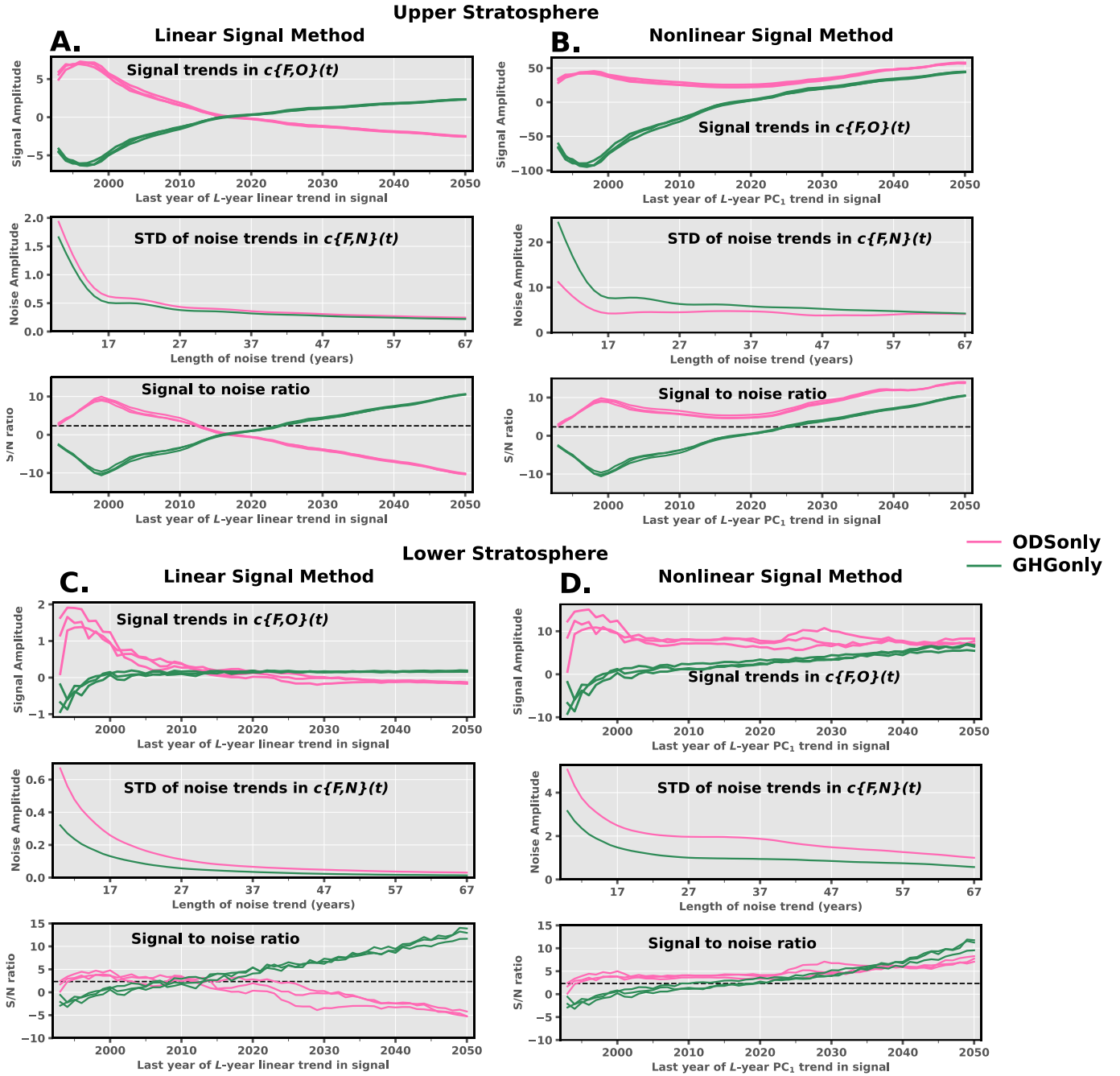
Figure 10: Same as in Figs. 7 and 8 but the ALL2 ensemble members (3 total) are used as surrogate observations, yielding information regarding the estimated detection time for the ODSonly and GHGonly fingerprints in model data. The \beta_l and \beta_{PC_1} results in A) and B) are for the upper stratosphere (respectively); results in C) and D) are the corresponding method 1 and method 2 for the lower stratosphere.
