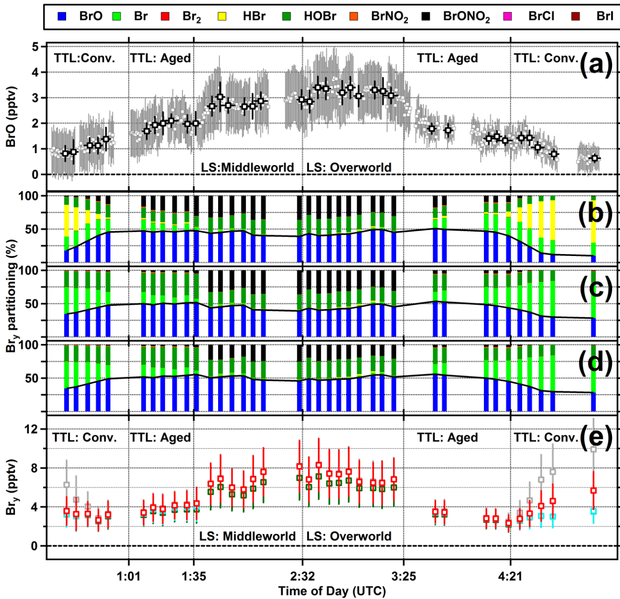
5 Figure 4: BrO, Br y , and Br y partitioning during the RF15 jet crossing flight. (a) (black) 5 min average BrO used for model input; (grey) 30 s data. (b-d) Partitioning of Br y species from box model for (b) case 0, (c) case 2, (d) case 3; (black line) BrO/Br y ratio. (e) Br y inferred along the flight track using the measured BrO and the modeled ratio; (grey) case 0; (red) case 1; (cyan) case 2; (dark green) case 3.
