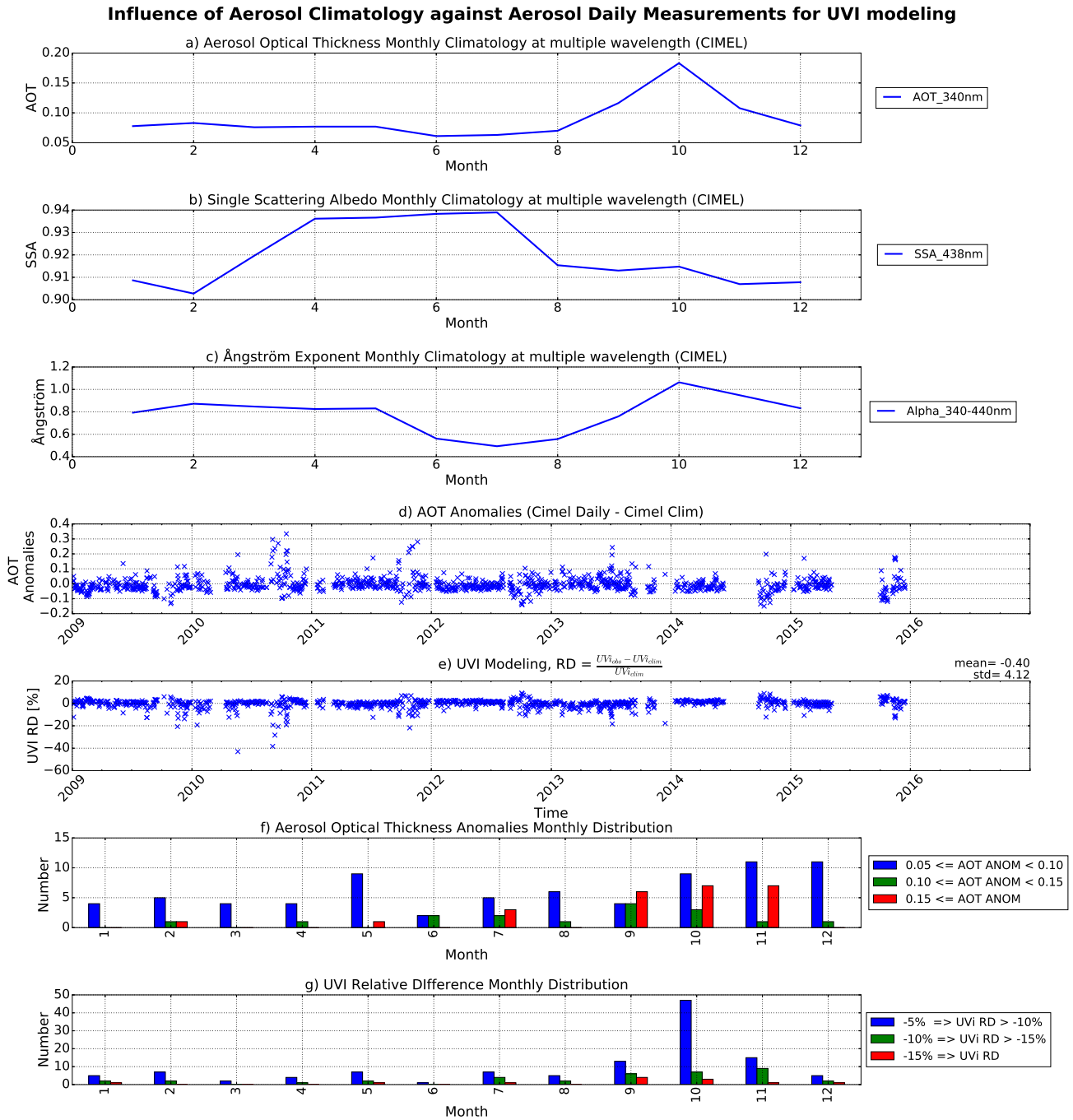
Figure 7. Impact of aerosols on UVI modelling.
