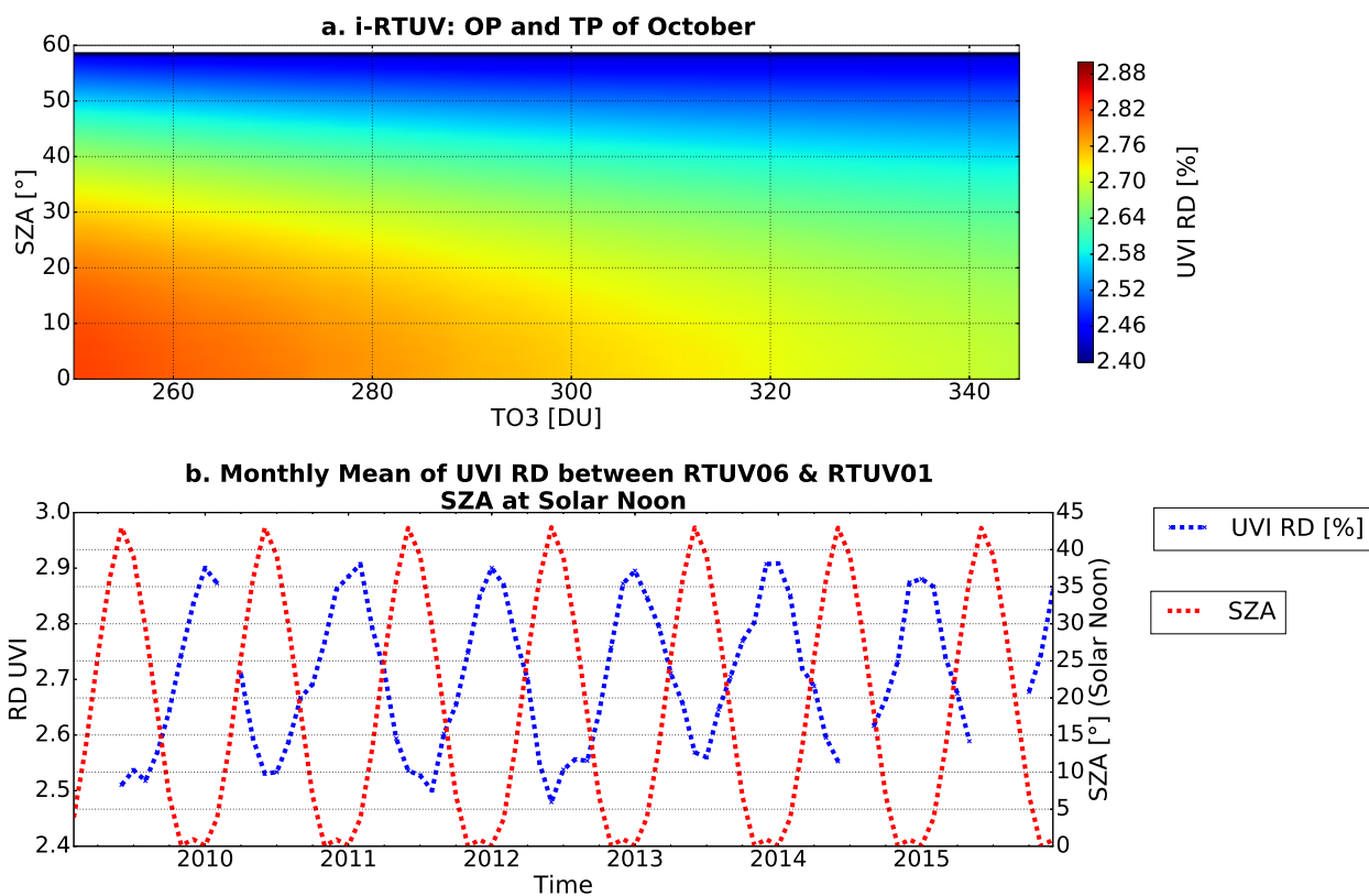
Figure 5. a) UVI Relative Difference between two idealized runs with different O3XS for a varying TO3 and SZA and for climatological OP and TP of October. b) Monthly Mean of UVI RD between RTUV06 and RTUV01 (blue dashed line). Monthly Mean of SZA at Solar Noon. (red dashed line)
