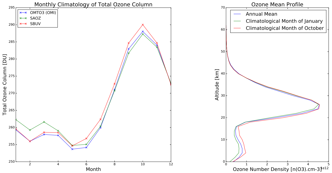
Figure 3. Ozone Variability over Reunion Island. Left : Monthly Climatology of Total Ozone Column for three datasets (OMI in blue, SAOZ in green and SBUV in red) Right: Mean Ozone Profile from McPeters and Labow [2012] Climatology. Annual mean in blue, January in green and October in red.
