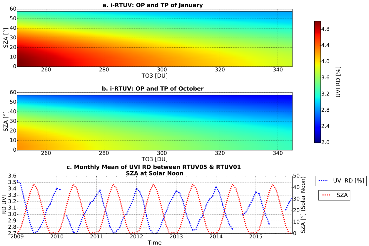
Figure 4. a) UVI Relative Difference between two idealized runs with different ET spectra for a varying TO3 and SZA for a climatological OP and TP of January b) Same as a) but for OP and TP of October. c) Monthly Mean of UVI RD between RTUV05 and RTUV01 (blue dashed line). Monthly Mean of SZA at Solar Noon. (red dashed line)
