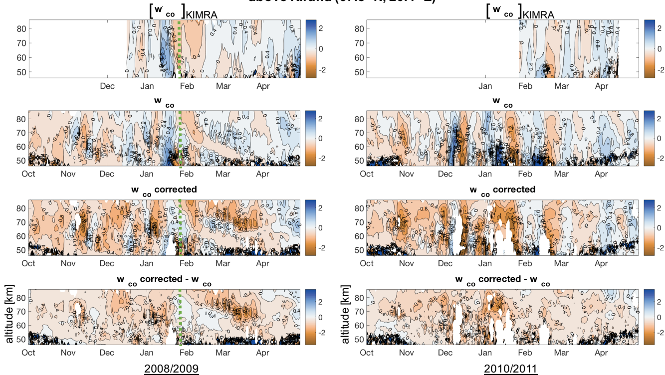
5 Figure 6: Rates of vertical motion, in km/day, calculated by tracking CO VMRs over time. w_{CO} is calculated using daily averaged SD-WACCM CO profiles. w_{CO} corrected is calculated using a combination of SD-WACCM CO profiles and TEM tendencies (see Sect. 4 for details). The difference between the two rates of descent is also shown. The results plotted are for above Kiruna for the winters of 2008/2009 and 2010/2011. Contour lines are spaced by 0.2 km/day. Areas with tightly packed contours (black areas) occur when there are very low CO VMRs and the calculation method is unreliable. White areas are where a CO VMR could not be tracked within the shown altitude range. The start date of the SSW on January 28 th 2009, is shown with a vertical green dashed line. Rates calculated using KIMRA CO data are also included in the upper panel, titled [w_{CO}]_{KIMRA} .
