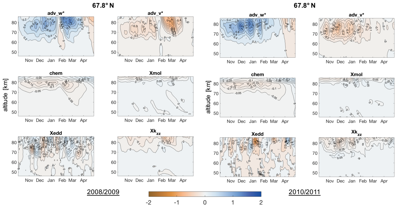
5 Figure 3: 11-day running mean tendencies of CO (in ppmv/day), calculated using daily averaged SD-WACCM output. Tendencies shown are for 67.8° N for the winters of 2008/2009 and 2010/2011. See section 3.1 for a description of the tendencies, which are represented in the TEM continuity equation. Note that the labelled contours may be differently spaced in each panel, to match the range of values for individual tendencies.
