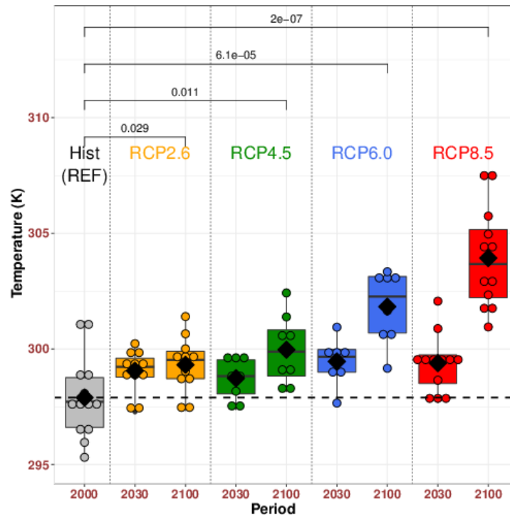
Figure R2.1 Box-whisker plots of the annual average of temperature in kelvin (K) since 2000, calculated over the Mediterranean Basin domain for the JJA period and for the RCP2.6 (yellow), RCP4.5 (green), RCP6.0 (blue) and RCP8.5 (red). The median is indicated by the thick horizontal black line, the multi-model mean by a filled diamond, the (25-75%) range by the colored box and minimum/maximum excluding outliers by whisker. Each filled circle represents a single model. The p-value of the student T test at the 95% confidence level is indicated for each RCP trend between 2000 and 2100 at the top of the figure. This means that if the p-value between two groups is less than 0.05, the trend is significant.
