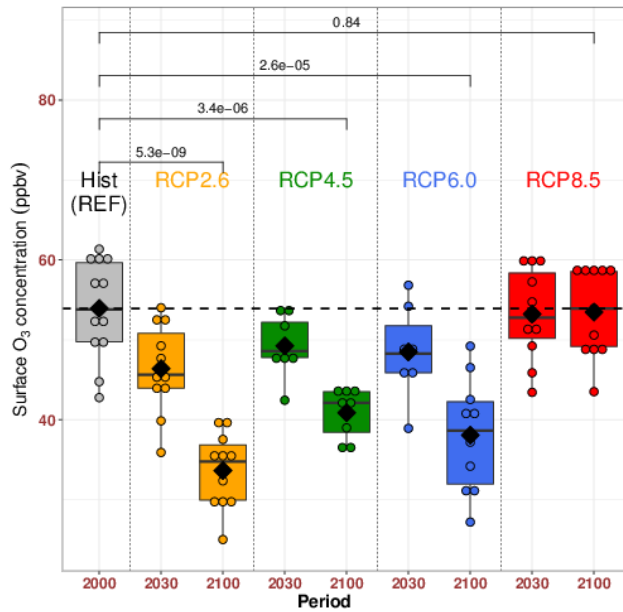
Figure R2.2: legend Box-whisker plots of the annual average of surface ozone in ppbv since 2000, calculated over the Mediterranean Basin domain for the JJA period and for the RCP2.6 (yellow), RCP4.5 (green), RCP6.0 (blue) and RCP8.5 (red). The median is indicated by the thick horizontal black line, the multi-model mean by a filled diamond, the (25-75%) range by the colored box and minimum/maximum excluding outliers by whisker. Each filled circle represents a single model. The p-value of the student T test at the 95% confidence level is indicated for each RCP trend between 2000 and 2100 at the top of the figure. This means that if the p-value between two groups is less than 0.05, the trend is significant.
