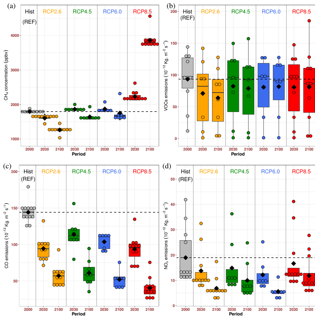
Figure 7. Same as Fig. 6 but for the surface CH 4 concentrations (a) and emissions of ozone precursors: VOCs (b), CO (c) and NO x (d).
