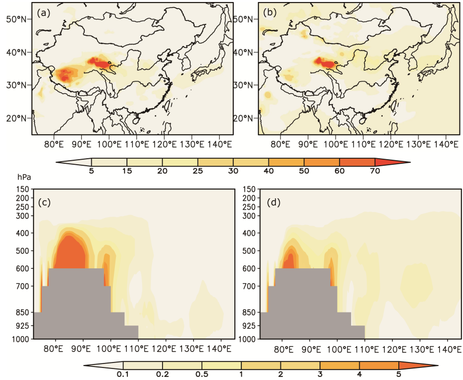
5 Figure 8: (a, b) Simulated differences (CON minus SEN) in the horizontal distribution of the column dust load ( \text{mg m}^{-2} ) and (c, d) the longitude–height cross-section (averaged over 32–36°N) of the dust mixing ratio ( \mu\text{g kg}^{-1} ) for summer in heavy (left) and light dust years (right).
