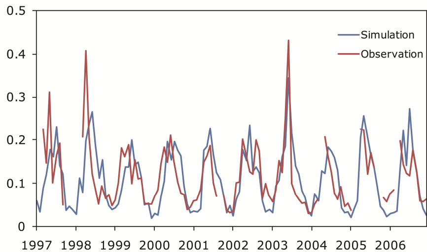
Figure 4: Comparison between the simulated variation of the monthly mean dust AOD in the control experiment and the AERONET-observed variation of the monthly mean aerosol AOD (500 nm) at Dalanzadgad from 1997 to 2006 ( r=0.66 ).
