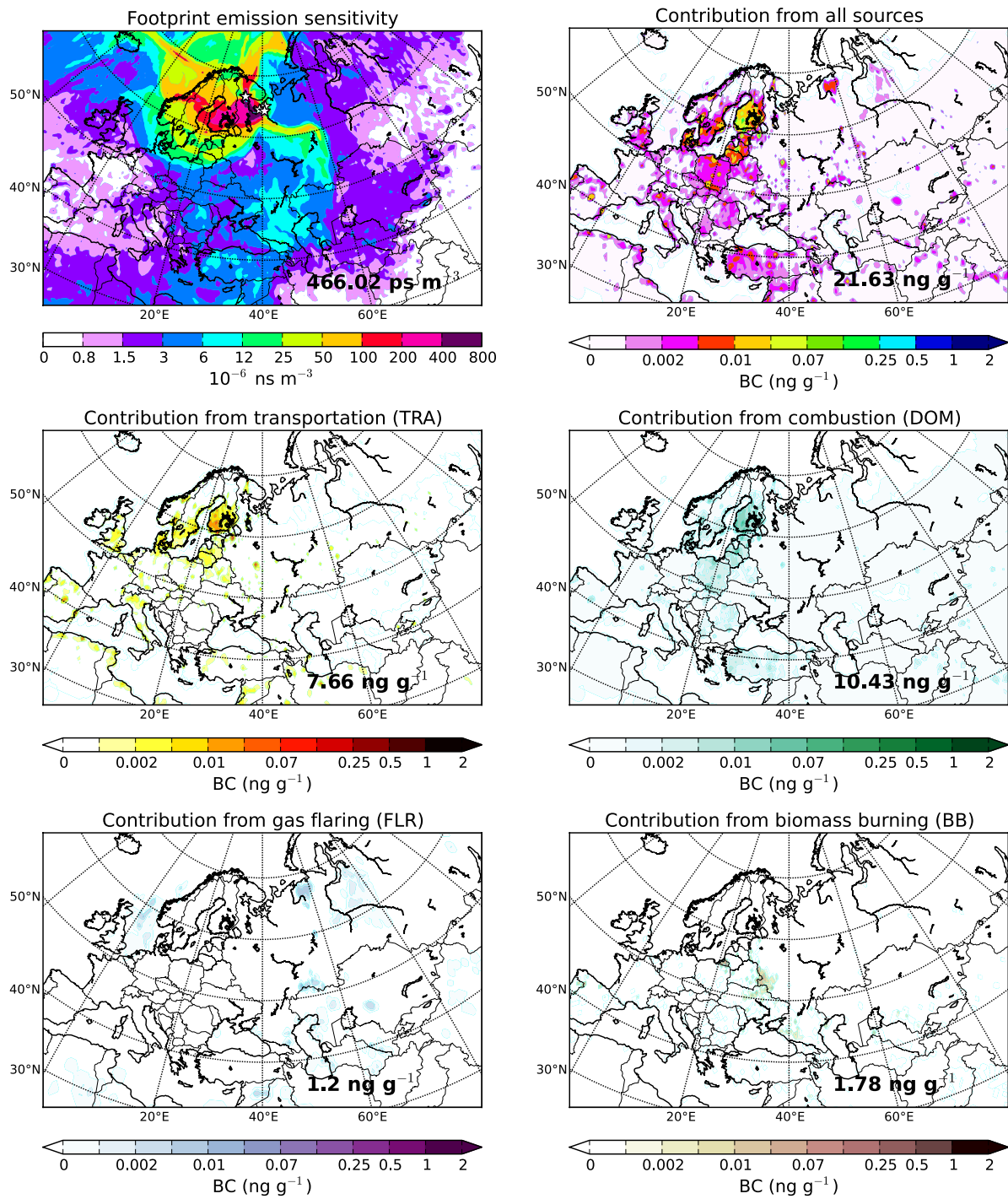
Figure S 4. Average footprint emission sensitivity and source contribution (from all sources, TRA, DOM, FLR and BB) for all the samples located in northwestern European Russia.
