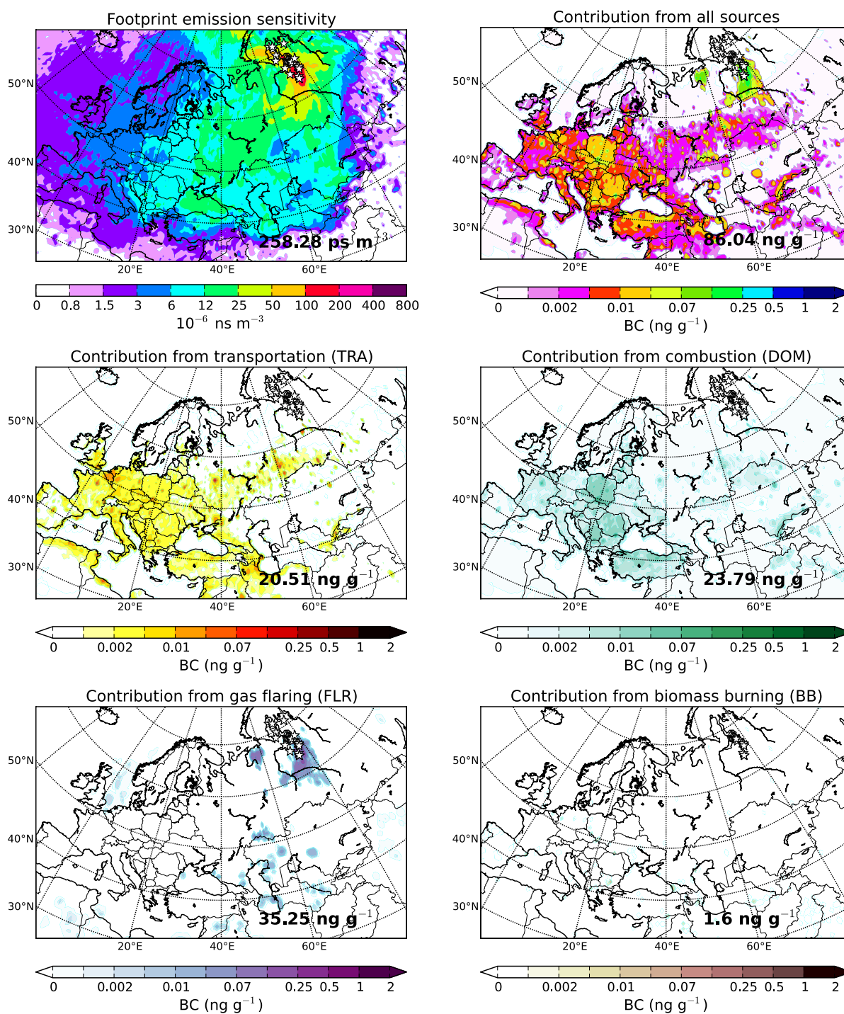
Figure S 5. Average footprint emission sensitivity and source contribution (from all sources, TRA, DOM, FLR and BB) for all the samples located in Western Siberia (north of 62 °N).
