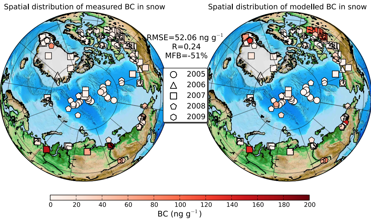
Figure S 2. Distribution of snow measurements of BC adopted from Doherty et al. (2010) in the Arctic from 2005 to 2009 (left). Simulated (FLEXPART) BC concentrations in snow for the same period (right). MFB, RMSE and correlation coefficient (R) values are further given.
