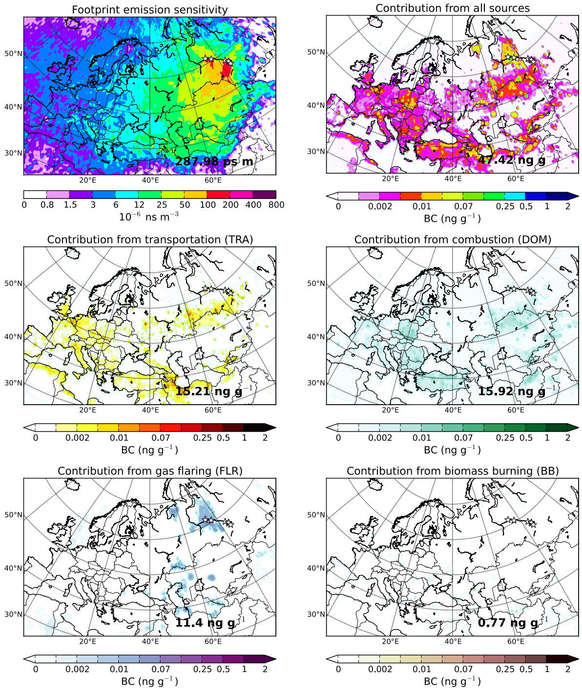
Figure S 6. Average footprint emission sensitivity and source contribution (from all sources, TRA, DOM, FLR and BB) for all the samples located in Western Siberia (south of 62 °N).
