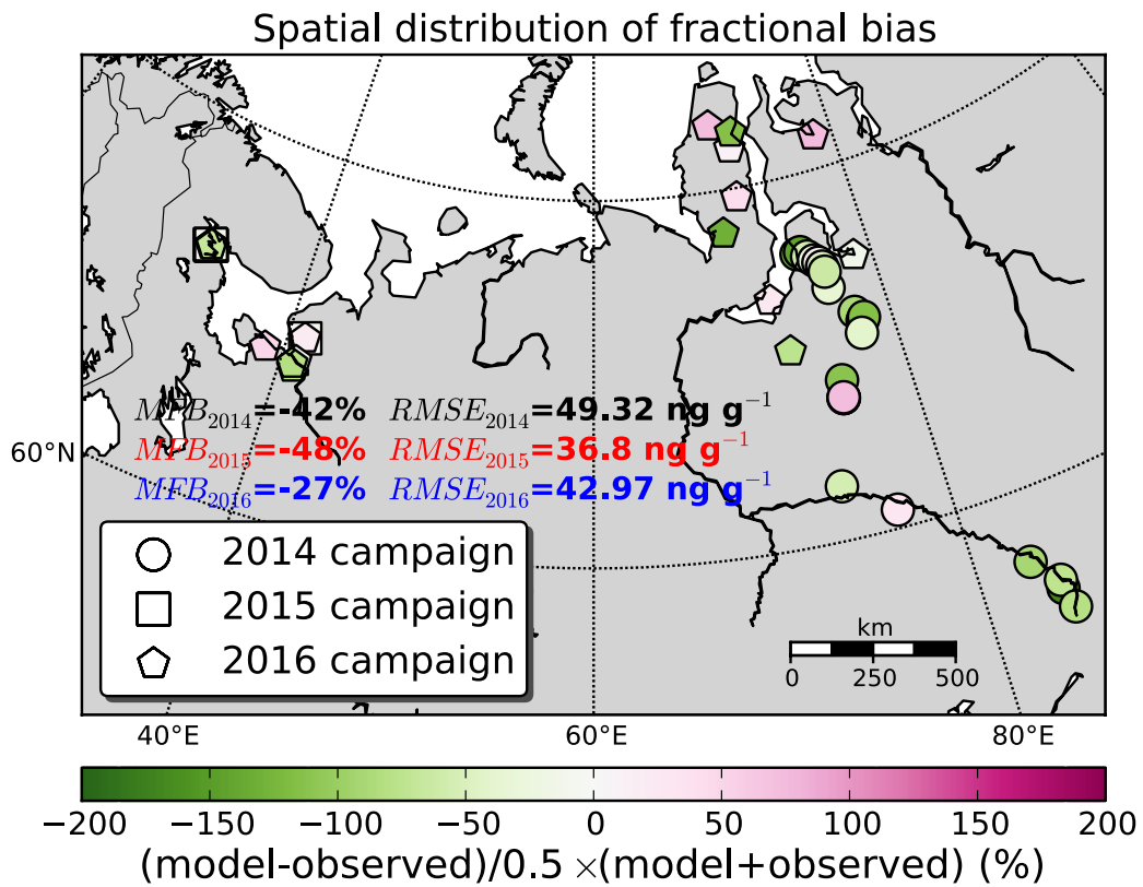
Figure S 1. Fractional bias ( FB = [(C_m - C_o)/(C_m + C_o) \times 0.5] \times 100\% ) for all samples collected from the three campaigns in Western Siberia and northwestern European Russia in 2014, 2015 and 2016. MFB (mean fractional bias) is the fractional bias averaged for all snow samples from 2014, 2015 and 2016, whereas RMSE is the root mean square error in \text{ng g}^{-1} ).
