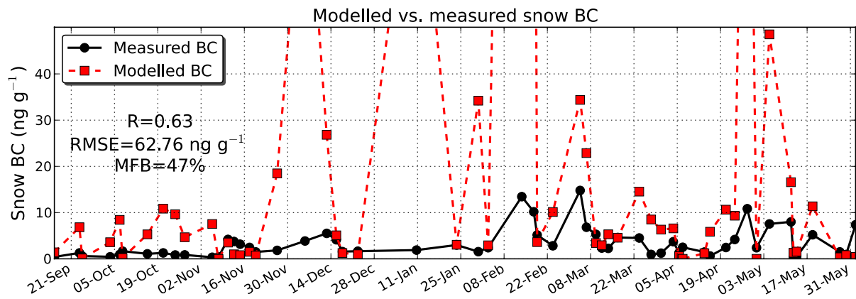
Figure S 3. Timeseries of simulated and measured BC concentrations in snow collected in Alert (Macdonald et al., 2016). Correlation coefficient (R) between modelled and measured BC, RMSE and MFB values are also shown.
