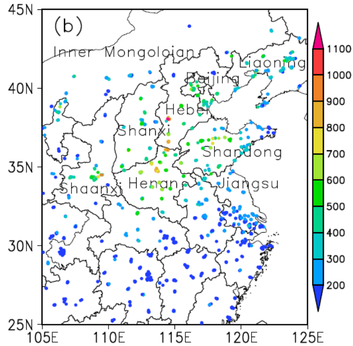
350 Figure 4 (a) the measures to limit anthropogenic emissions and (b) the maximum hourly PM_{2.5} concentration during the period of 16–21 December 2016. In panel (a), the red rectangle indicates both the vehicle control and production restriction measures that were implemented, while the blue triangle indicates the production that was restricted. The letters in panel (b) were the names of the provinces.
