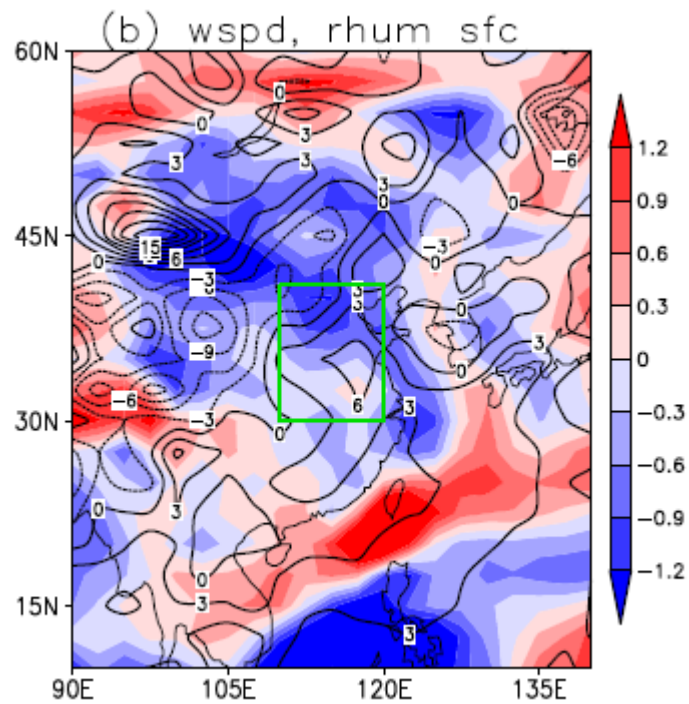
Figure 3 Distribution of the regional atmospheric circulation anomalies, (a) the height of PBL (shading), surface lift index ( contour ) and wind at 850 hPa (arrow); and (b) the surface wind speed (shading) and surface relative humidity (contour) in December 2016. The anomalies here are calculated with respect to the period from 1981–2010. —
