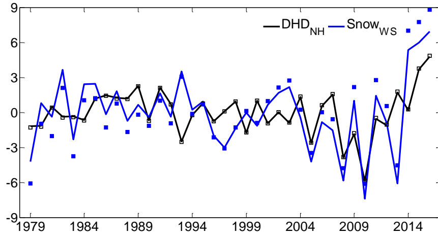
Figure 13 Variation of the DHD NH (black) and Snow WS (blue) indices from 1979 to 2016. The solid lines indicate the indices whose linear trends were removed, and the symbols without lines are the original indices.
