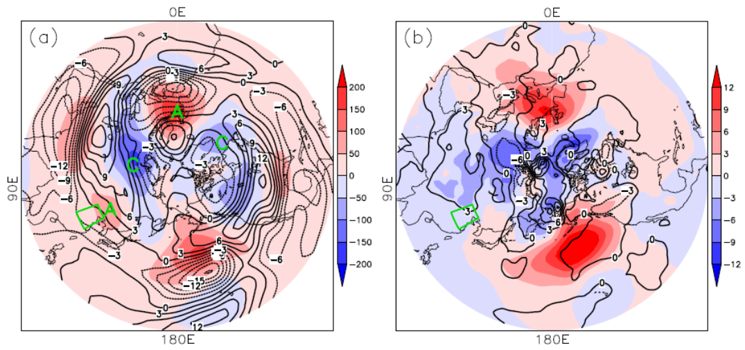
335 Figure 2 Distribution of the global atmospheric circulation anomalies, (a) Z500 (shading) and U200 (contour) and (b) SLP (shading) and SAT (contour) in December 2016. The anomalies here are calculated with respect to the period from 1981–2010.
