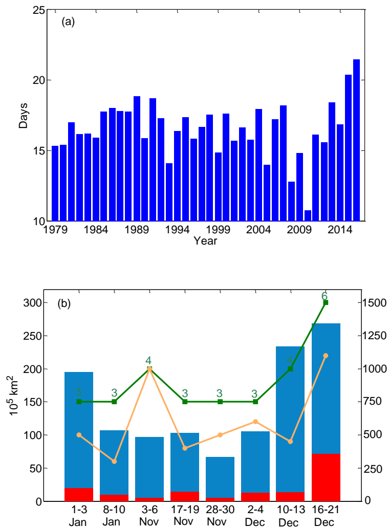
330 Figure 1 (a) The variation of DHD_{NH} from 1979 to 2016 and (b) the parameters of the main haze processes in China in 2016: haze (blue bar) and severe haze (red bar) cover area, the maximum PM_{2.5} concentration (yellow line, right y-axis, unit: \mu g/m^3 ) and the number of lasting days (green line and number).
