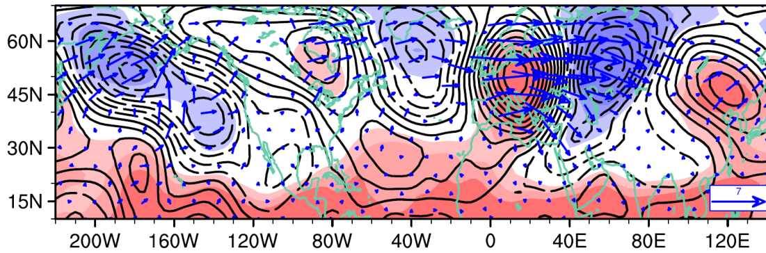
Figure 10 (a) The correlation coefficients (shading) between the preceding autumn SST and DHD_{NH} , and the anomalous SST in 2016 (contour) that are calculated with respect to the period from 1979–2016; and (b) The correlation coefficients between SST_{EP} and Z500 exceeding the 90% confidence level (shading), correlated WAF (arrow) and quasi-geostrophic stream function (contour) at 500 hPa in December.
