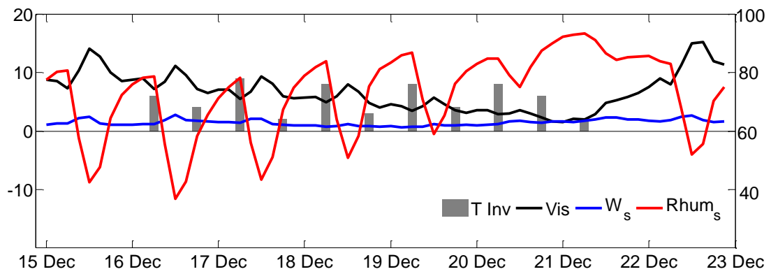
355 Figure 5 The variation of area-mean visibility (black), surface wind speed (blue) and surface relative humidity (red, right y-axis). The intensity of the temperature inversion ( T_{925}-T_{1000} ) in Beijing is shown as gray bar.
