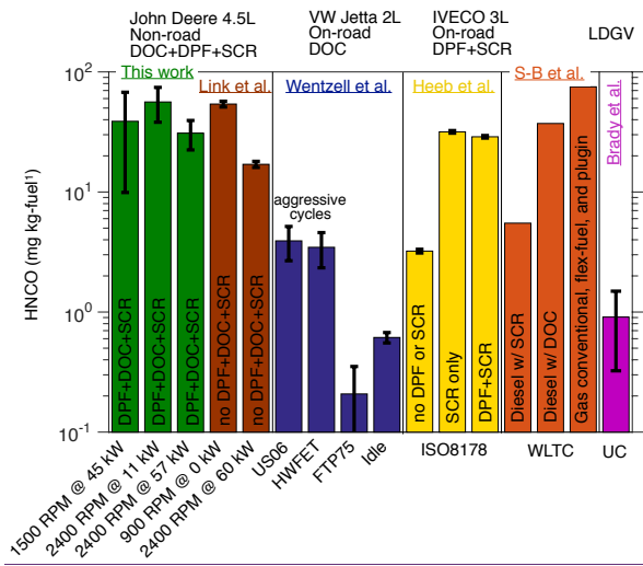
Figure 3: Emission factors for HCNCO from this work compared to literature data. US06, HWFET, FTP75, ISO8178, WLTC and UC are vehicle/engine drive cycles. S-B refers to the Suarez-Bertoa and Astorga (2016).
