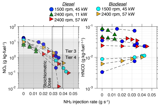
Figure 2: Emission factors for (a) NO x (NO+NO 2 ) and (b) HNCO with varying NH 3 injection rates for all the experiments performed in this work. The NH 3 injection rates are calculated assuming each urea molecule produces two NH 3 molecules.
