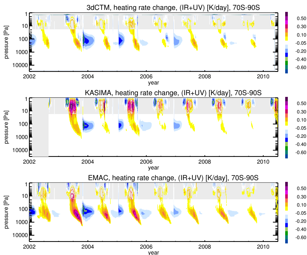
Figure 10. Changes in daily net radiative (short-wave and long-wave) heating rates (K/day) due to particle-induced ozone changes derived from all three models (top: 3dCTM, middle: KASIMA, bottom: EMAC) at high Southern latitudes (70–90°S).
