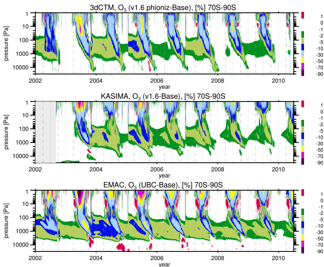
Figure 8. Relative Ozone anomalies due to energetic particle precipitation at high Southern latitudes (70–90°S), calculated as the difference of model runs with to without particle impact (%). Top: 3dCTM (v1.6 phioniz-Base), middle: KASIMA (v1.6 - Base), third: EMAC (UBC - Base). The gray shaded area in the middle figure denotes the time-period before the start of the KASIMA model runs. Dashed and dotted vertical gray lines mark zero, one-quarter, one-half, and three-quarters of each year.
