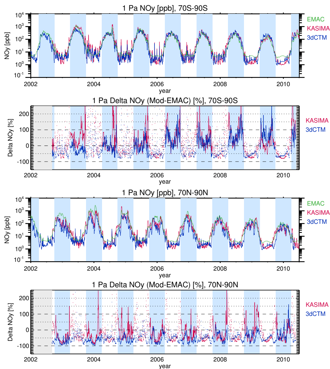
Figure 2. Temporal evolution of the volume mixing ratio of NO y (ppb) from all three models at high Southern and Northern latitudes (70–90°S/N), at 1 Pa. Also shown are relative differences from KASIMA and 3dCTM to EMAC results (%). Light blue shading denotes winter in the Southern/Northern hemisphere (second and third quarter of each year / first and fourth quarter of each year). The gray shading in the difference plots denote the period at the start where KASIMA results were not yet available. To highlight differences in polar winter, differences in summer are shown as dots, while differences in winter are shown as solid lines. KASIMA: red, 3dCTM: blue, EMAC: green.
