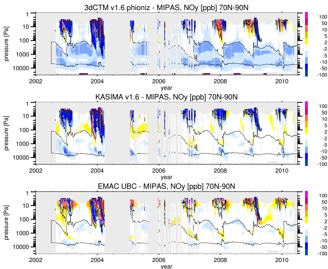
Figure 6. Absolute difference in \text{NO}_y (ppb) between models and MIPAS observations in high Northern ( 70\text{--}90^\circ\text{N} ) latitudes. Model data have been interpolated to the vertical grid of the MIPAS data, and only days and altitudes are shown where MIPAS data are available, and fulfill the averaging kernel criterion. From top to bottom: 3dCTM v1.6 phioniz, KASIMA v1.6, and EMAC UBC. The black lines show the 10, 20, and 3000 ppb contours of the MIPAS data, smoothed with a 7-day running mean for clarity. The gray shaded areas are periods without MIPAS data, in the second panel also the period before the start of the KASIMA model run.
