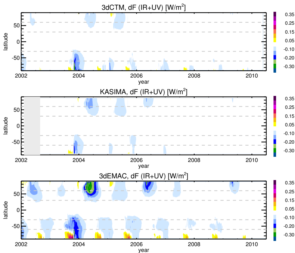
Figure 12. Daily changes in the net amount of energy absorbed or transmitted due to particle induced ozone destruction in the stratosphere ( \text{W/m}^2 ), derived from the difference of model runs with to model runs without particle forcing, as a function of time and latitude.
