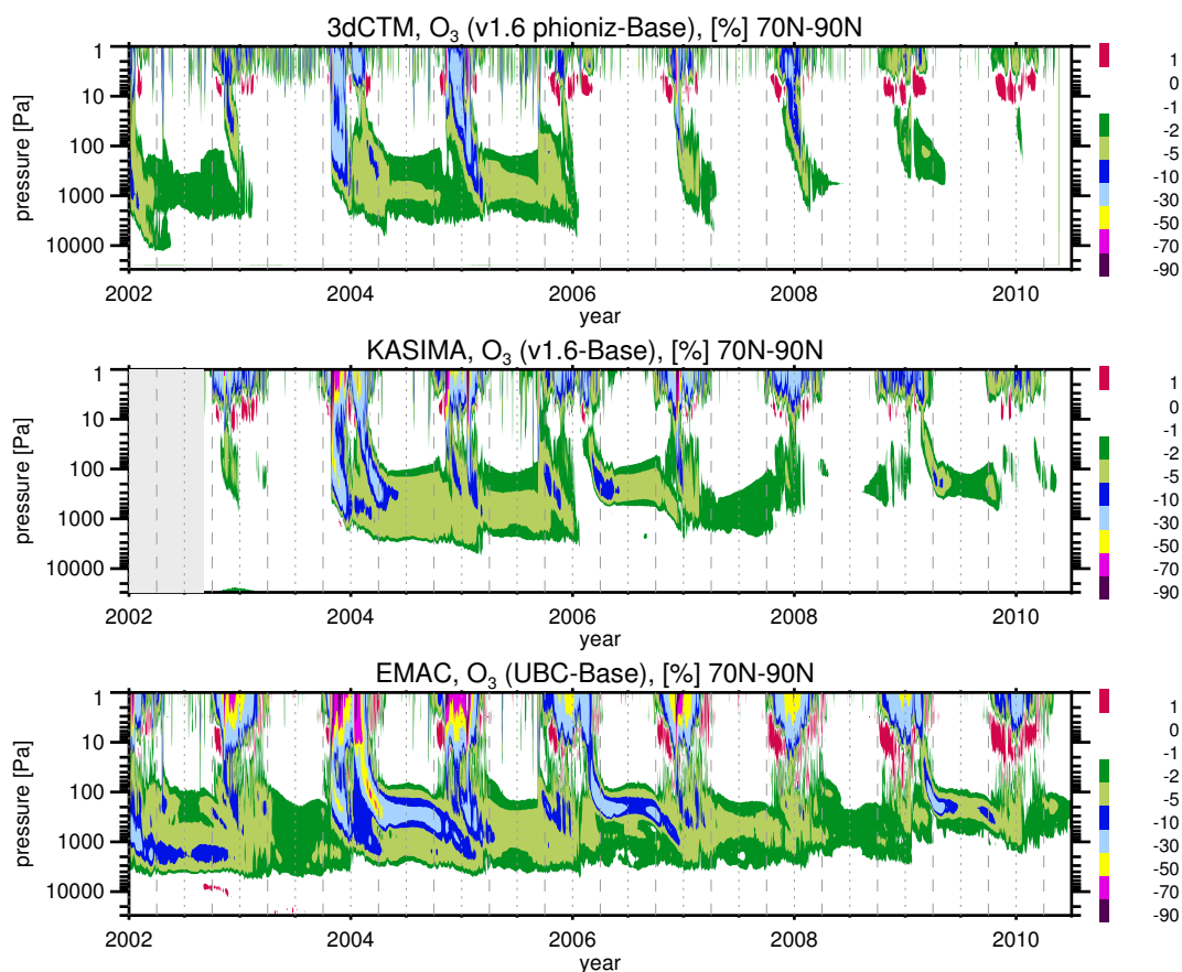
Figure 9. Relative Ozone anomalies due to energetic particle precipitation at high Northern latitudes (70–90°N), calculated as the difference of model runs with to without particle impact (%). Top: 3dCTM (v1.6 phioniz-Base), middle: KASIMA (v1.6 - Base), third: EMAC (UBC - Base). The gray shaded area in the middle figure denotes the time-period before the start of the KASIMA model runs. Dashed and dotted vertical gray lines mark zero, one-quarter, one-half, and three-quarters of each year.
