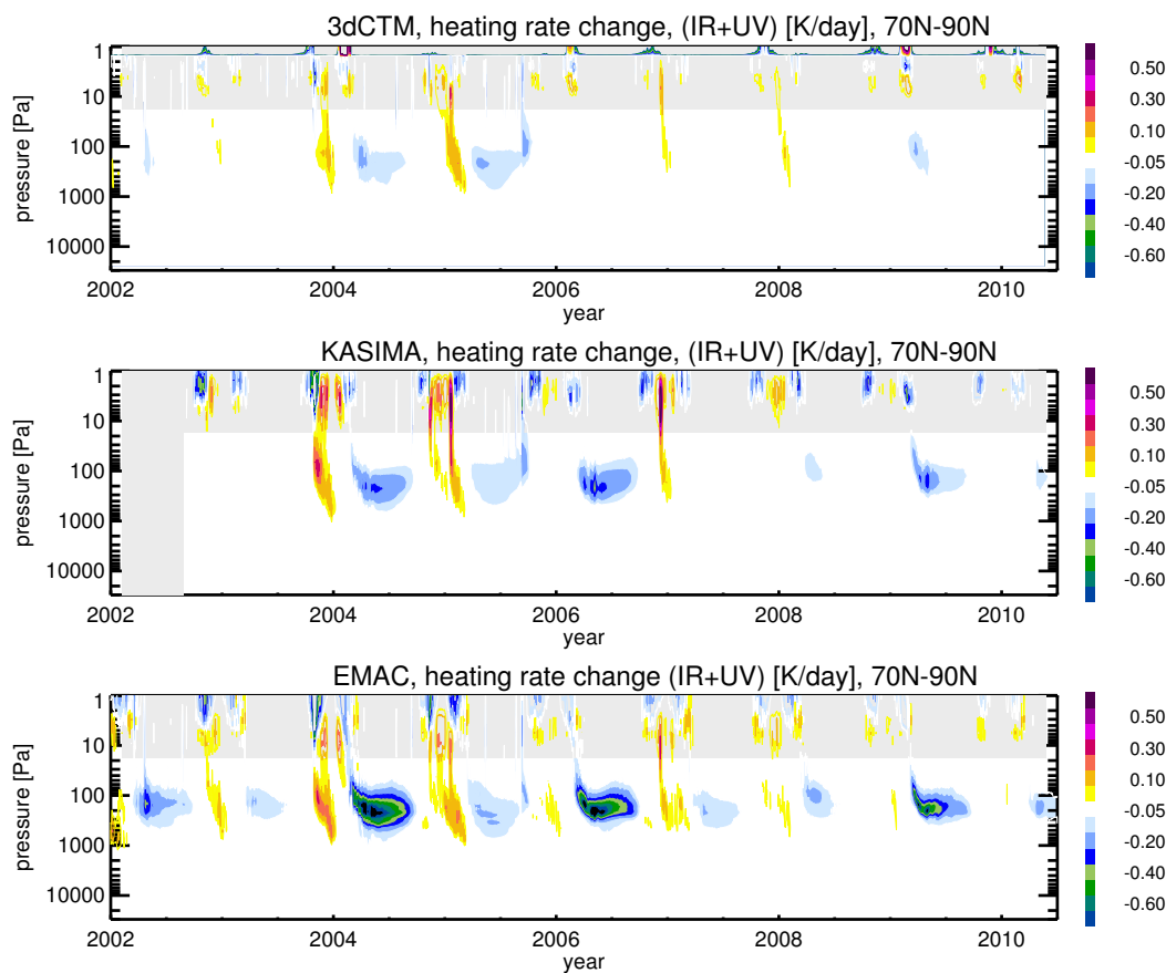
Figure 11. Changes in daily net radiative (short-wave and long-wave) heating rates (K/day) due to particle-induced ozone changes derived from all three models (top: 3dCTM, middle: KASIMA, bottom: EMAC) at high Northern latitudes (70–90° N).
