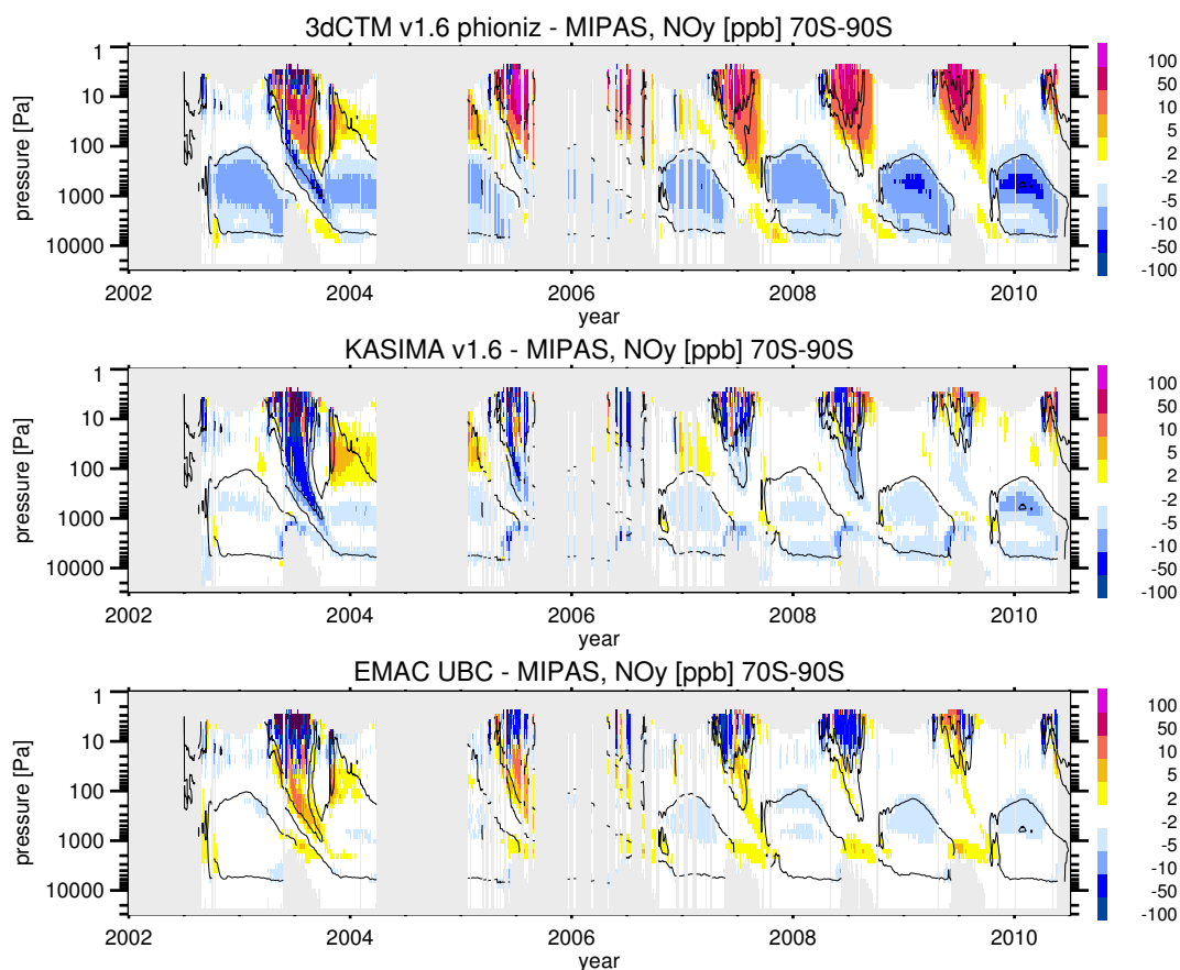
Figure 5. Absolute difference in \text{NO}_y (ppb) between models and MIPAS observations in high Southern (70–90°S) latitudes. Model data have been interpolated to the vertical grid of the MIPAS data, and only days and altitudes are shown where MIPAS data are available, and fulfill the averaging kernel criterion. From top to bottom: 3dCTM v1.6 phioniz, KASIMA v1.6, and EMAC UBC. The black lines show the 10, 20, and 3000 ppb contours of the MIPAS data, smoothed with a 7-day running mean for clarity. The gray shaded areas are periods without MIPAS data, in the second panel also the period before the start of the KASIMA model run.
