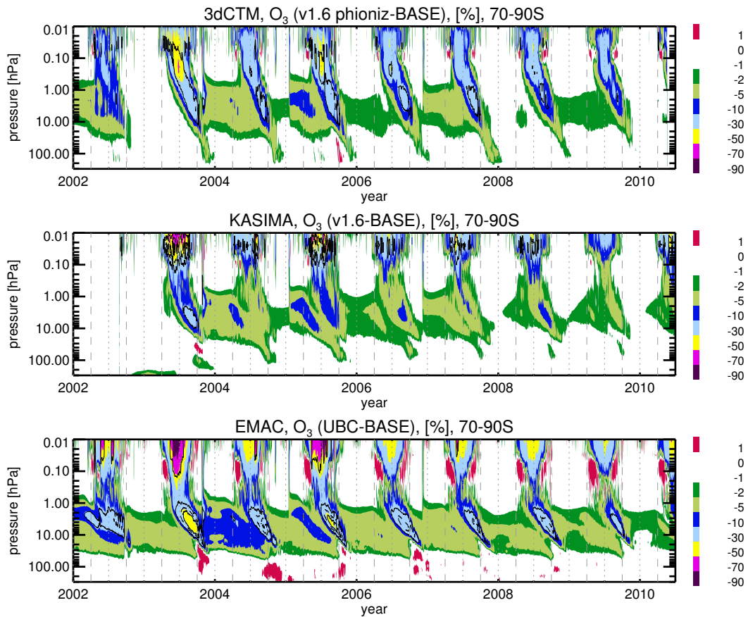
Figure 12. Relative Ozone anomalies due to energetic particle precipitation at high Southern latitudes ( 70\text{--}90^\circ\text{S} ), calculated as the difference of model runs with to without particle impact (%). Top: 3dCTM (v1.6 phioniz-Base), middle: KASIMA (v1.6 - Base), third: EMAC (UBC - Base). The gray shaded area in the middle figure denotes the time-period before the start of the KASIMA model runs. Dashed and dotted vertical gray lines mark zero, one-quarter, one-half, and three-quarters of each year. The thin black contours refer to -1.5 (solid), -1 (dashed) and -0.5 (solid) ppm.
