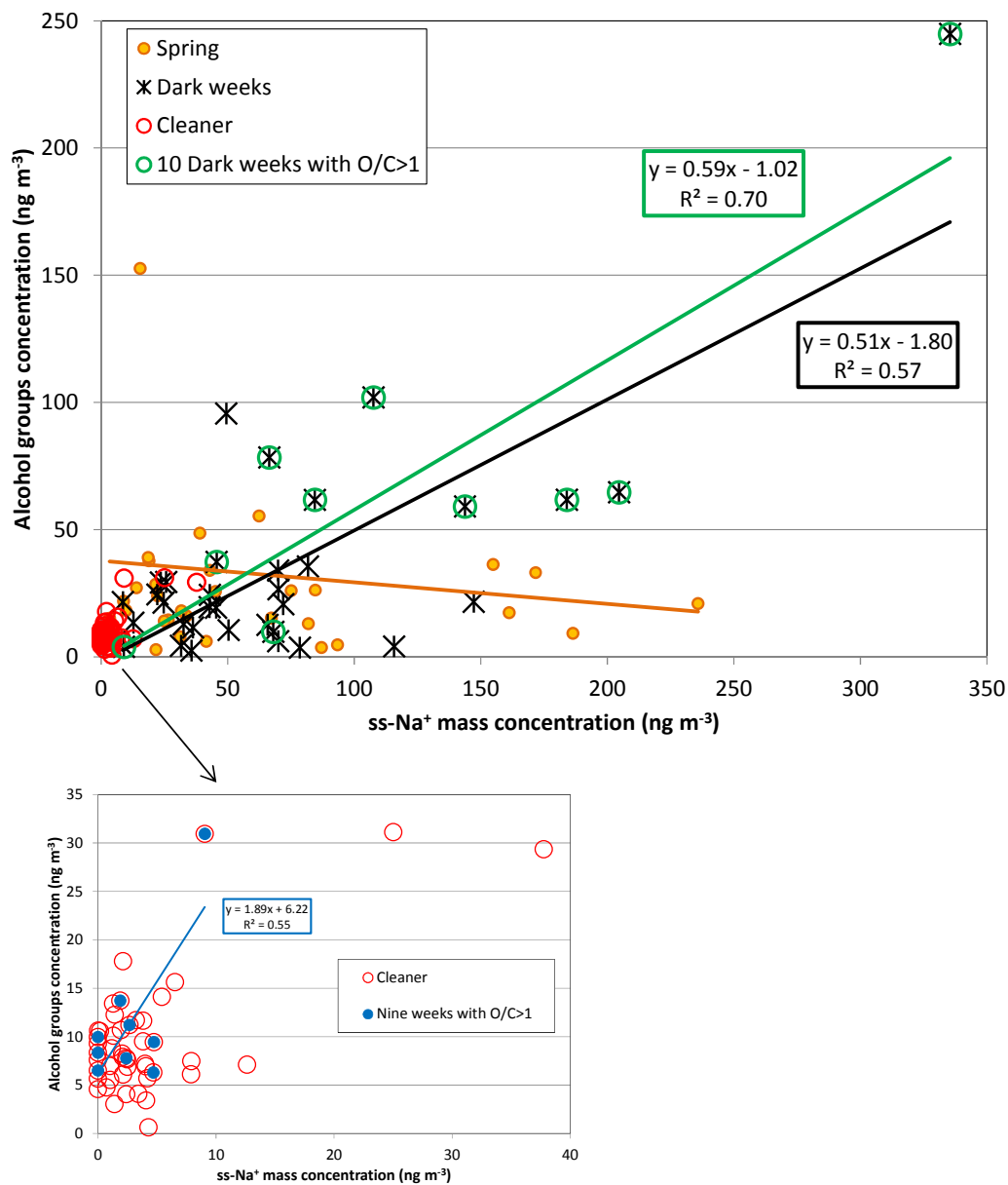
5 Figure 10. Regressions of weekly-averaged mass concentrations of alcohol functional groups with ss-Na^+ for the spring weeks, dark weeks, cleaner weeks and for the 10 dark weeks with O/C > 1 . Results of linear regressions are indicated where significant ( P < 0.05 ). Lower plot expands the cleaner weeks and identifies the nine weeks during July and August of 2013 with O/C > 1 .
