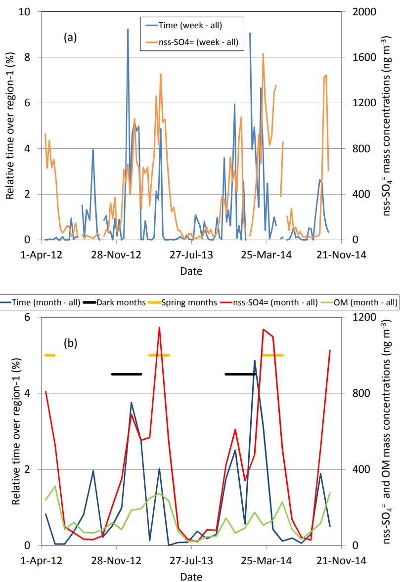
5 Figure 7a and 7b. (a) Time series of percentage time over Region 1 from weekly averages of FLEXPART analysis with weekly-averaged nss-SO 4 - mass concentrations. (b) Time series of time over Region 1 from monthly averages of FLEXPART analysis with monthly-averaged nss-SO 4 - and OM concentrations. The bars in (b) delineate the dark months (NDJF) and spring months (MAM).
