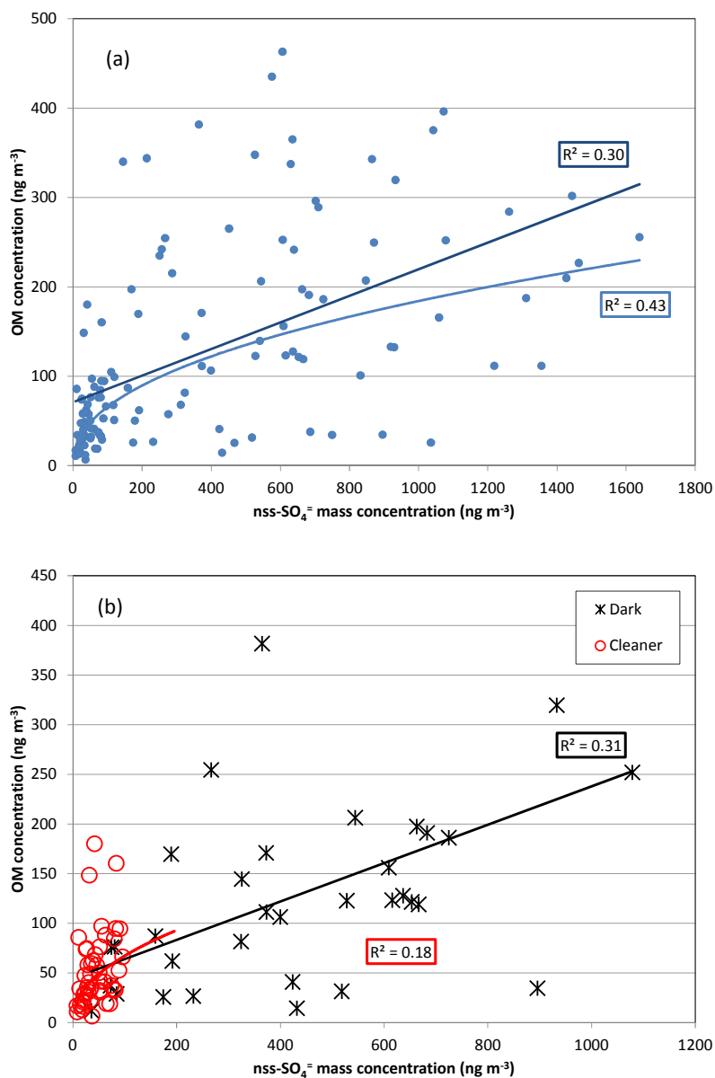
5 Figure 8. Regressions of OM versus nss-SO 4 = for a) all weeks and b) for dark weeks (during NDJF) and cleaner weeks (nss-SO 4 = <100 ng m -3 ). Coefficients of determination are indicated. Linear and power-law regressions are shown for all points (p<0.01), and linear regressions for the dark period (p<0.01) and the cleaner period (p<0.03).
