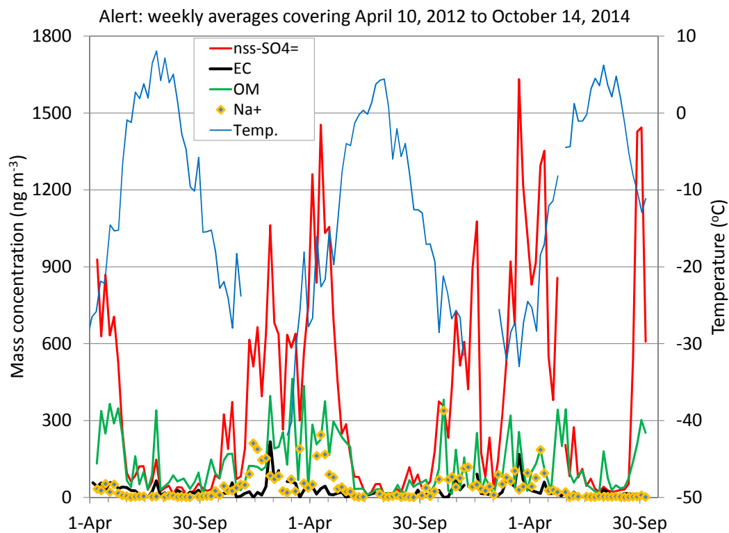
5 Figure 2. Time series of temperature and weekly-integrated mass concentrations of OM, EC, nss-SO 4 - and Na + for the study period: April, 10, 2012 to October, 14, 2014.
