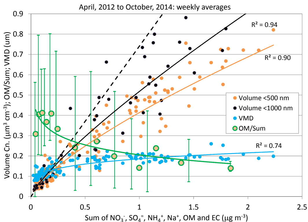
Figure 3. Scatter plot of volume concentrations, ratio of OM to the sum of other measured chemical components ( \text{NO}_3^- , \text{SO}_4^{2-} , \text{NH}_4^+ , \text{Na}^+ and EC) and particle sizes (from SMPS) as a function of the “Sum” of all major chemical components (OM, \text{NO}_3^- , \text{SO}_4^{2-} , \text{NH}_4^+ , \text{Na}^+ and EC). Volume concentrations are shown for particles <500 nm diameter (SMPS only) and particles <1000 nm diameter (SMPS+OPC). Values of OM/Sum are averaged over successive 10 values of the ‘Sum’ to reduce scatter. The error bars represent the range of values of OM/Sum for each 10-point average. The dashed curve is the volume vs mass concentration for a constant density of 1.35 \text{ g cm}^{-3} calculated using equation 1 as the average for the lower mass concentration points ( <0.25 \mu\text{g m}^{-3} ).
