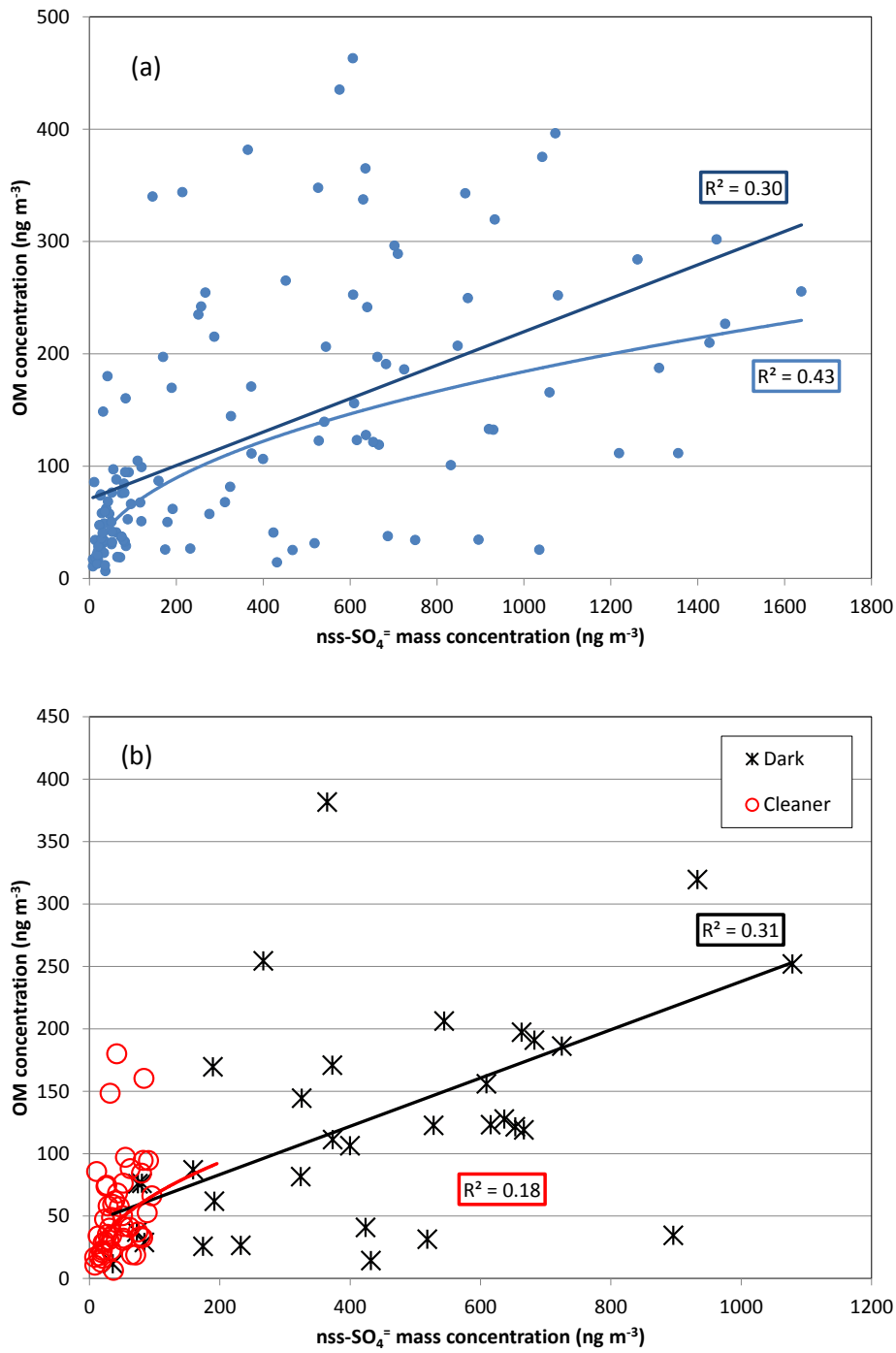
Figure 8. Regressions of OM versus nss-SO 4 = for a) all weeks and b) for dark weeks (during NDJF) and cleaner weeks (nss-SO 4 = < 100 ng m -3 ). Coefficients of determination are indicated. Linear and power-law regressions are shown for all points (p < 0.01), and linear regressions for the dark period (p < 0.01) and the cleaner period (p < 0.03).
