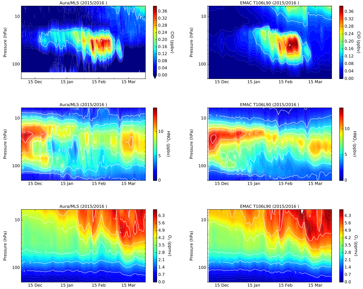
Figure 13. Temporal evolution of daily mean \text{ClO} , \text{HNO}_3 and \text{O}_3 at northern high latitudes (averaged over 70\text{--}90^\circ\text{N} ) as function of pressure as observed by Aura/MLS (left) and simulated by EMAC T106L90 (right) for the Arctic winter 2015/2016 (EMAC SORBIT output used).
