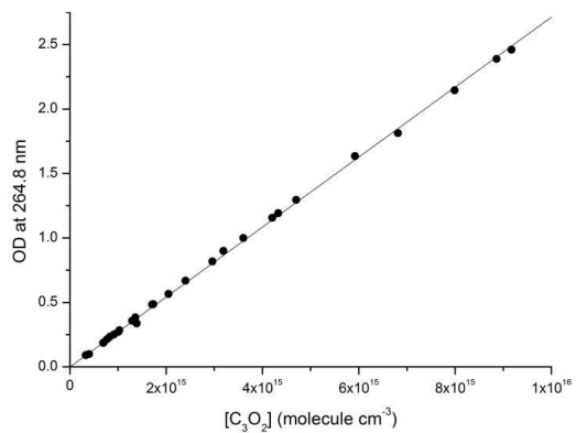
Figure 2: Beer-Lambert plot of optical density at 264.8 nm versus [C 3 O 2 ]. The line is an unweighted proportional fit to the data with a slope of 2.71 \times 10^{-16} \text{ nm cm}^3 \text{ molecule}^{-1} .
