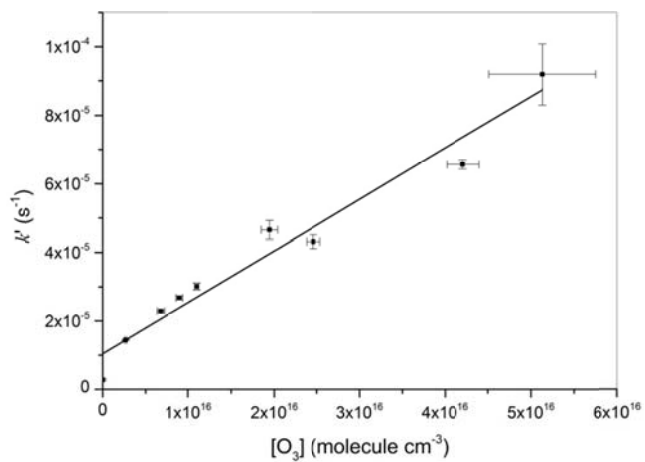
Figure 10: Pseudo-first-order decay constant of C_3O_2 plotted against the O_3 concentration. The slope is the bimolecular rate constant k_6 . The horizontal error bars represent uncertainty in the O_3 concentration based on analysis of three different spectral regions (see text). The vertical error bars are 2\sigma from the fits to data as shown in Figure 9.
