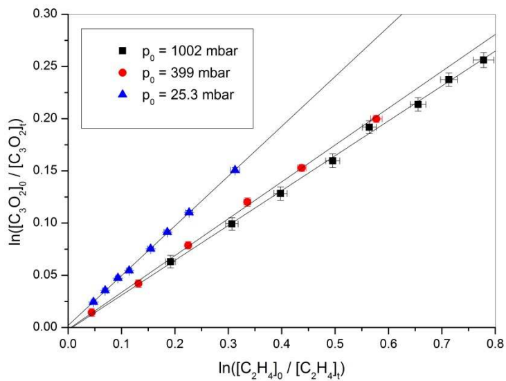
Figure 6: Depletion factors for C_3O_2 versus C_2H_4 during reaction of both traces gases with OH at three different pressures. Error bars are 2\sigma as returned by the least-squares fitting routine. The slope at each pressure yields the relative rate constant ratio k_4 / k_5 .
