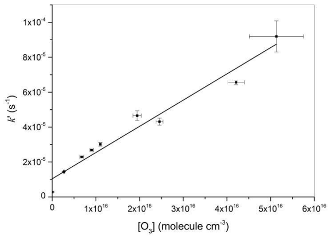
Figure 10: Pseudo-first-order decay constant of C 3 O 2 plotted against the O 3 concentration. The slope is the bimolecular rate constant k_6 . The horizontal errors bars represent uncertainty in the O 3 concentration based on analysis of three different spectral regions (see text). The vertical error bars are 2\sigma from the fits to data as shown in Figure 9.
