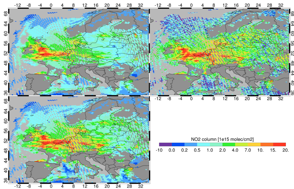
Figure 3: Example result of the assimilation of OMI NO 2 tropospheric column amounts (DOMINO-2 product, upper right) on 26 March 2007 in the LOTOS-EUROS regional air quality model (model simulation for OMI ground pixels is provided in the upper left by spatial interpolation and by applying the averaging kernels). LOTOS-EUROS makes use of the ensemble Kalman filter to optimise model processes by assimilating observations. In this case the surface NO x emissions are adjusted to optimise the match with the tropospheric NO 2 columns observed. The resulting analysis is shown in the lower-left panel. OMI observations for cloud-covered scenes (cloud radiance fraction > 50%) are removed.
