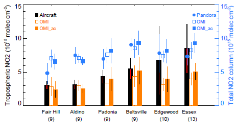
Figure 16: Comparison of average tropospheric (orange bars) and total (blue squares) \text{NO}_2 columns determined from in situ aircraft (black bars) measurements and total columns retrieved from Pandora (filled blue circles) at the six locations in Maryland during the DISCOVER-AQ field campaign (from Lamsal et al., 2014). Open bars and squares represent the operational retrievals and filled bars and squares represent the retrievals performed using collocated aircraft-measured \text{NO}_2 vertical profiles. The vertical lines represent the standard deviation of the average.
