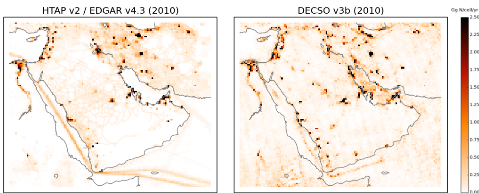
Figure 5: NO x emissions in the Middle East in 2010 derived from (left) the bottom-up inventory EDGAR v4.3 and (right) the DECOSO algorithm v3b applied to OMI NO 2 observations.
