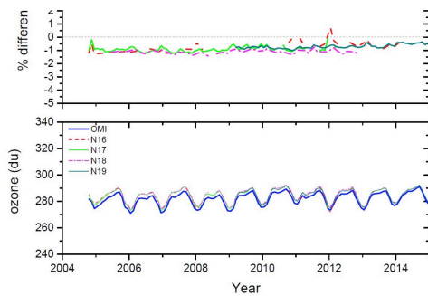
5 Figure 11: Total column ozone from OMI and four NOAA SBUV instrument (bottom) and differences in % of OMI minus each SBUV instrument (top) (adapted from McPeters et al., 2013).
