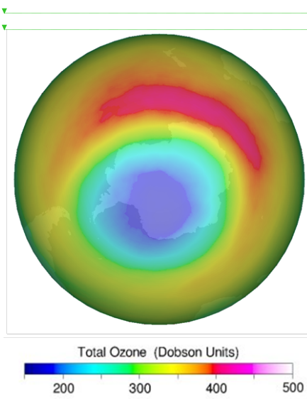
Figure 9: October 2017, monthly average OMI total ozone column over Antarctica.
