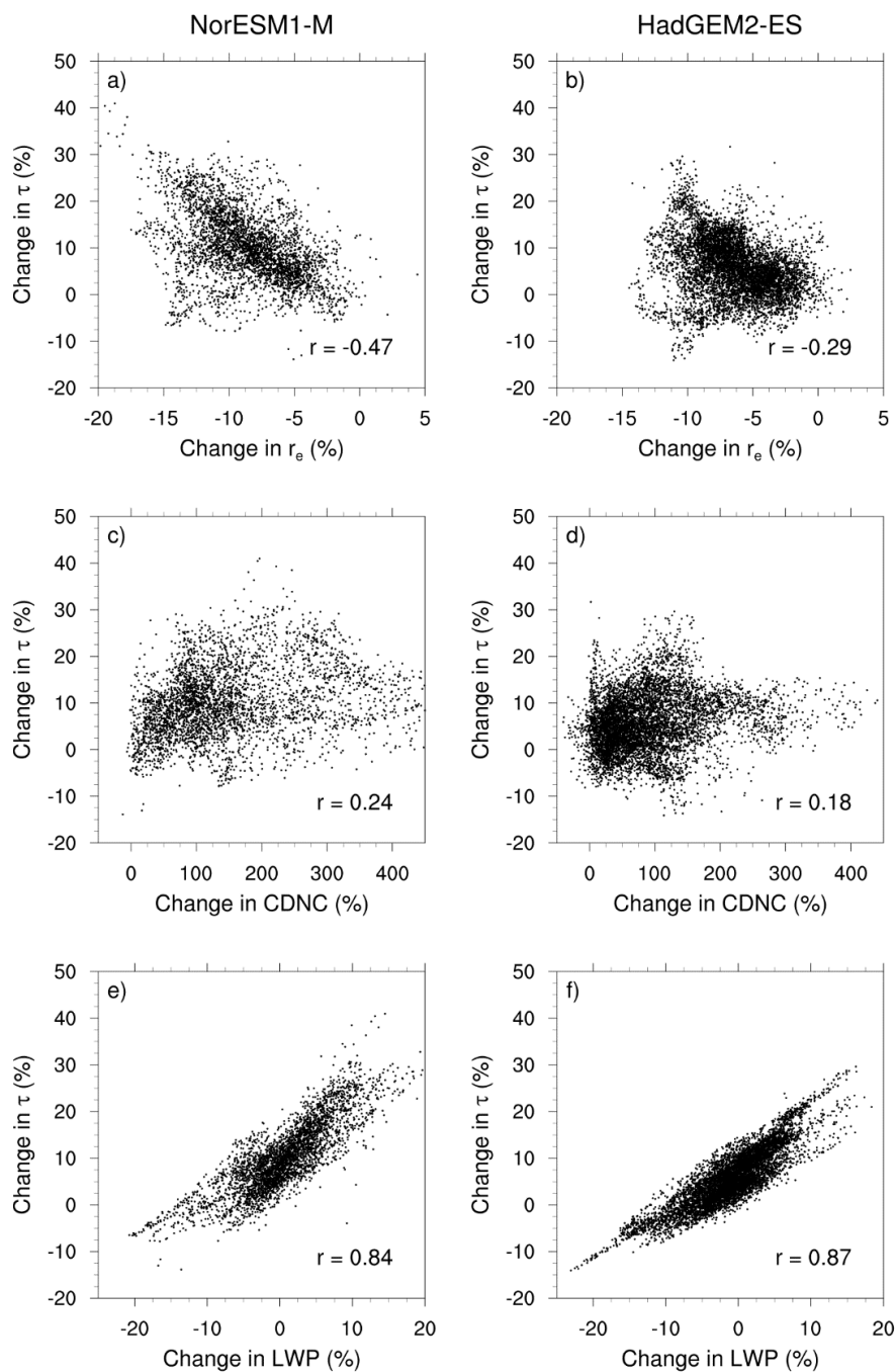
Figure 9. Relations between the relative change in cloud optical depth ( \tau ) due to sea salt injection against the corresponding changes in r_e for a) NorESM1-M and b) HadGEM2-ES; CDNC for c) NorESM1-M and d) HadGEM2-ES; and LWP for e) NorESM1-M and f) HadGEM2-ES. The relations represent averages over the period 2035-2065 within the injection area. Pearson's correlation coefficient ( r ) is given for each relation.
