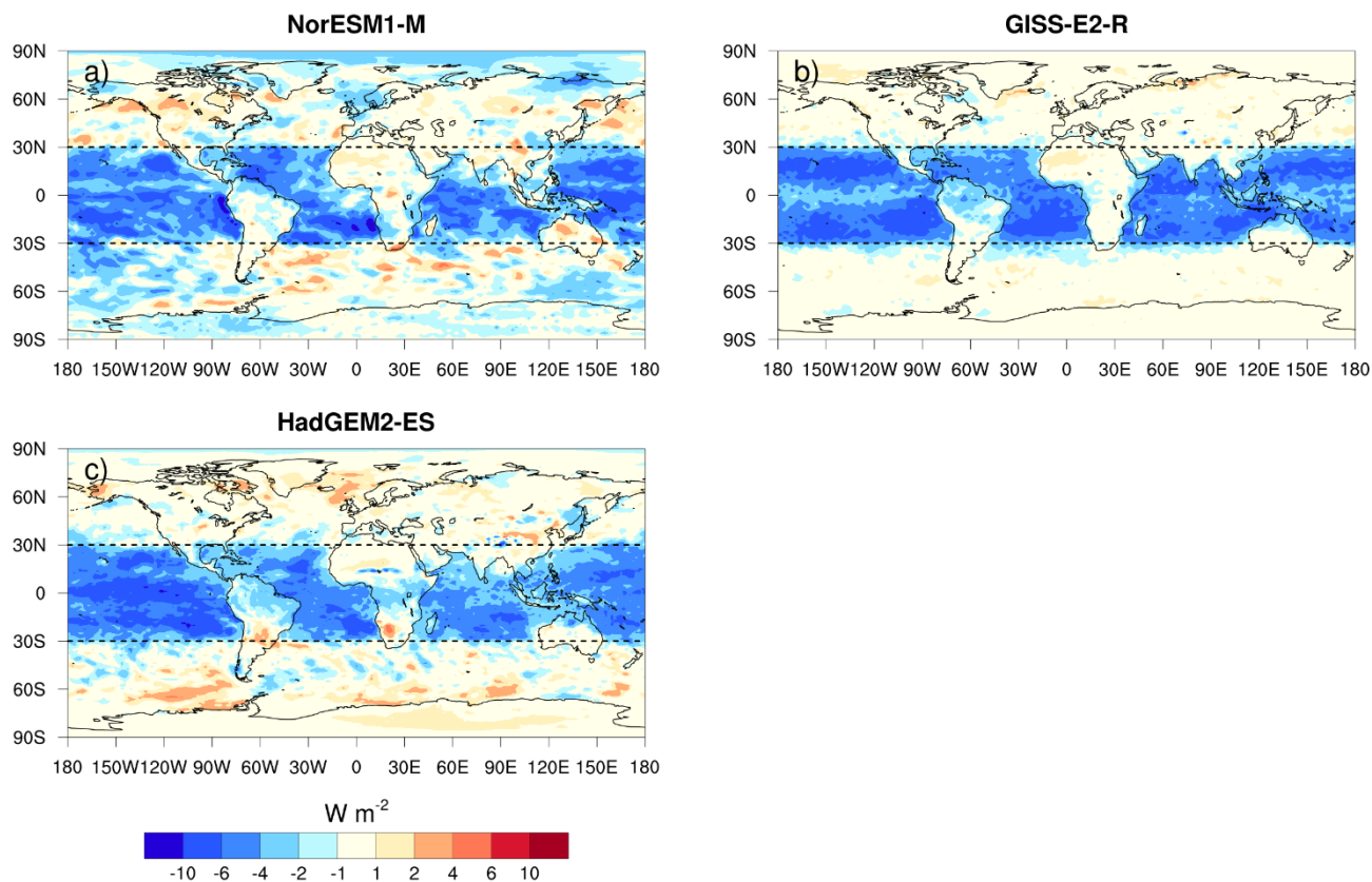
Figure 3. TOA mean effective radiative forcing over the 10 years of simulation with fixed SST for a) NorESM1-M, b) GISS-E2-R, and c) HadGEM2-ES.
