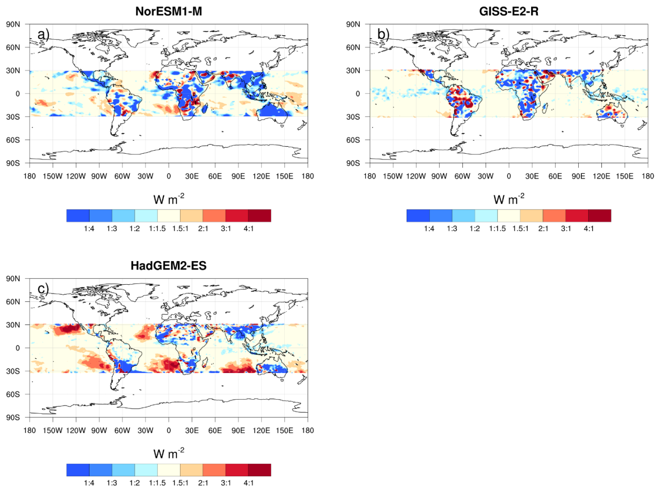
Figure 4. The ratio of the total ERF to the clear-sky ERF at the TOA averaged over the 10 years of simulation with fixed SST for a) NorESM1-M, b) GISS-E2-R, and c) HadGEM2-ES.
