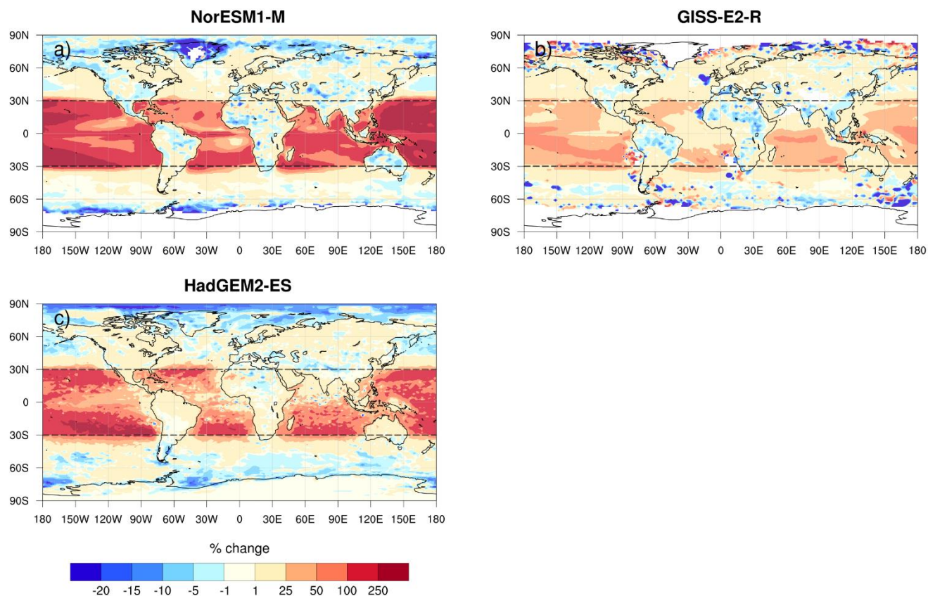
Figure 6. Mean relative change in CDNC due to sea salt injection for NorESM1-M (a), GISS-E2-R (b), and HadGEM2-ES (c). CDNC represents the cloud droplet number concentration within the model layer below 700 hPa with maximum concentration, and the maps represent averages over 2035-2065.
