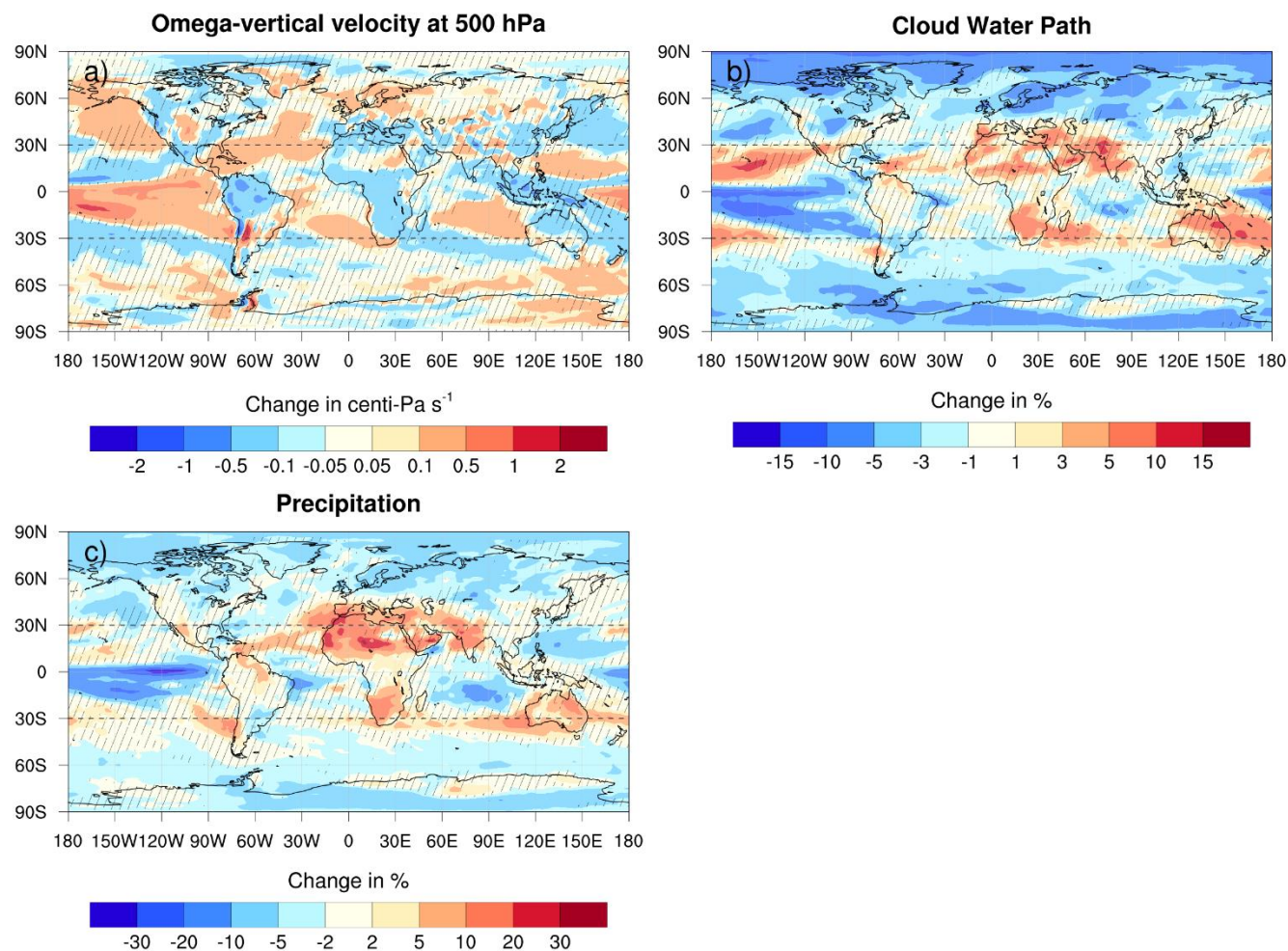
Figure 8. The multi-model mean difference between the G4sea-Salt experiment and RCP4.5 averaged over years 2035-2065. The multi-model mean difference refers to the mean of all three models, NorESM1-M, GISS-E2, and HadGEM2-ES. Hatching denotes areas where the models disagree on the sign of the change. Change in a) Omega-vertical velocity at 500 hPa (positive values corresponds to reduced upward motion) (centi-Pa s -1 ), b) Cloud Water Path (vertically-integrated cloud water content) (%), and c) Precipitation rate (%).
