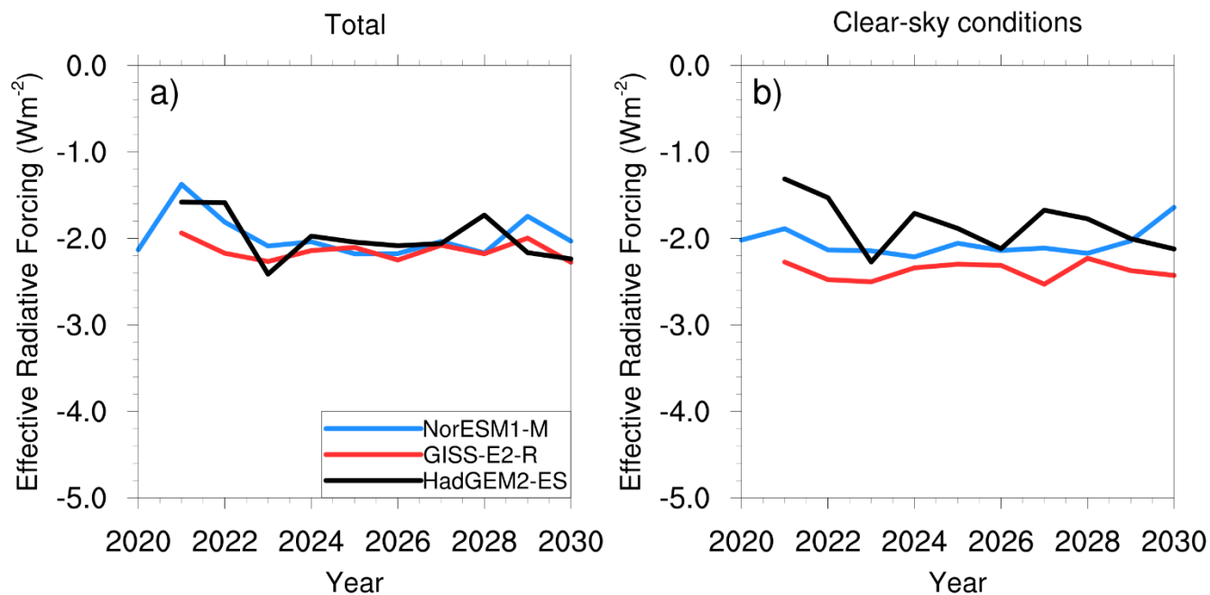
Figure 2. Global-mean TOA effective radiative forcing of the injected particles in total (a) and in clear-sky conditions (b). The ERF for each model was determined from 10-year simulations with fixed SST with and without sea salt injection.
