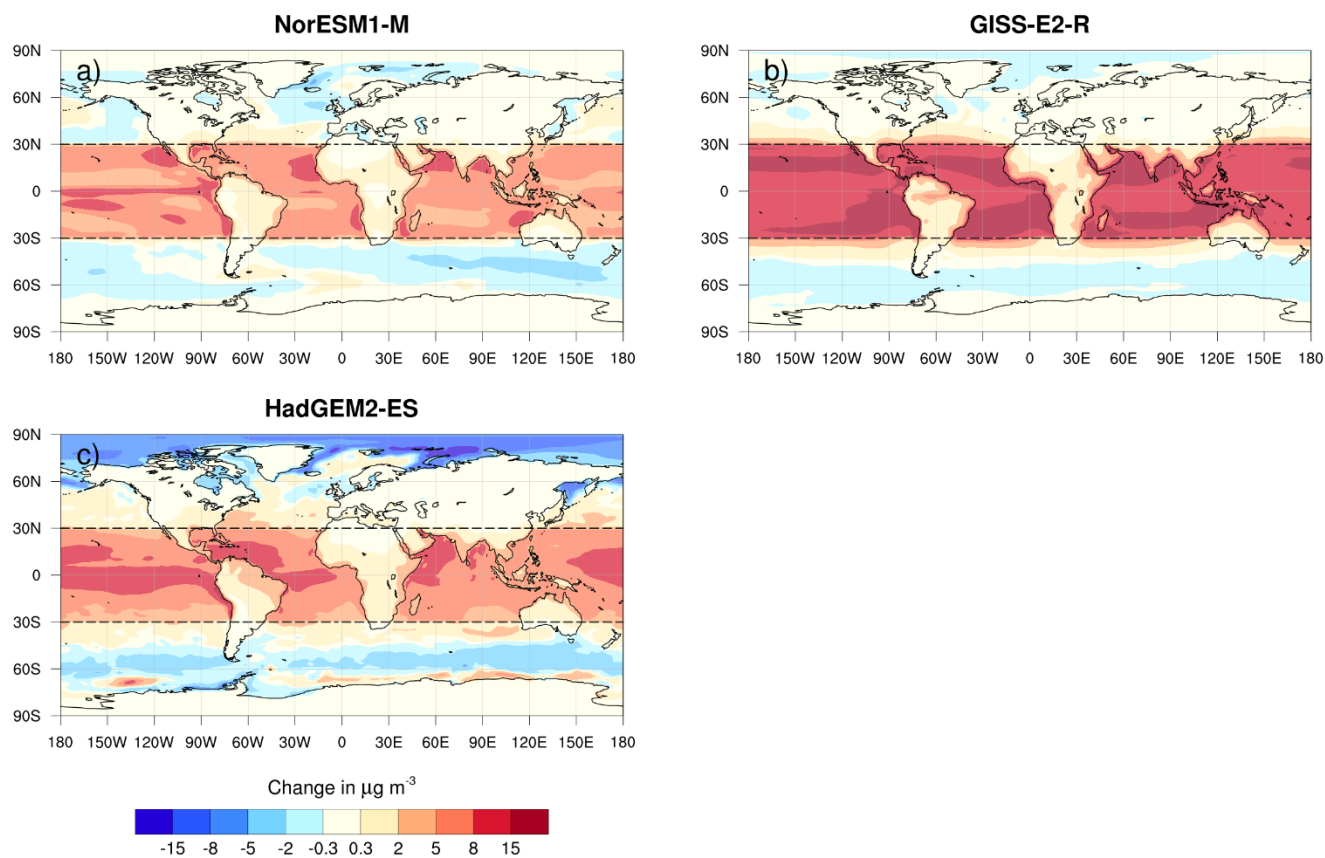
Figure 5. Mean difference in sea salt mass concentration in the lowest model layer between G4sea-Salt and RCP4.5 averaged over 2035 and 2065, for a) NorESM1-M, b) GISS-E2-R, and c) HadGEM2-ES.
