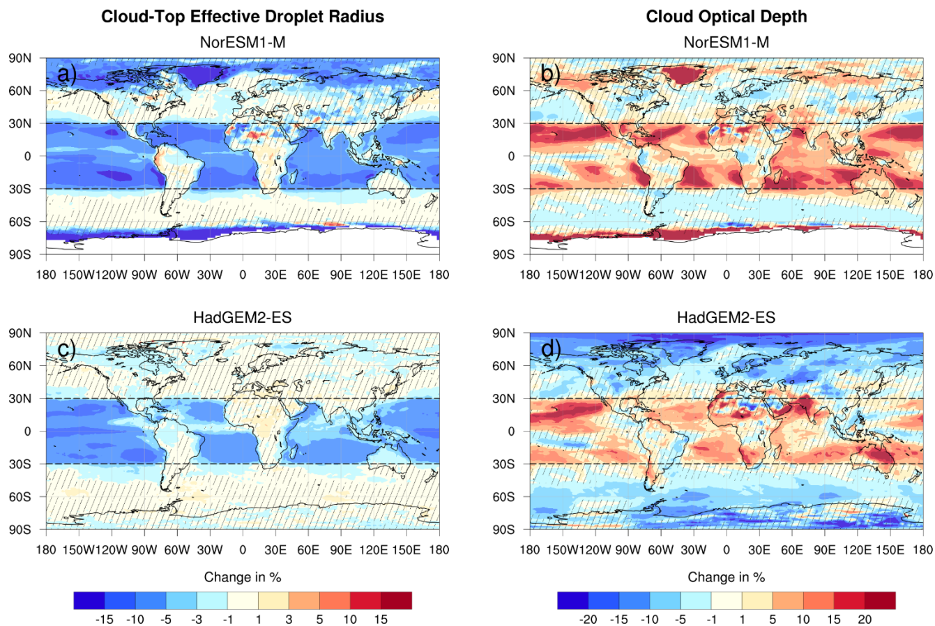
Figure 7. Mean relative change between G4sea-Salt and RCP4.5 in Cloud-Top Effective Radius for NorESM1-M (a) and HadGEM2-ES (c), and in Cloud Optical Depth for NorESM1-M (b) and HadGEM2-ES (d). The maps represent average change due to sea spray climate engineering over the period 2035-2065. Hatching denotes areas where changes are not significant at the 95% confidence level (Student t-test with respect to variance of annual mean values).
