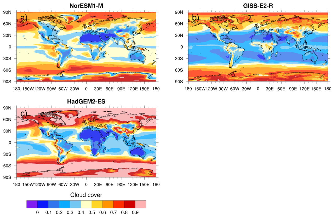
Figure 1. Cloud fraction for low clouds averaged over 2020-2030 within the RCP4.5 scenario for a) NorESM1-M, b) GISS-E2-R, and c) HadGEM2-ES. Cloud fractions have been estimated by assuming the random overlapping assumption for layers 5 below 850 hPa (a and c) and below 600 hPa (b).
