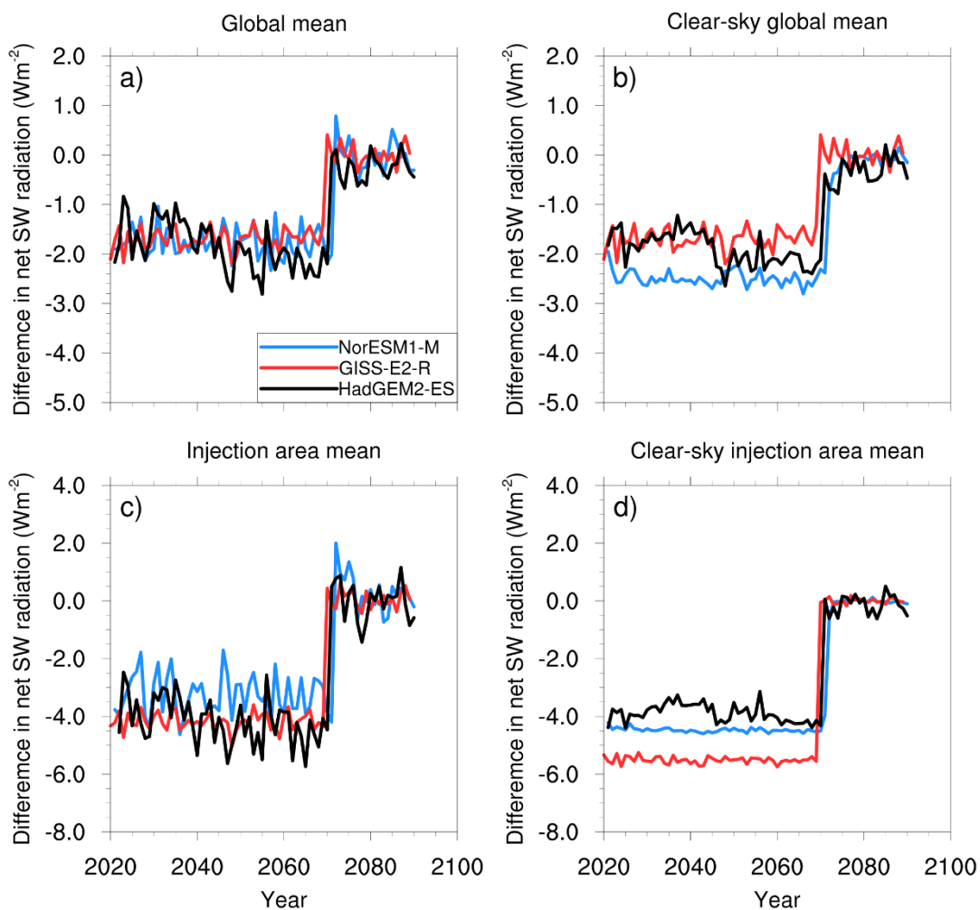
Figure 10. Difference in net SW radiation at the TOA between G4sea-Salt and RCP4.5 a) global mean, b) clear-sky global mean, c) injection area mean, and d) clear-sky injection area mean. The colors denote NorESM1-M (blue), GISS-E2-R (red), and HadGEM2-ES (black). Only grid cells over ocean have been included in the mean values representative of the injection area.
