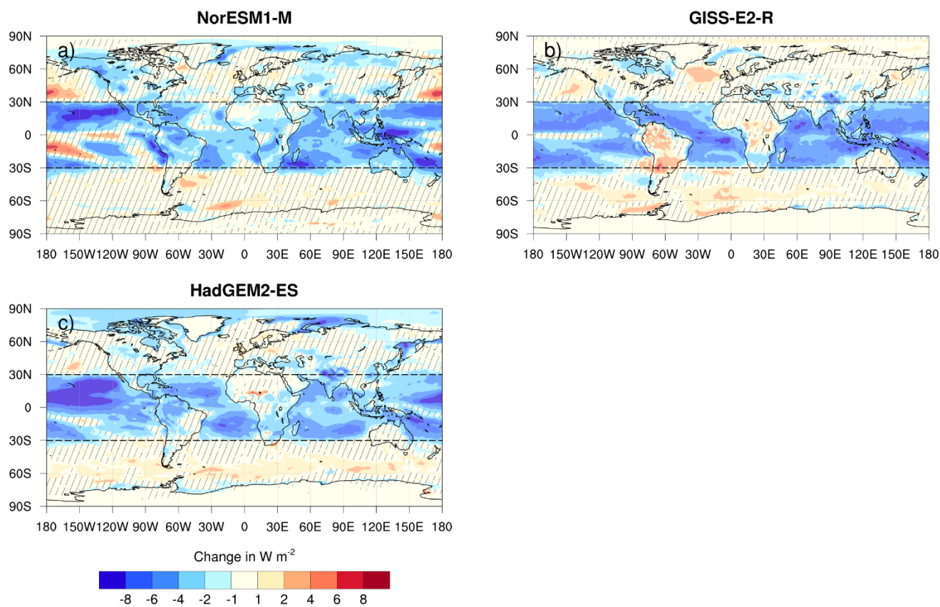
Figure 11. Mean change in net SW radiation [W m -2 ] at the TOA between G4sea-Salt and RCP4.5 for the period 2035-2065 for a) NorESM1-M, b) GISS-E2-R, and c) HadGEM2-ES. Hatching denotes areas where changes are not significant at the 95% confidence level (Student t-test with respect to variance of annual mean values).
