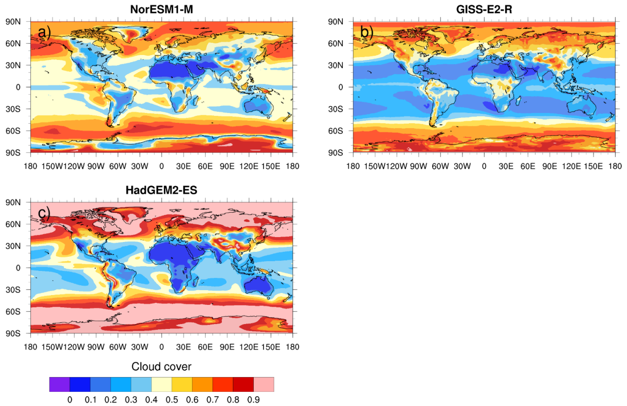
Figure 2. Cloud fraction for low clouds averaged over 2020-2030 within the RCP4.5 scenario for a) NorESM1-M, b) GISS-E2-R, and c) HadGEM2-ES. Cloud fractions have been estimated by assuming random overlapping for layers below 850 hPa (a and c) and below 600 hPa (b).
