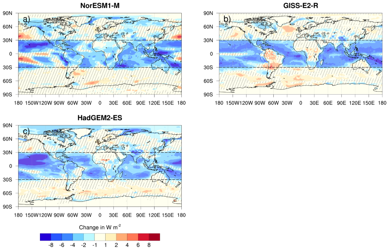
Figure 12. Mean change in net SW radiation [ W m^{-2} ] at the TOA between G4sea-Salt and RCP4.5 for the period 2035-2065 for a) NorESM1-M, b) GISS-E2-R, and c) HadGEM2-ES. Hatching denotes areas where changes are not significant at the 95% confidence level (Student t-test with respect to variance of annual mean values).
