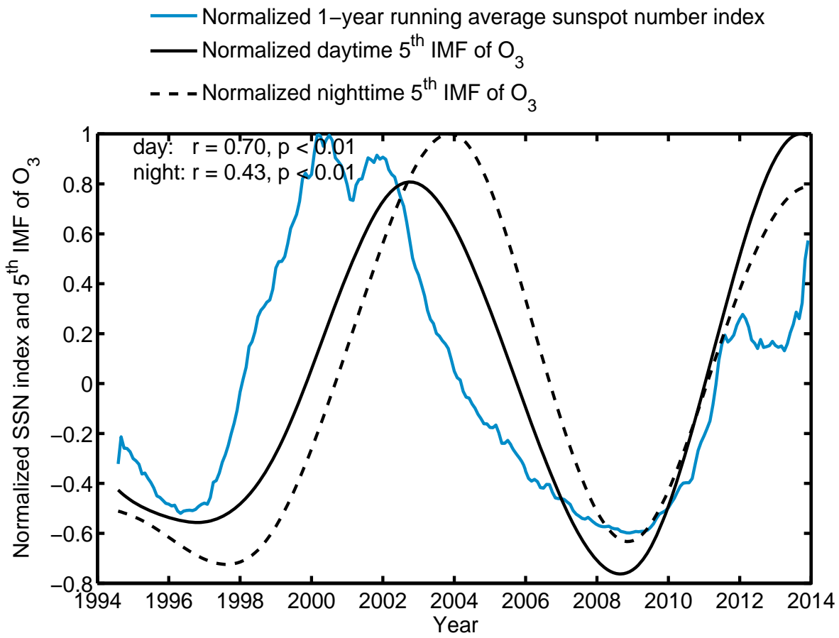
Figure 17 Comparison between the 5th IMF and the 1-year running average SSN during 1994-2013.
