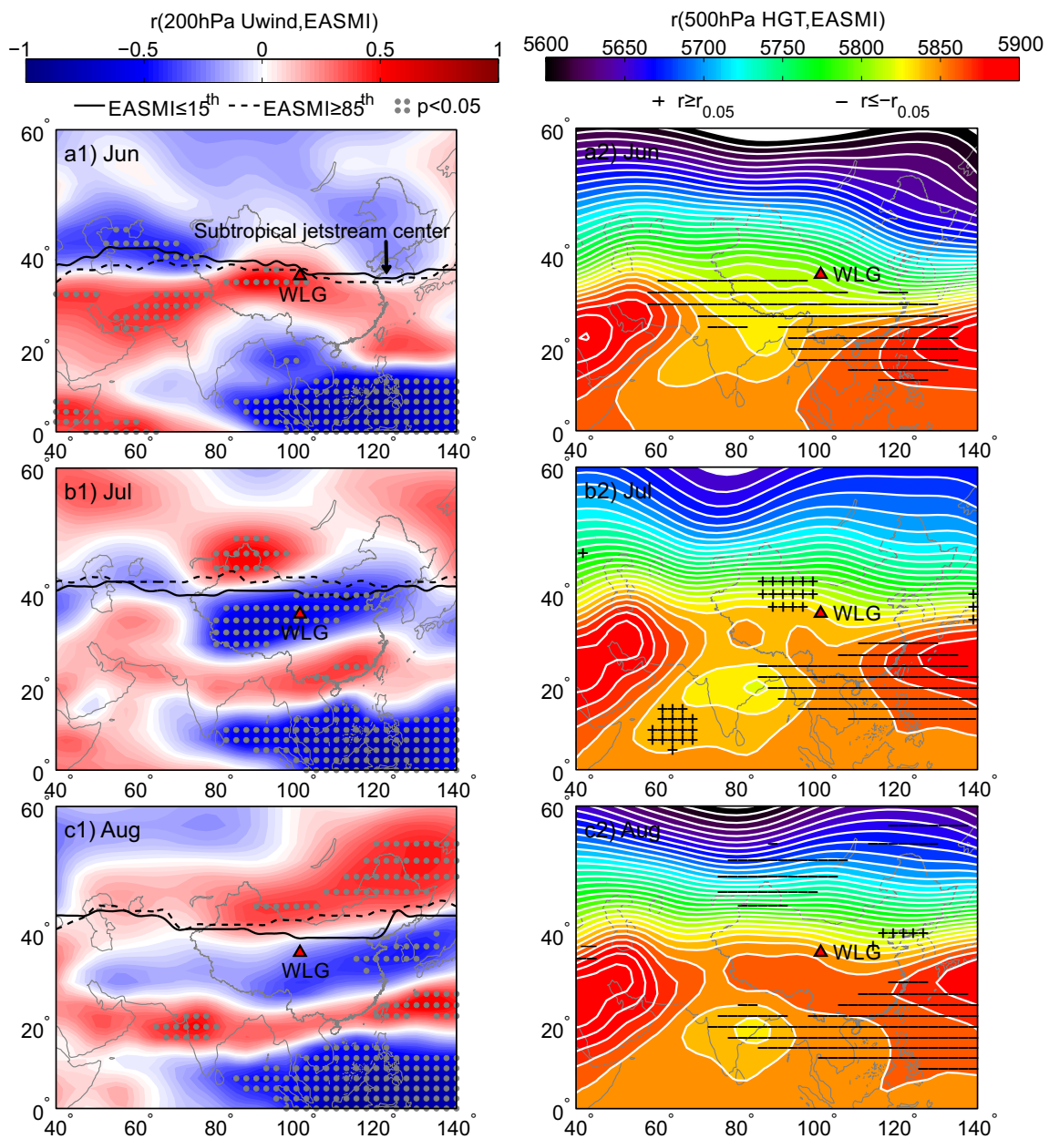
Figure 16 1) The correlation coefficient between the 200hPa zonal wind and the EASMI and the average location of the subtropical jetstream center for the EASMI \leq 15^{\text{th}} and EASMI \geq 85^{\text{th}} cases and 2) the average 500hPa geopotential height and the location of significant positive(+)/negative(-) correlation ( p < 0.05 ) between 500hPa geopotential height and the EASMI in a) Jun, b) Jul and c) Aug during 1990 to 2015.
