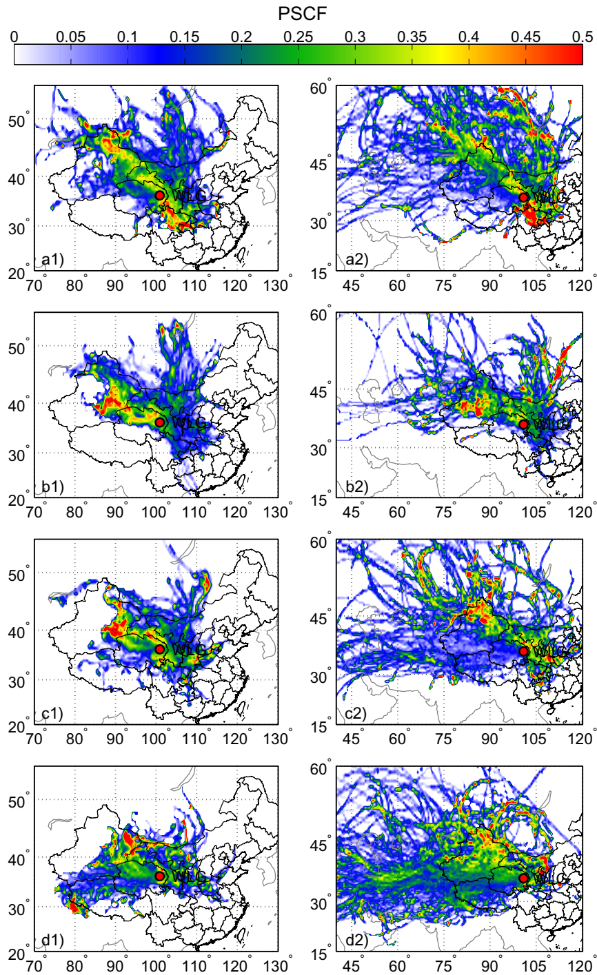
Figure 1 The 1994-2013 climatology of air mass origins at WLG in the PBL (left) and FT (right) for spring (a), summer (b), autumn (c) and winter (d), based on the PSCF analysis of ozone concentrations higher than the 75th percentile value (Sect. 2.3).
