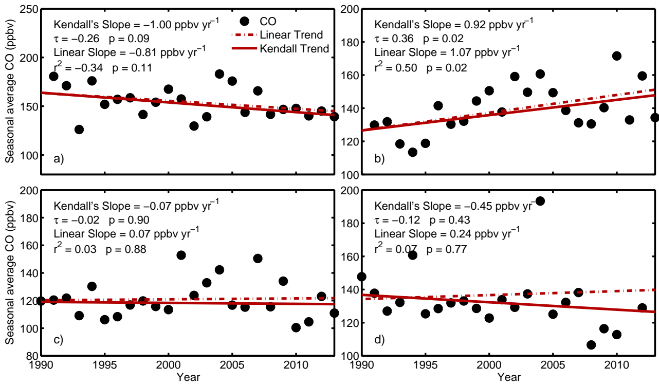
Figure 10 Mann-Kendall and linear trends of seasonal average CO observed during a) spring, b) summer, d) autumn and d) winter from 1990-2013 at WLG
