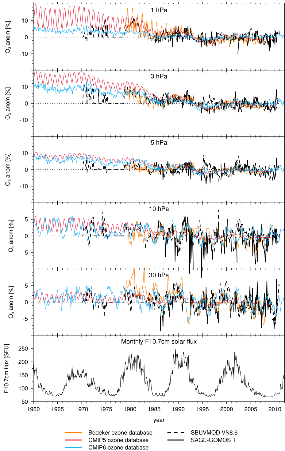
Figure 4. Timeseries of deseasonalised percent tropical (30°S-30°N) ozone anomalies from two satellite observation datasets (black) and the Bodeker (orange), CMIP5 (Cionni et al., 2011) (red), and CMIP6 (blue) ozone databases over the period 1960-2011 at (a) 1 hPa, (b) 3 hPa, (c) 5 hPa, (d) 10 hPa and (e) 30 hPa. The lowest panel shows the F10.7 cm solar flux for reference. Anomalies are shown relative to a baseline period 1985-2009.
