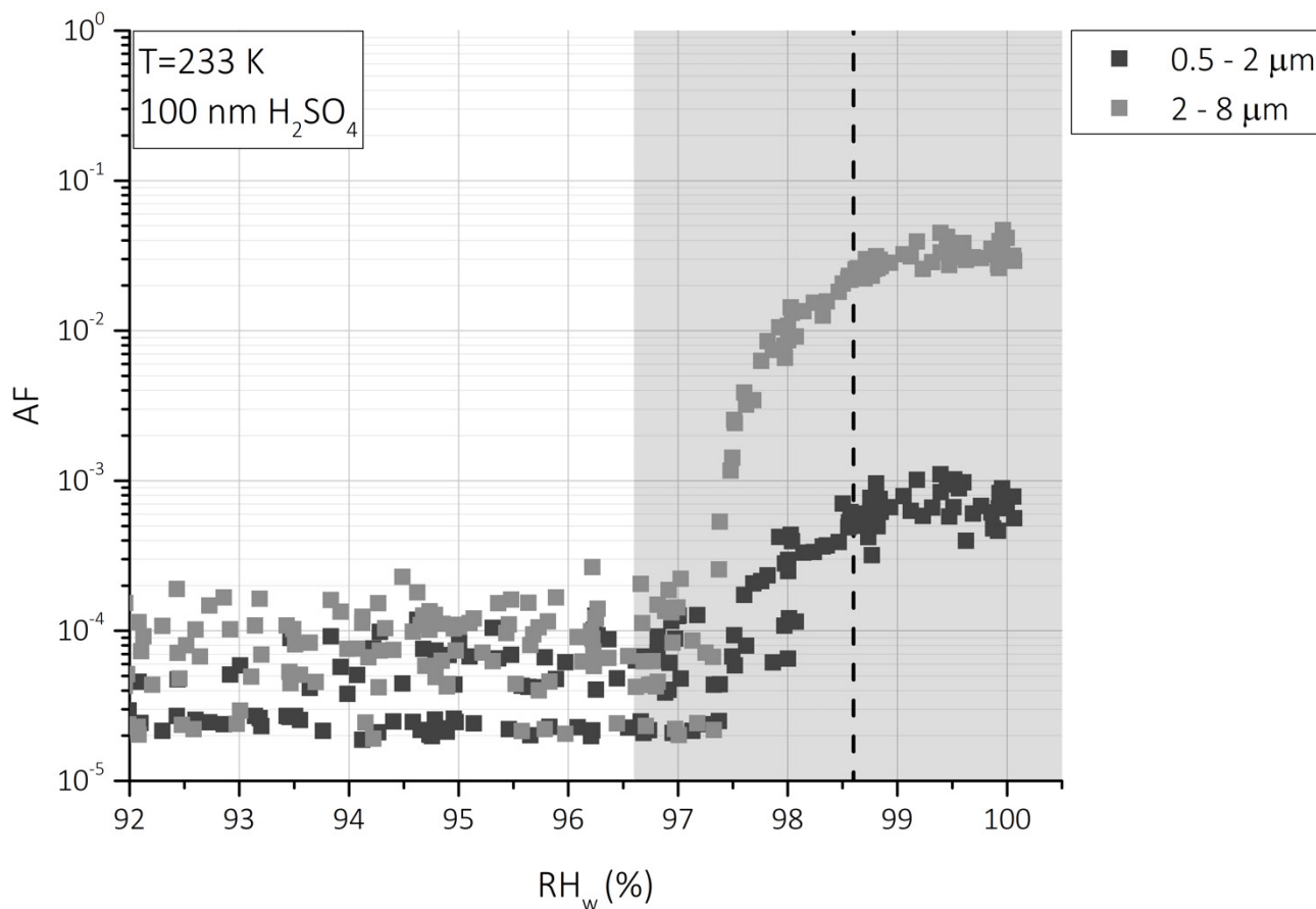
Fig. 2: Homogeneous freezing curve of 100 nm dry diameter \text{H}_2\text{SO}_4 particles. AF as a function of \text{RH}_w at 233 K in the size channel 0.5 – 2 \mu\text{m} (dark grey) and 2 – 8 \mu\text{m} (light grey). The dashed line ( \text{RH}_w = 98.6\% ) represents the expected \text{RH}_w for homogeneous freezing of dilute solution drops of an initial dry diameter of 100 nm (Koop et al., 2000a), and the shaded region indicates the calculated range of \text{RH}_w and uncertainty to which the particles in the aerosol layer in HINC are exposed to.
