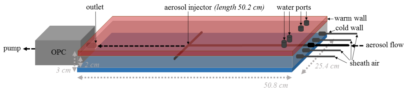
10 Fig. 1: Schematic and outer dimensions of HINC (main chamber).
