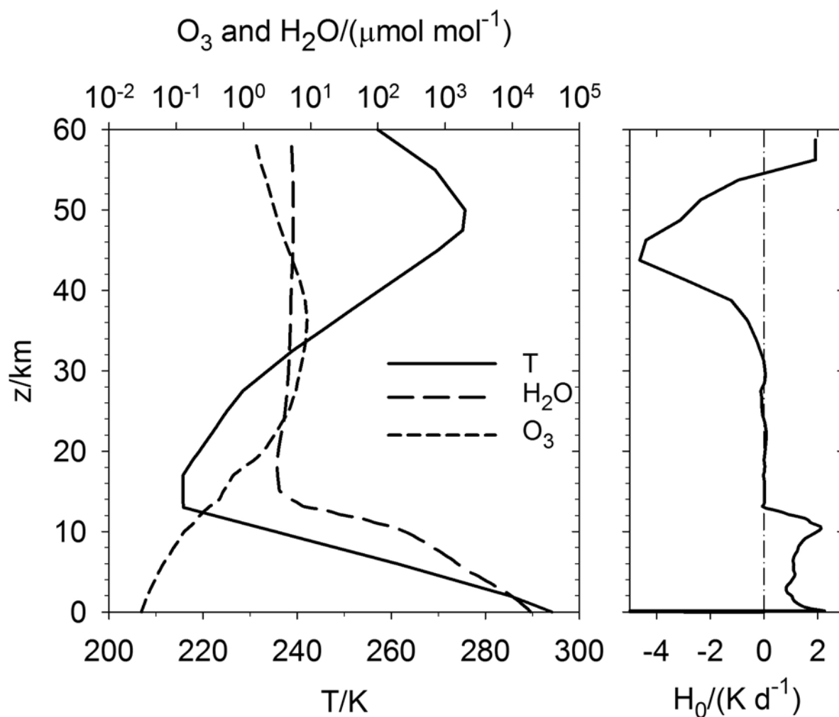
725 Figure 1. Temperature T of the mid-latitude summer standard atmosphere versus height z , together with water vapor and ozone molar mixing ratio ( O_2 : 0.2002 \text{ mol mol}^{-1} ; CO_2 : 360 \mu\text{mol mol}^{-1} ), and heating rate H_0 = Q_0/(\rho c_p) keeping the atmosphere at steady-state. Because of TOA radiative imbalance, H_0 is strongly negative at the surface; in the mass-weighted average, H_0 = -1.25 \text{ K d}^{-1} in the troposphere and -0.057 \text{ K d}^{-1} in the stratosphere, balancing the summer warming.
