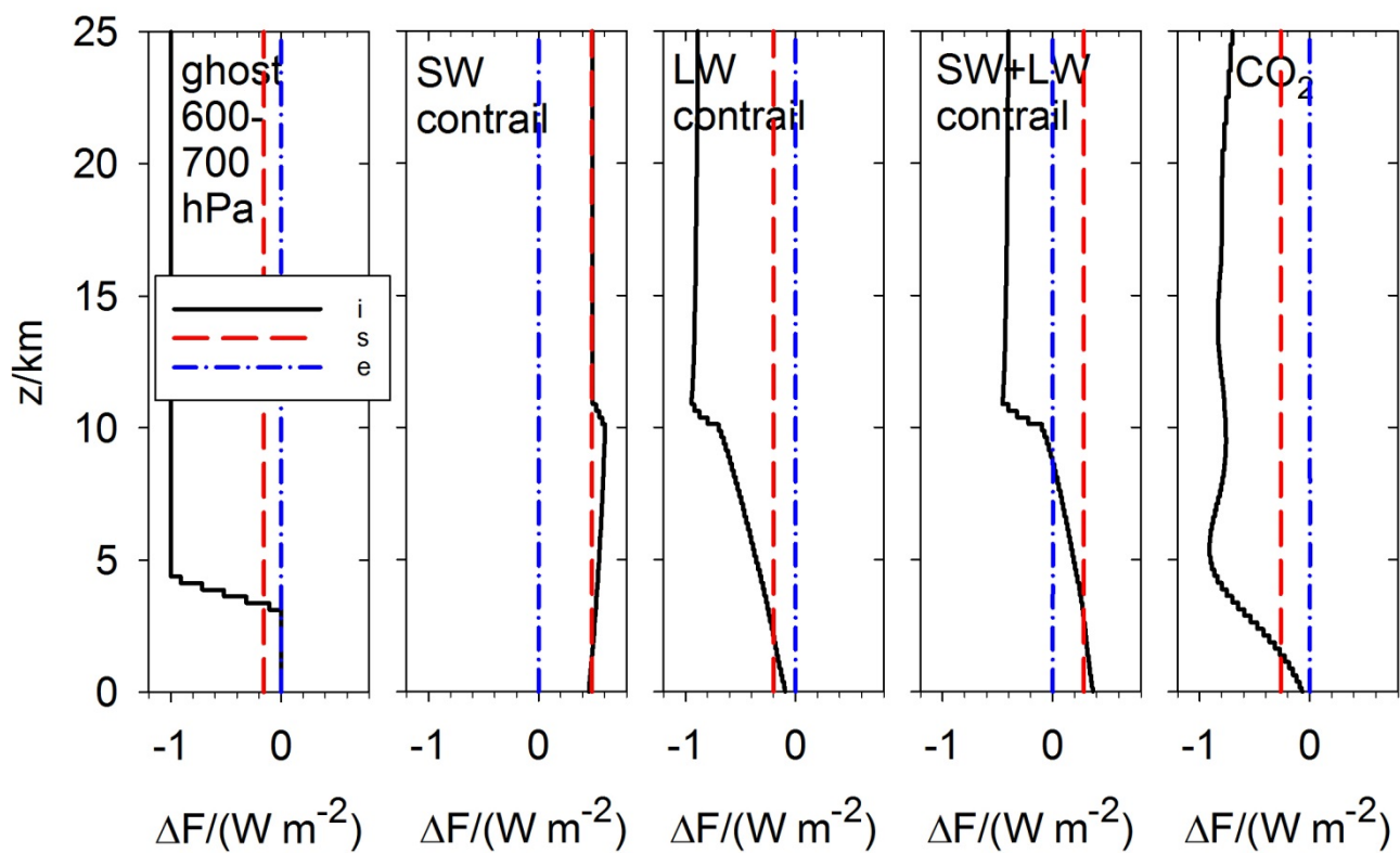
Figure 5. Initial and final radiative flux changes \Delta F versus height z as induced by a disturbance from added ghost heating, SW, LW, and SW+LW contrail cirrus, and 10 % increased CO 2 , in the panels from left to right, respectively. Black full lines (i): instantaneous flux; red dashed line (s): adjusted to constant surface temperature; blue dash-dotted line (e): equilibrium over adiabatic surface. The fluxes F are positive if upwards.
