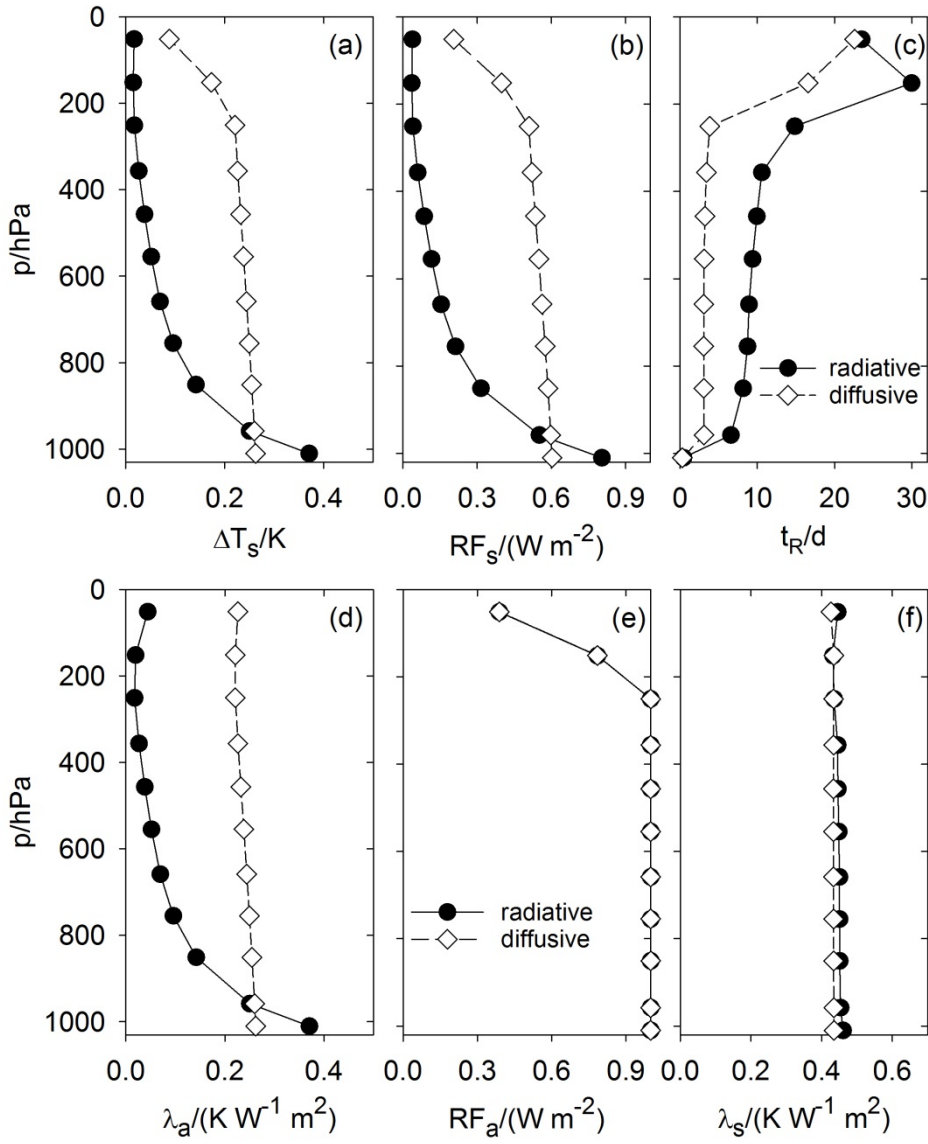
Figure 7: (a) Temperature change at the surface for layer heating versus the layer pressure height. The ghost forcing corresponds to an RF_1 of 1 W m^{-2} at TOA. Black symbols with full line: radiative case; white symbols with dashed line: radiative-diffusive case. (b) Corresponding RF_s values for fixed T_s . (c) Relaxation time scales t_R = \Delta T_{layer}/H . (d) Climate sensitivity parameter \lambda_a = \Delta T_s/RF_a based on stratosphere-adjusted RF_a ; (e) RF_a ; (f) climate sensitivity parameter \lambda_s = \Delta T_s/RF_s based on effective RF_s .
