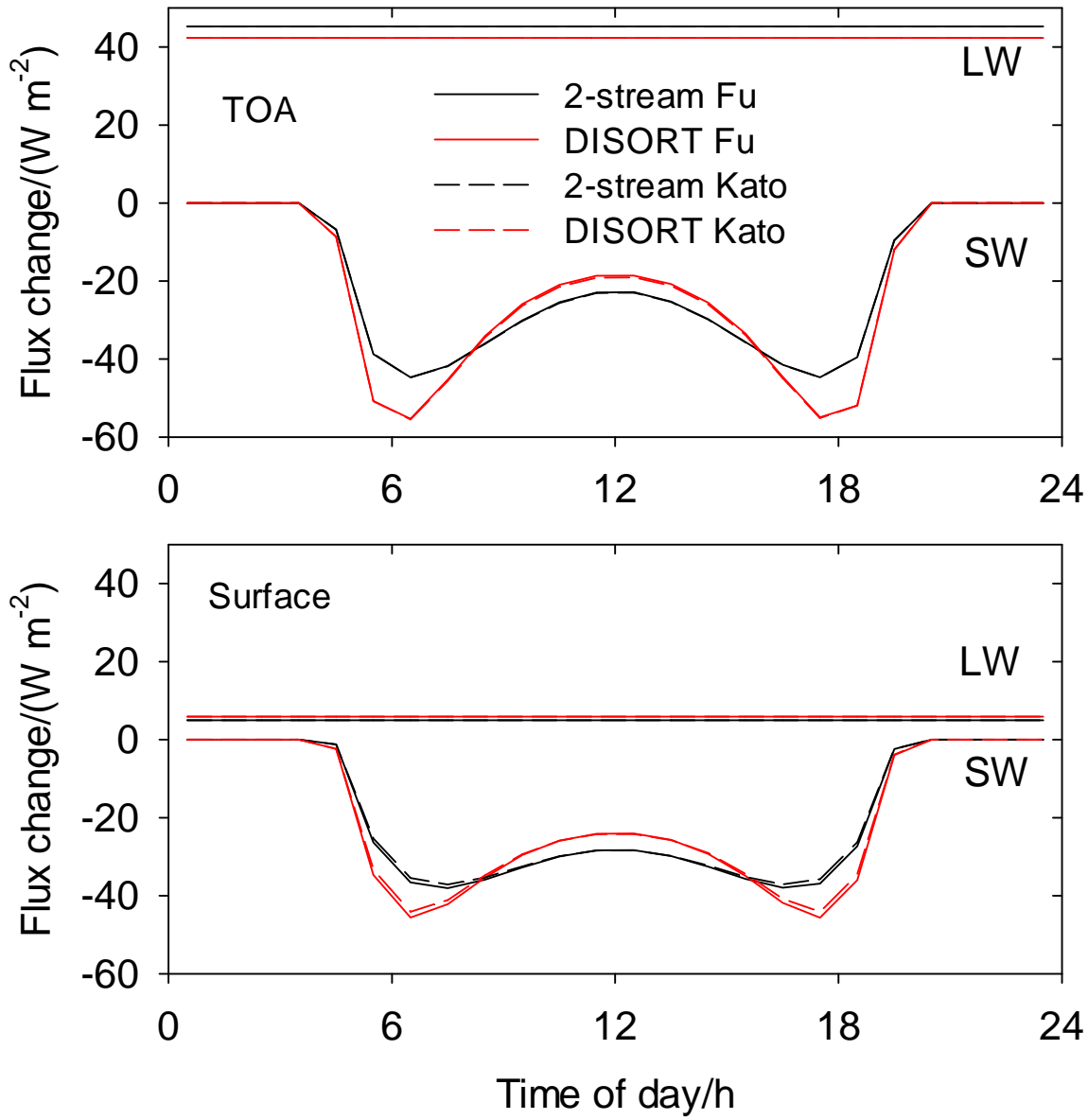
740 Figure 3. LW and SW flux changes versus time of day at TOA and at the surface, for two-stream and DISORT solvers, and 745 for Fu & Liou and Kato shortwave molecular absorption parametrizations. The model parameters are the same as in Figure 2, \tau = 0.5 . The flux differences for different molecular absorption models of Fu and Kato are far smaller than between the two-stream solver and DISORT.
