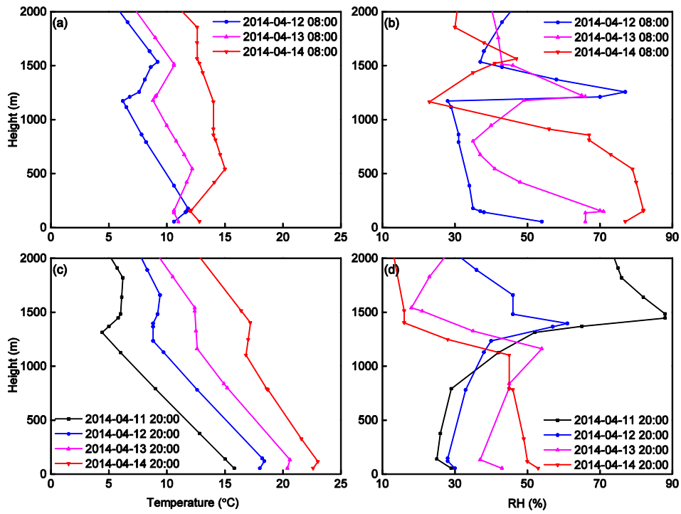
Figure 9: The temperature and RH profiles during the whole haze event in Beijing city. (a) temperature and (b) RH at 8:00 LST. (c) temperature and (d) RH at 20:00 LST.
