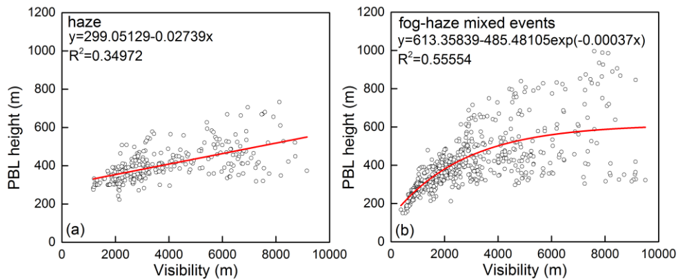
10 Figure 4: Relationship between visibility and PBL height for (a) haze and (b) fog-haze mixed events from January 2014 to March 2015 in Beijing city
