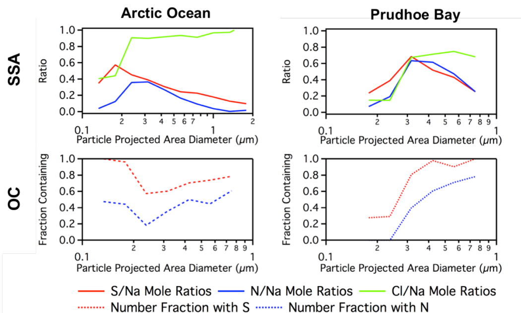
Figure S4. S/Na, N/Na, Cl/Na mole ratios of individual SSA (top) and fraction of OC particles (bottom) containing S, N, and/or Cl, measured by CCSEM-EDX for Arctic Ocean and Prudhoe Bay influenced air masses. Size bins with less than 25 particles are not displayed.
