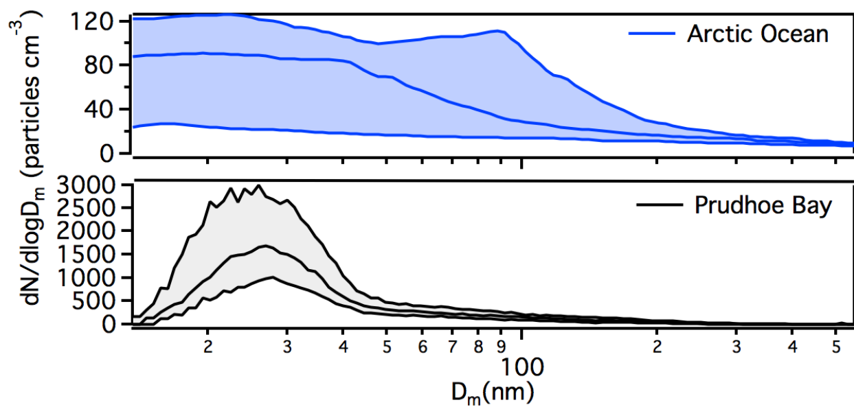
130 Figure S3. Median, as well as 25 th and 75 th percentile, particle size distributions, measured by SMPS, during Prudhoe Bay and Arctic Ocean influenced air masses from August 21–September 20, 2015.
