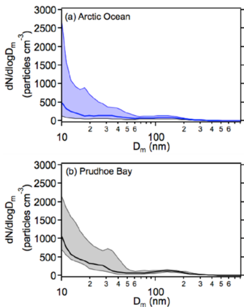
Figure 3. Particle number distribution ( 10 – 810 nm mobility diameter ) for (a) Arctic Ocean and (b) Prudhoe Bay air masses observed for August-September 2008, 2009, 2013, and 2014 (median shown by the solid line, 25 th and 75 th percentiles shaded) at the NOAA Barrow Observatory.
