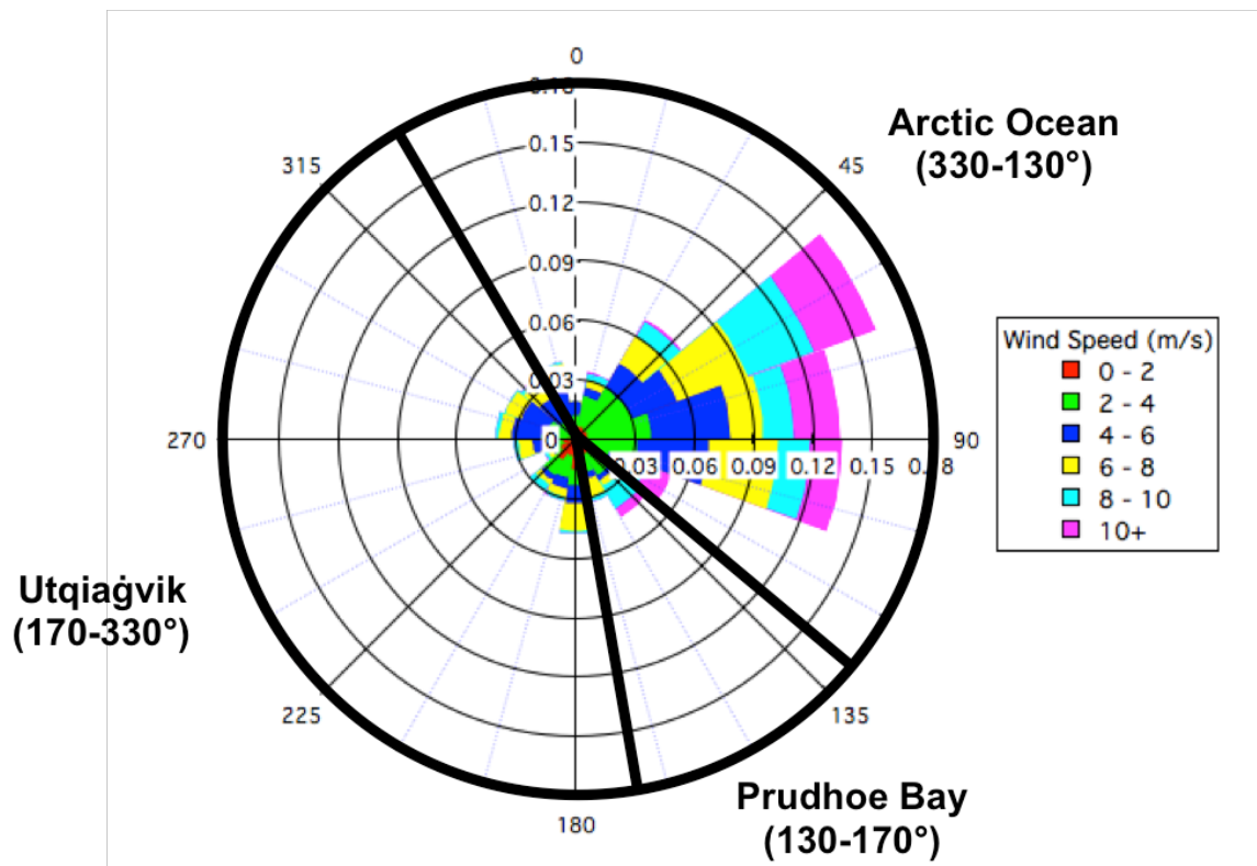
115 Figure S1. Wind rose from August 21–September 30, 2015 measured at the NOAA Barrow Observatory. Wind speed is binned by 2 m/s, and wind direction is binned by 20 degrees, with the radial axes representing the fraction of the study under those wind conditions.
