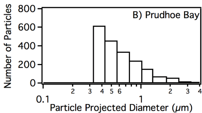
Figure S6. Numbers of particles, per particle projected diameter size bin, analyzed by CCSEM-EDX for (A) Arctic Ocean and (B) Prudhoe Bay air mass samples.
