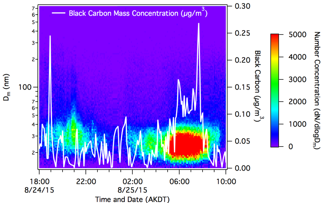
Figure S5. Aerosol size-resolved number concentrations (mobility diameter) measured by the SMPS during Prudhoe Bay air mass influence on August 24-25, 2015. Black carbon mass concentrations measured by the aethalometer are overlaid in white.
