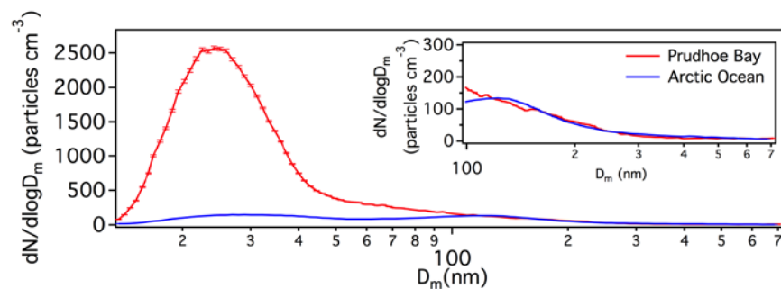
Figure 2. Average, and standard error of the mean, particle number size (14 – 746 nm mobility diameter) distributions during Prudhoe Bay and Arctic Ocean influenced air masses from August 21–September 20, 2015, with the above 100 nm distributions inset. The full time series of the time-varying aerosol distribution is shown in Figure S2.
