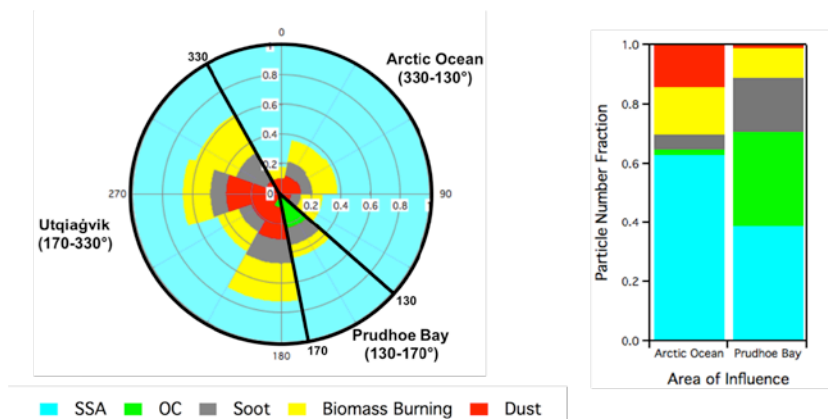
Figure 5. ATOFMS individual particle composition (0.2–1.5 \mu\text{m} ) number fractions for 496 analyzed particles from September 8–20, 2015, based on wind direction (left) and air mass influence (right), determined by backward air mass trajectories. Data were binned every 40 degrees.
