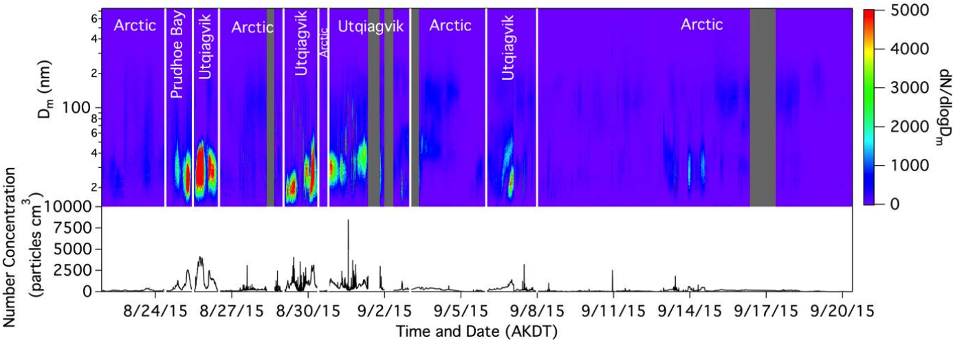
Figure S2. Aerosol size-resolved number concentrations (mobility diameter) measured by the SMPS from August 21-September 20, 2015. Identified air mass source regions, determined based on wind direction and backward air mass trajectories, are labeled and divided by white lines in the time series. Periods lacking data are indicated in gray. Total particle (0.013 – 746 nm) number concentrations are also shown.
