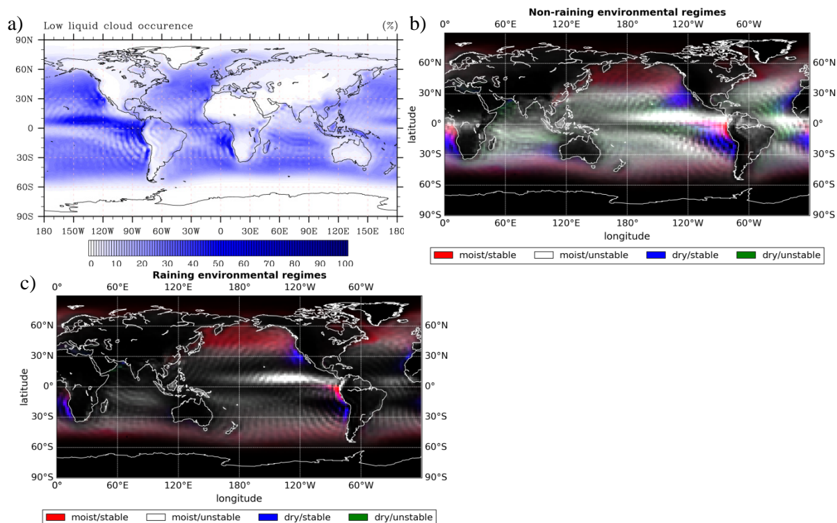
Figure 1: Average frequency of the occurrence of low liquid clouds (cloud top pressure > 500 hPa, cloud top temperature > 273.15 K) in E6_Ref between 1995 and 2012 in a) for all environmental regimes together, b) for non-raining regimes, c) for raining regimes.
