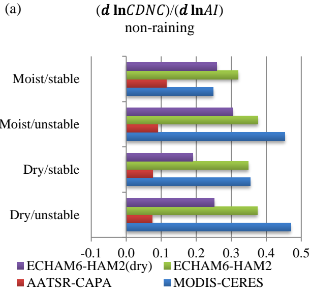
Figure 3: Susceptibility of CDNC to changes in AI for ECHAM6-HAM2 (E6_Ref), E6_Ref without aerosol water uptake (dry) during 1995-2012, for AATSR-CAPA using the full satellite record span 2002-2012 and for MODIS-CERES during 2006-2010. The definition of the different environmental regimes is given in the text. a) For all non-raining scenes, b) for all raining scenes. Only values averaged over global oceans are shown. The MODIS-CERES data is from Christensen et al. (2016).
