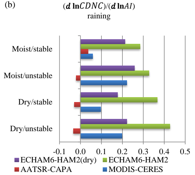
Figure 3: Susceptibility of CDNC to changes in AI for ECHAM6-HAM2 (E6_Ref), E6_Ref without aerosol water uptake (dry) during 1995-2012, for AATSR-CAPA using the full satellite record span 2002-2012 and for MODIS-CERES during 2006-2010. The definition of the different environmental regimes is given in the text. a) For all non-raining scenes, b) for all raining scenes. Only values averaged over global oceans are shown. The MODIS-CERES data is from Christensen et al. (2016).
