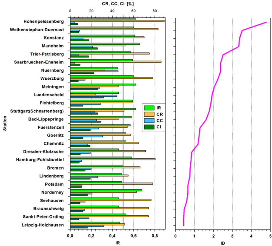
Figure 12. Visualization of the different scores described in Appendix C for all pyranometer stations. The stations are sorted by their \overline{ID} score with the station with the highest score on top.
