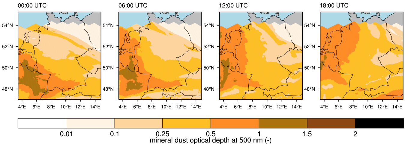
Figure 4. Mineral dust optical depth at 500 nm over Germany on 4 April 2014 at 00 UTC, 06 UTC, 12 UTC and 18 UTC (TT case). Note the saw-tooth shape in the northern part which marks the margin of the high resolution (5 km) domain and must not be confused with mineral dust-free conditions.
