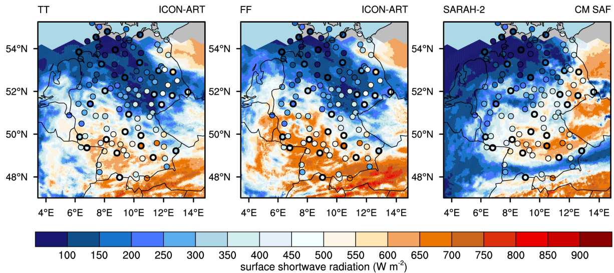
Figure 6. SIS of TT (left), FF (middle) and SARA-2 dataset by CM SAF (right) on 4 April 2014 at 12:30 UTC in Germany. Dots: SIS at SYNOP (thin circle lines) and pyranometer stations (thicker circle lines).
