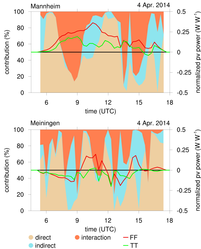
Figure 10. Temporal evolution of the difference in normalized PV power between TT and measurements (green line, right ordinate) and the corresponding difference between FF and measurements (red line, right ordinate) on 4 April 2014 at Mannheim (top) and Meiningen (bottom). Contours: percentaged contribution of direct radiative, indirect radiative and synergistic interaction effects to the change between TT and FF based on the FM calculation (left ordinate).
