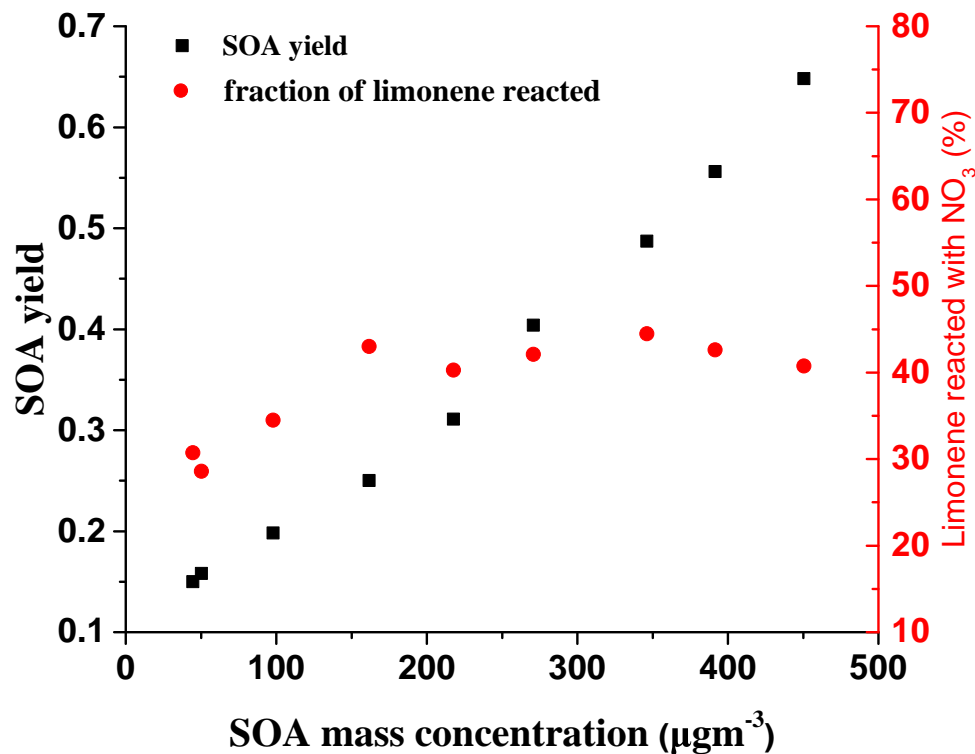
Fig. 1. Figure R1. The fraction of the limonene reacted with \text{NO}_3 (model study) and the corresponding SOA yields (experimental work) for Exp. N8-N16.
