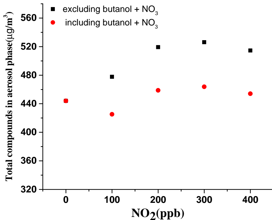
Fig. 2. Figure R2. Effect of the reaction of butanol + NO 3 on the particle mass. (∂ŪŪ the total compounds in aerosol phase including the butanol + NO 3 in the simulation, same as that shown in Fig 6c in the revis
