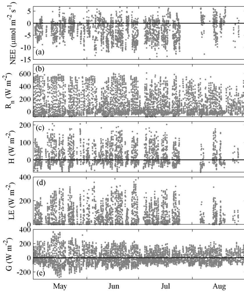
Figure 4: Time series of the 30-minute average surface fluxes measured with the eddy-covariance system: (a) net ecosystem exchange, (b) net radiation, (c) sensible heat, (d) latent heat, and (e) ground heat flux.
