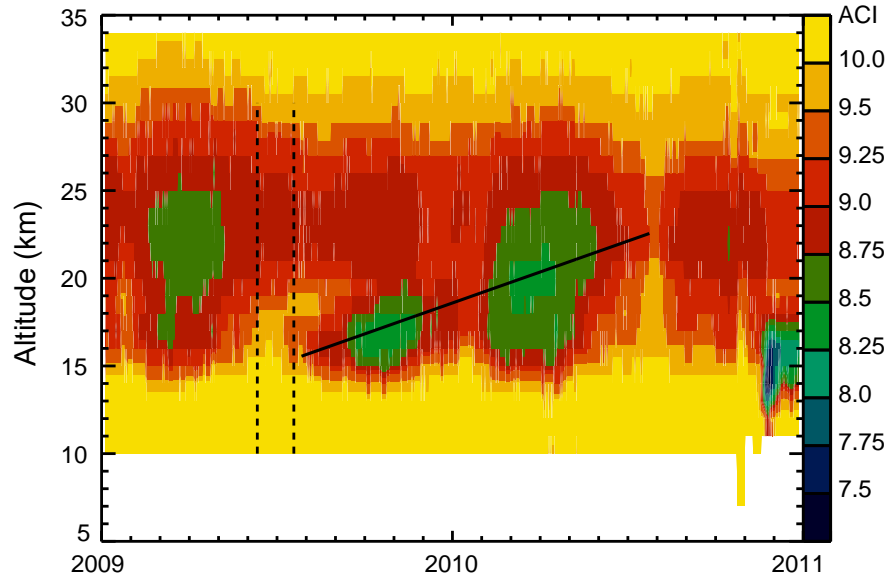
Figure 13: MIPAS nine-day running median of aerosol-cloud-index (ACI) between 10°N and 10°S (averaged along longitudes) from 2009 to 2010, overlaid with ascent speed of the water vapor tape recorder (solid line) derived with Aura Microwave Limb Sounder (MLS) water vapor mixing ratio from Glanville et al. (2017). Black dashed lines indicate the 12 June 2009 when the eruption started and 20 July 2009 when the simulations show first substantial aerosol transport to 10°N–10°S.
