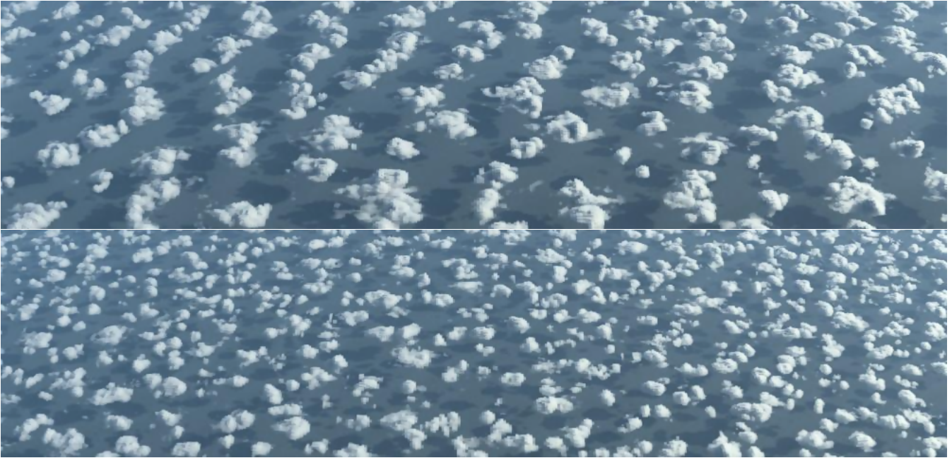
Figure 1. Virtual photograph of LES simulations at a cruising altitude of 15 km. Top panel: cloud formation of a simulation driven by 3D radiation (TenStream with sun in the east, i.e. right ( \varphi = 90^\circ )). Lower-panel: cloud formation of a simulation which was performed with 1D radiation (Two-stream). The specific model setup is the same as referenced in fig. 2, i.e., no background wind and a continental land surface. The simulations differ with respect to cloud size distributions and the organization in cloud streets, the cloud fraction though is the same (27 %). The visualization was performed with a physically correct rendering with MYSTIC (MonteCarlo solver in libRadtran (Mayer, 2009; Emde et al., 2015)).
