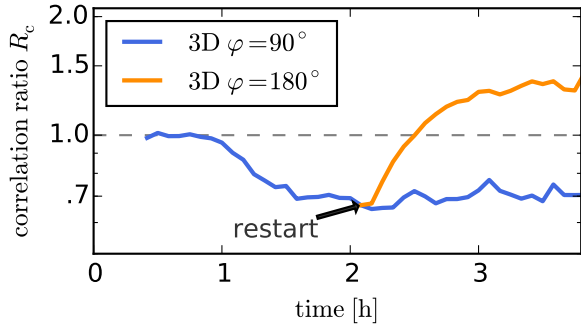
Figure 4. Time evolution of the correlation ratio R_c (e.g. as in fig. 2). The solar zenith angle is \theta = 40^\circ , there is no mean background wind speed ( u = 0 \text{ ms}^{-1} ) and the surface skin heat capacity is set to an equivalent of 1 cm water depth (representative for continental land surface). The radiative transfer is computed with the TenStream solver and the sun is positioned in the east ( \varphi = 90^\circ ) The first shallow cumulus clouds develop with a random orientation ( R_c = 1 ). The radiative response (i.e. surface shadows) changes the organization of convection to bands from north to south R_c < 1 in about one hour. Additionally, to examine the timescales of radiatively induced organization of convection, we perform a restart of the simulation with the sun positioned in the south ( \varphi = 180^\circ ). Once the sun is rotated, it takes the simulation again about one hour to change the orientation of convection into bands from east to west ( R_c > 1 ).
