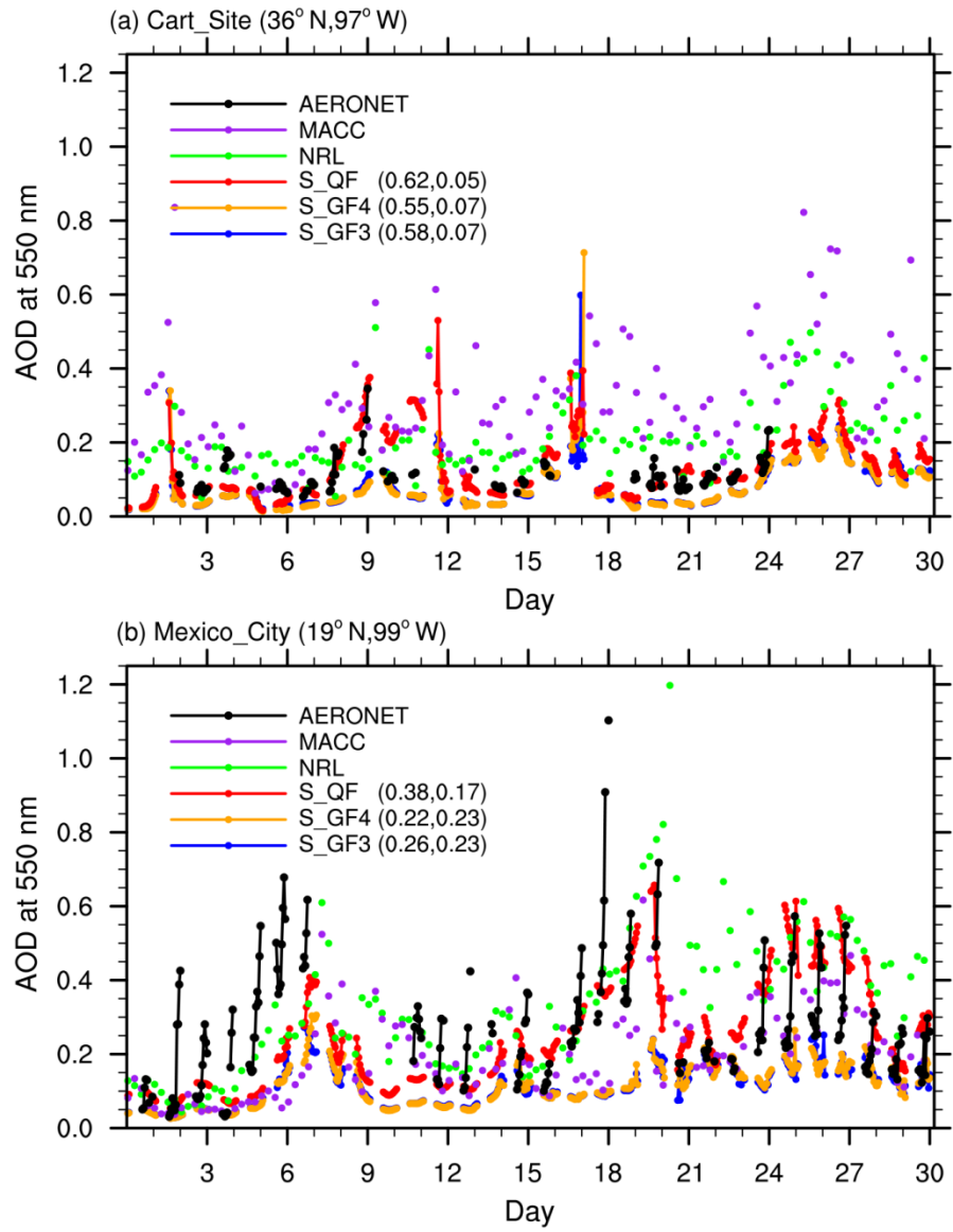
Fig.4. Time series of hourly regional mean AOD in April, 2009 from group A simulations, reanalysis data and AERONET retrievals at AERONET sites. Numbers in parenthesis denote TCC (left) and RMSE (right) between each simulation and AERONET AOD.
