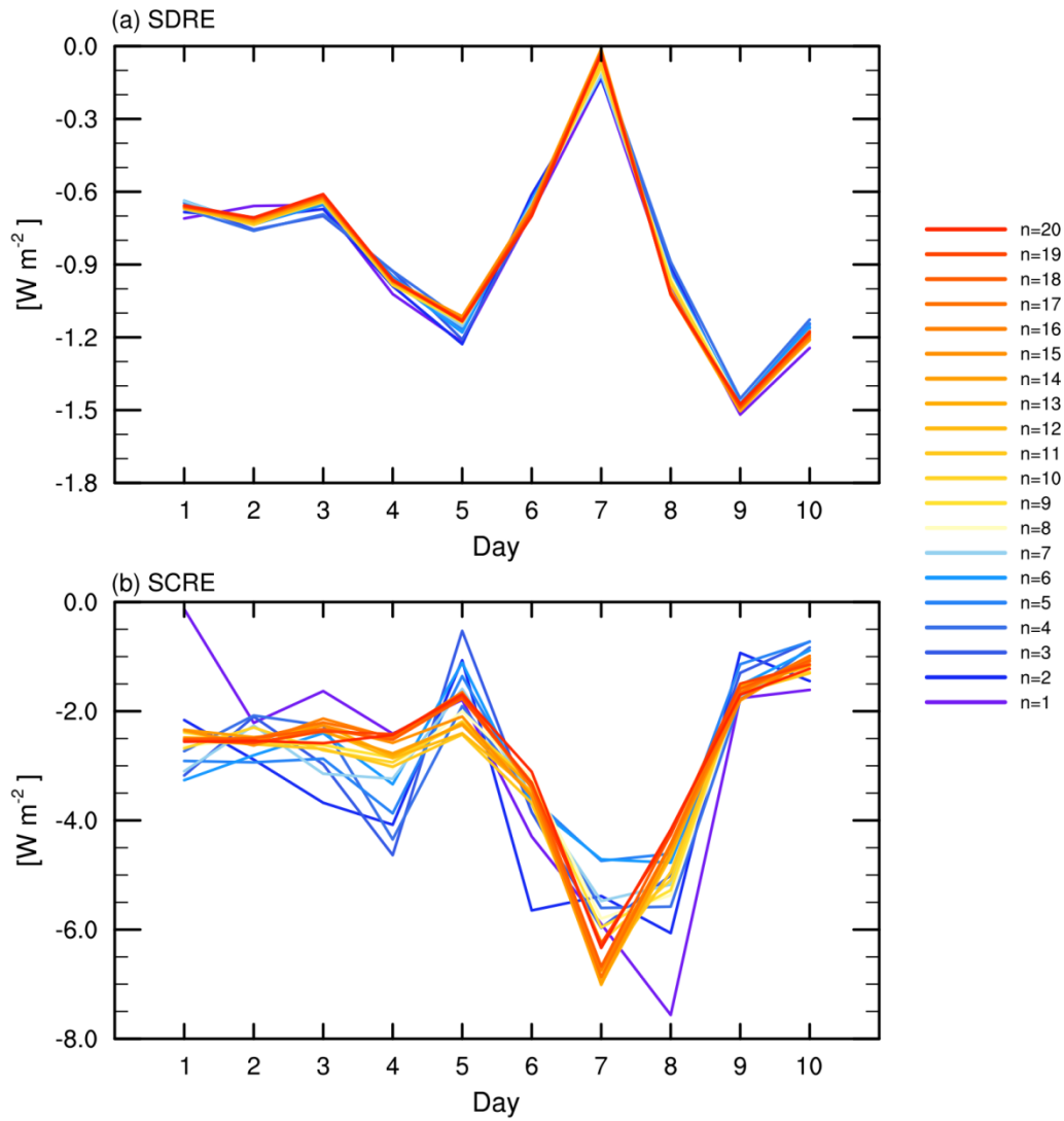
Fig.14. Time series of daily ensemble mean fire aerosol a) SDRE and b) SCRE averaged over Southern Mexico during Apr. 1-10, 2009 in QFED forced ensemble simulations with varying the total number of member numbers (n=1-20).
