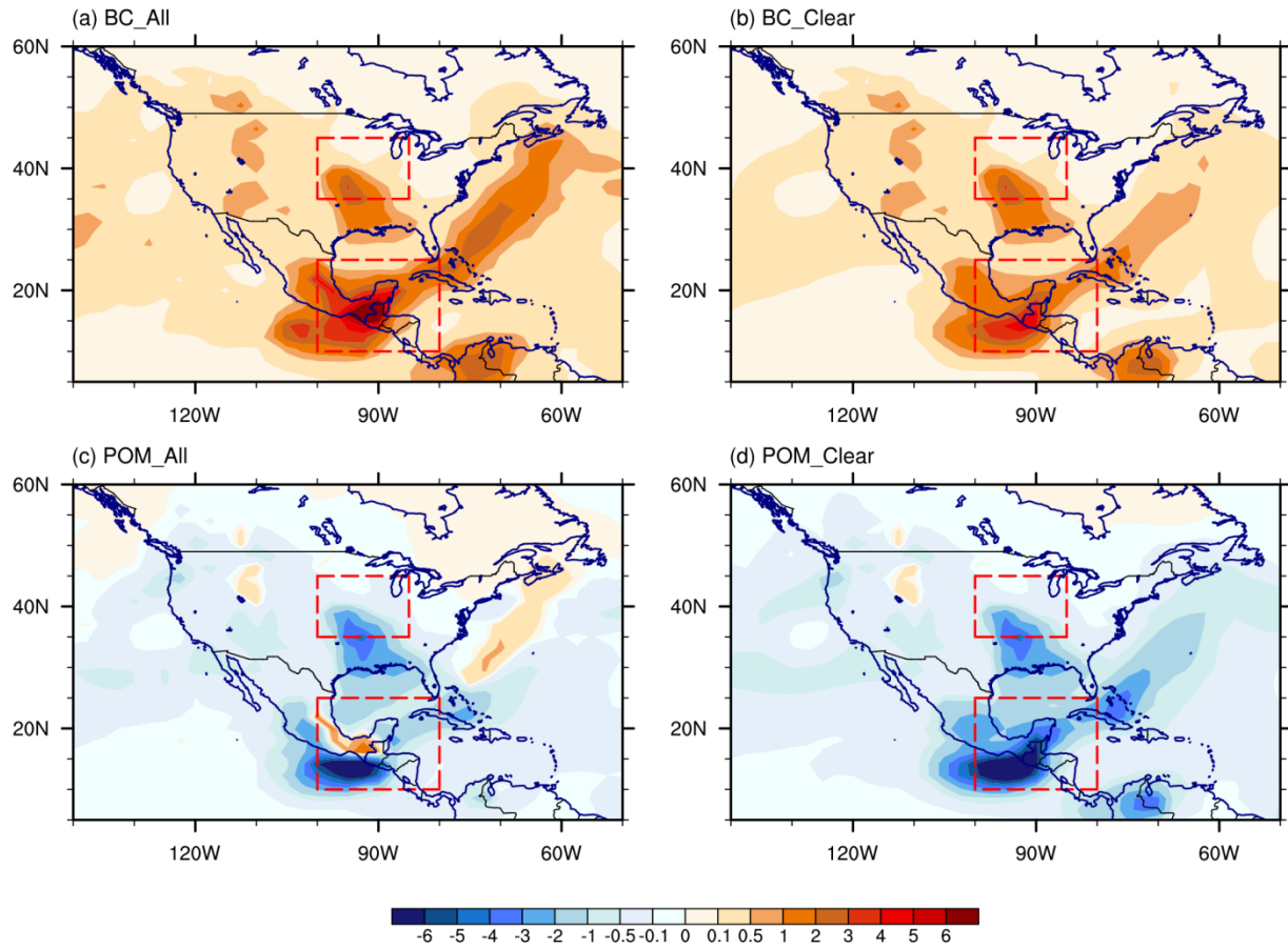
Fig.12. Spatial distributions of fire BC SDRE and fire POM SDRE ( W m^{-2} ) on all-sky and clear-sky conditions on April 7 in the E_QF simulation.
