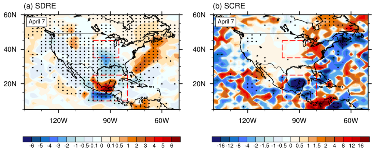
Fig.11. Spatial distributions of ensemble mean fire aerosol a) SDRE and b) SCRE ( W m^{-2} ) on April 7 in the E_QF simulation. Dots denote grids where fire aerosol effect is statistically significant at the 95% confidence level based on the KS test.
