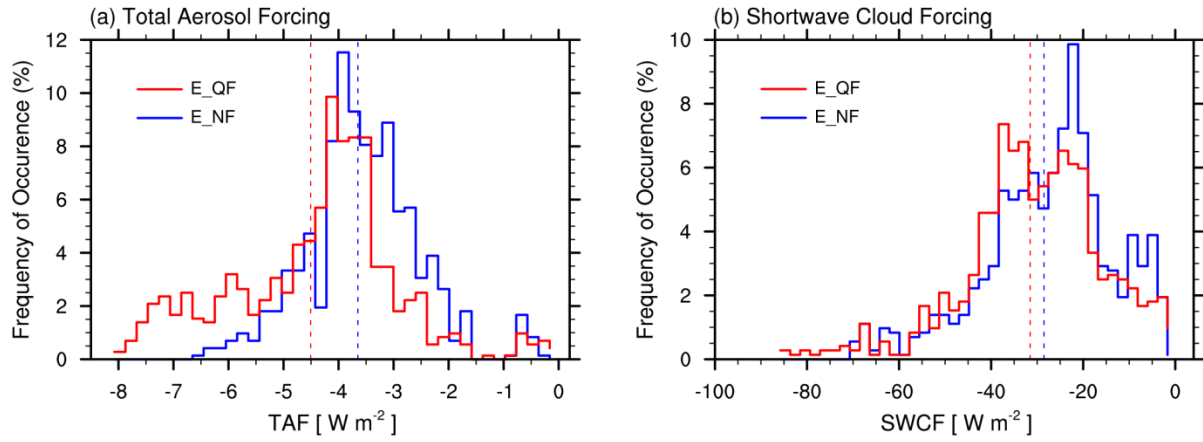
Fig. 9. Probability distributions of 10-day average (Apr.1-10) a) total aerosol forcing and b) cloud forcing over Southern Mexico in simulations E_NF and E_QF sampled from grid values of ensemble members (72x10 for each case). Dashed lines indicate the mean of the distribution.
