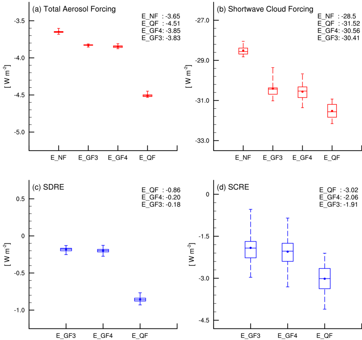
Fig.10. 10-day average (Apr. 1-10) regional mean a) total aerosol direct forcing, b) total shortwave cloud forcing and fire aerosol, c) SDRE, and d) SCRE in Southern Mexico in group B simulations. Box denotes the 25 th and 75 th percentiles. Bars outside the box indicate minimum and maximum. Bar within the box denotes the 50 th percentile. Total aerosol and cloud forcing are sampled from different ensemble members (10 for each case). Fire aerosol SDRE and SCRF are sampled by calculating the difference between members in simulations E_QF (E_GF3/E_GF4) and E_NF (10x10 for each case).
