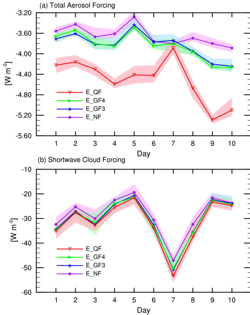
Fig.13. Time series of daily regional mean total a) aerosol forcing and b) cloud forcing in Southern Mexico during Apr.1-10, 2009 in group B simulations. Individual lines indicate ensemble mean values. Shaded areas illustrate the ensemble spread (from minimum to maximum).
