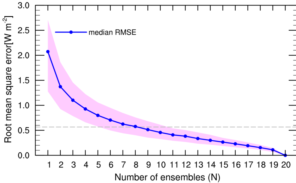
Fig.15. Root mean square errors (RMSE) of the ensemble mean of the regional mean fire aerosol SCRE during April 1-10 over Southern Mexico in simulations with different total number of ensemble members (N). The blue line represents the median RMSE of the 1000 groups (each group has N members/simulations). The grey line represents the threshold RMSE. Shaded area denotes the range between the 10 th and 90 th percentiles.
