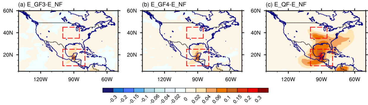
Fig. 6. Spatial distributions of 10-day average (Apr. 1-10) ensemble mean AOD differences between simulations with (E_GF3, E_GF4, and E_QF) and without fire emission (E_NF).
