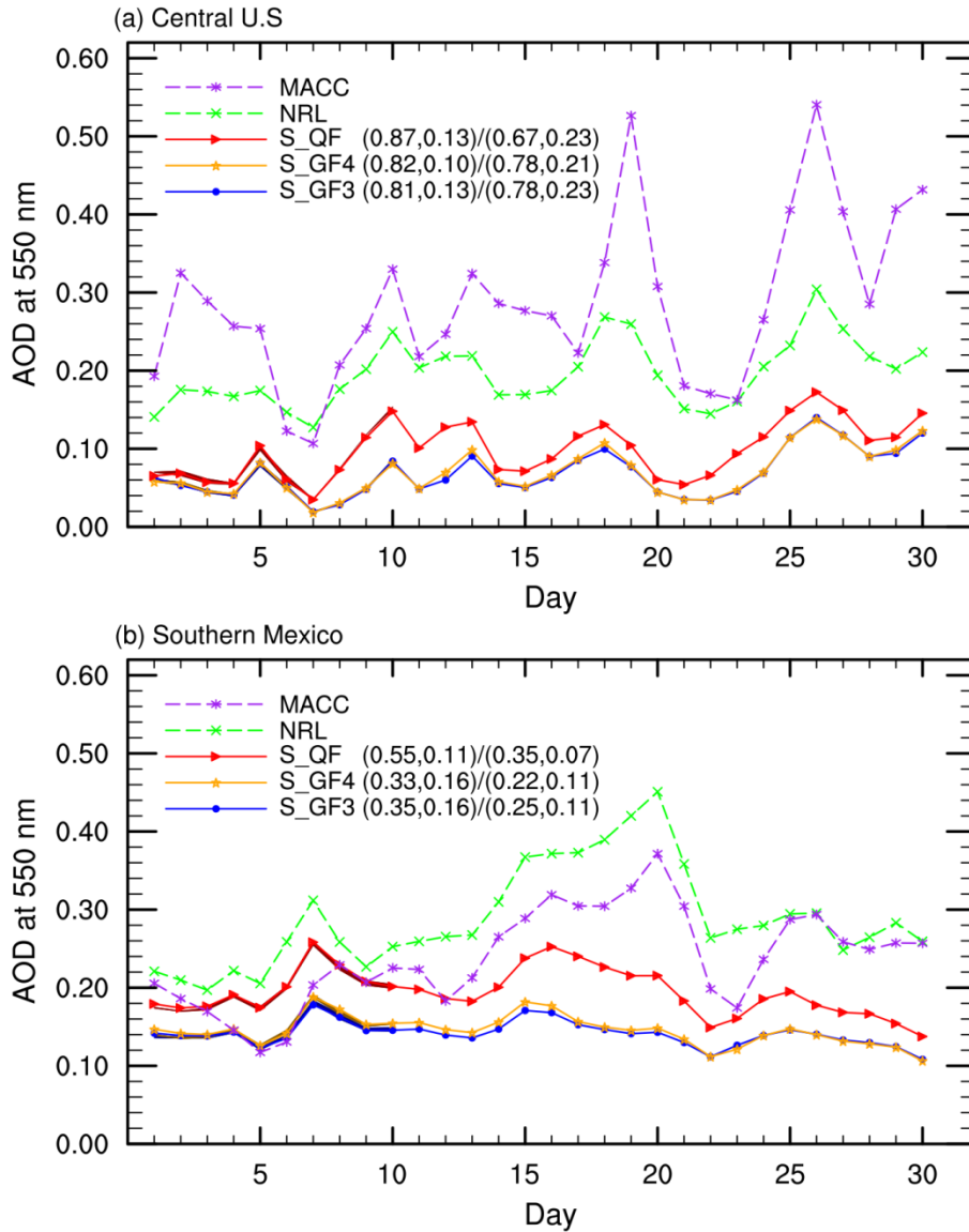
Fig.3. Time series of daily regional mean AOD in April, 2009 in simulations and reanalysis data. Numbers in parenthesis denote time correlation coefficient (TCC) and root mean square error (RMSE) between each simulation in group A and reanalysis data (left: NRL; right: MACC). Individual lines indicate group A simulations. Shaded areas (very narrow) in slightly darker colors during April 1-10 illustrate maximum and minimum values of daily mean AOD among ensemble members in group B simulations. For the single-member simulation and the ensemble simulation driven by same fire emission, the shaded area and the solid line almost overlap, given the barely indistinguishable AOD between ensemble members and the corresponding Group A simulation.
