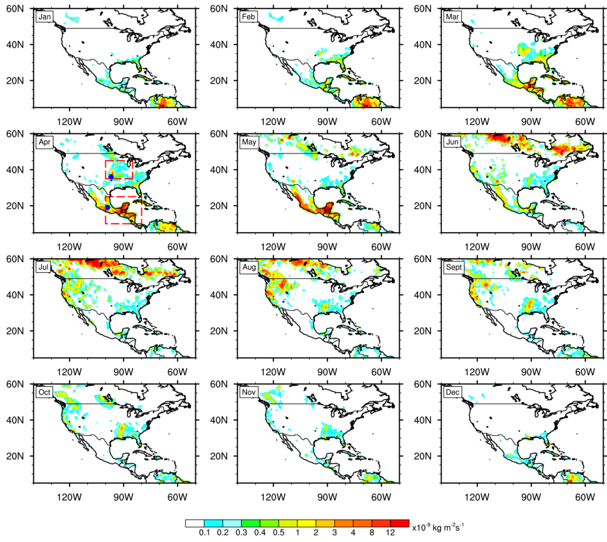
Fig.1. Spatial distributions of multi-year monthly mean biomass burning consumed dry matter over North America during 2003-2014 from GFEDv4.1. Boxes denote selected regions: central U.S (35 - 45°N, 85 - 100°W) and Southern Mexico (10 - 25°N, 80 - 100°W). Dots denote locations of AERONET sites: Cart_Site (36°N, 97°W) and Mexico_City (19°N, 99°W)
