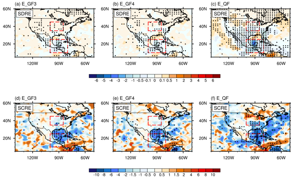
Fig. 7. Spatial distributions of 10-day average (Apr. 1-10) ensemble mean fire aerosol shortwave direct radiative effect (SDRE) and shortwave cloud radiative effect (SCRE) ( W m^{-2} ) in group B simulations. Dots denote regions where SDRE is statistically significant at the 95% confidence level based on the Kolmogorov-Smirnov (KS) test.
