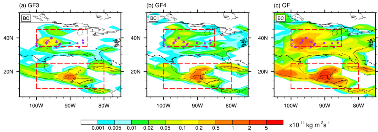
Fig.2. Spatial distributions of monthly mean BC emissions from three emission inventories in April, 2009. IMPROVE data sites are shown as asterisks for sites near the source region and as dots for sites in the region downwind of the fire source.
