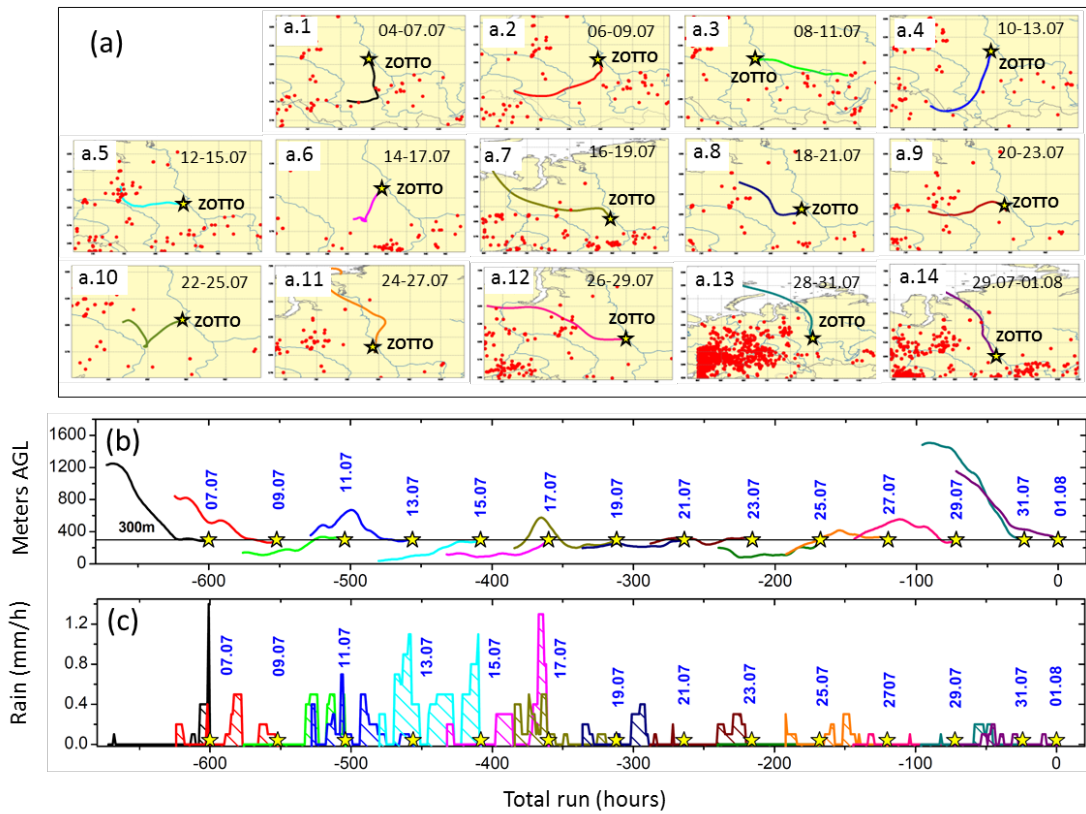
Figure 12. (a) 72-h HYSPLIT air mass trajectories with 48-h intervals during back-ground periods at ZOTTO at 300 m from 07 July to 01 August 2010; red dots indicate the fire locations within a 72 h period, (b) their height above ground level (AGL), and (c) precipitation rate along the air mass trajectories. Stars and dates show the arrival time of the air mass (b, c).
