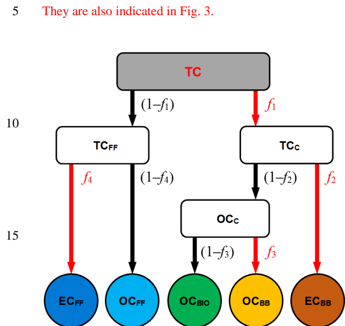
Figure 3. Source apportionment scheme based on the coupled radiocarbon-levoglucosan marker method for the relative contributions of EC and OC from fossil fuel (FF) combustion, biomass burning (BB) and biogenic sources (BIO) to the total carbon ( TC=EC+OC ). The multiplication factors are further explained in the text. The subscript C indicates contemporary carbonaceous fraction. The red arrows specify the input of the primary multiplication factors into the apportionment scheme.
