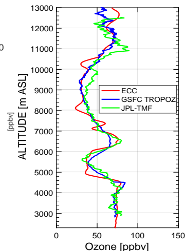
5 Figure 8: a) Time series of 10-min GSF TROPOZ lidar observations during the SCOOP campaign at JPL-Table Mountain Facility (TMF, site elevation: 2300 masl) along with six ECC sondes (denoted with triangles). b) Comparison of 30-min averaged ozone from GSF TROPOZ and JPL-TMF ozonlidars as compared to the last sounding of the time series. Courtesy: J. T. Sullivan, NASA/GSFC.
