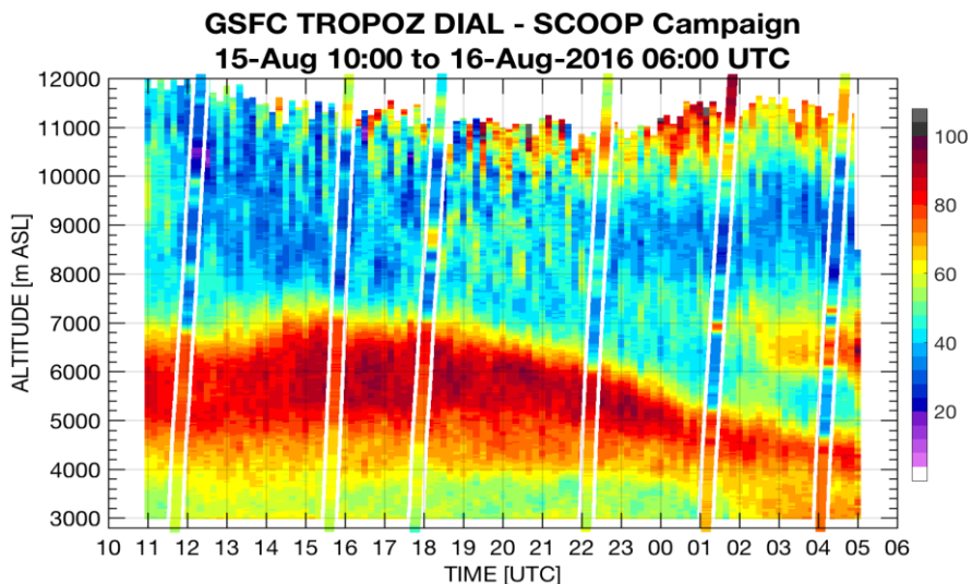
5 Figure 8: a) Time series of 10-min GSF TROPOZ lidar observations during the SCOOP campaign at JPL-Table Mountain Facility (TMF, site elevation: 2300 masl) along with six ECC sondes (denoted with triangles). b) Comparison of 30-min averaged ozone from GSF TROPOZ and JPL-TMF ozonlidars as compared to the last sounding of the time series. Courtesy: J. T. Sullivan, NASA/GSFC.
