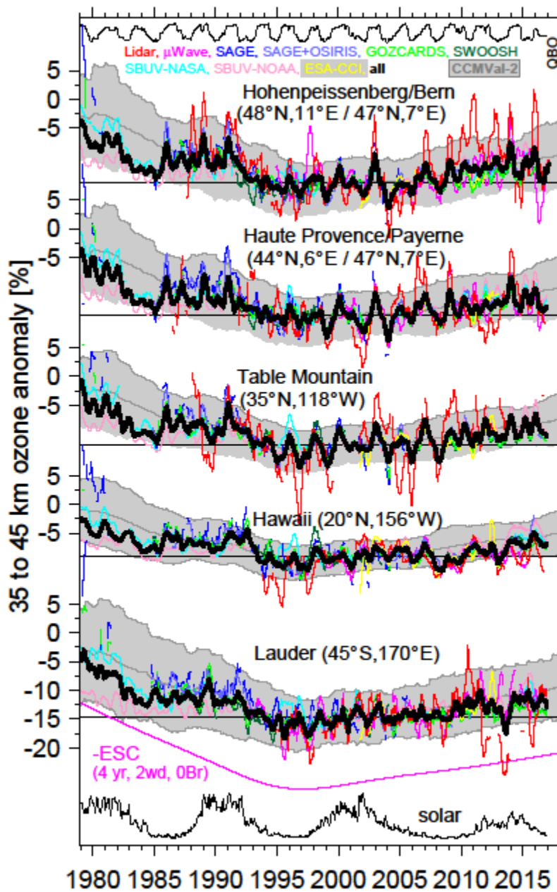
5 Figure 5: The essential synergism of NDACC measurements with data from satellites. The grey area shows the range of model evaluations from the CCMVal-2 initiative. Also shown at the top/bottom are the expected natural variability (QBO / solar cycle) and the evolution of ESC (effective stratospheric chlorine). The data are used for verifying successful implementation of the Montreal Protocol.
