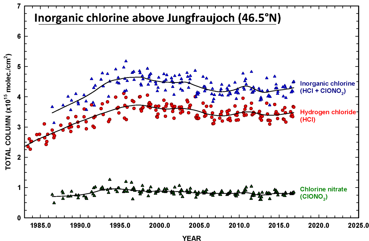
Figure 10: Inorganic chlorine above Jungfraujoch. Multi-decadal monthly mean total column time series of the two main chlorine reservoirs, hydrogen chloride (HCl; red circles) and chlorine nitrate (ClONO 2 ; green triangles), monitored at the Jungfraujoch station (Swiss Alps, 46.5°N, 3580 m a.s.l.) in the framework of the NDACC network. The data sets are restricted to the June to November months such as to limit the impact of variability caused by atmospheric transport and subsidence mainly during winter-springtime. A good proxy of northern midlatitude total inorganic chlorine (Cly) is obtained by summing the HCl and ClONO 2 total columns (see blue triangles). The thin continuous lines correspond to non-parametric least square fits involving an integration time of about 3-year, they help appraising a non-monotonous decrease of chlorine in the stratosphere after 1996-1997. Using the 1997.0 Cly column as reference and the bootstrap resampling tool of Gardiner et al. (2008), a mean post-peak rate of change of -(0.50 \pm 0.15) %/yr is obtained for the 1997-2016 time period. Courtesy: E. Mahieu et al., Univ. Liège.
