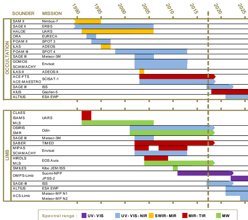
Fig. 6b: Low Earth Orbit limb-viewing satellite profilers supported by NDACC, from the inception of the NDSC through present day and beyond. Upper chart: solar (and stellar) occultation instruments measuring in the UV / VIS / NIR (typically O 3 , NO 2 , BrO, H 2 O, aerosols...) and the MIR / TIR (typically O 3 , NO, NO 2 , HNO 3 , CH 4 , CO, H 2 O, CFC-11, CFC-12, aerosols...) Lower chart: limb-scanning instruments measuring scattered light solar radiation (typically O 3 , NO 2 , H 2 O, aerosols...), MIR / TIR emission (typically O 3 , NO, NO 2 , HNO 3 , N 2 O, CH 4 , CO, H 2 O, HCl, ClONO 2 , CFC-11, CFC-12, aerosols...) and MW emission (typically O 3 , HCl, ClO, N 2 O, H 2 O, HNO 3 ...)
