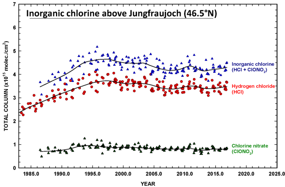
Figure 10: Inorganic chlorine above Jungfraujoch. Multi-decadal monthly mean total column time series of the two main chlorine reservoirs, hydrogen chloride (HCl; red circles) and chlorine nitrate (ClONO 2 ; green triangles), monitored at the Jungfraujoch station (Swiss Alps, 46.5°N, 3580 m a.s.l.) in the framework of the NDACC network. The data sets are restricted to the June to November months such as to limit the impact of variability caused by atmospheric transport and subsidence mainly during winter-springtime. A good proxy of northern midlatitude total inorganic chlorine (Cly) is obtained by summing the HCl and ClONO 2 total columns (see blue triangles). The thin continuous lines correspond to non-parametric least square fits involving an integration time of about 3-year, they help appraising a non-monotonous decrease of chlorine in the stratosphere after 1996-1997. Using the 1997.0 Cly column as reference and the bootstrap resampling tool of Gardiner et al. (2008), a mean post-peak rate of change of -(0.50 \pm 0.15) %/yr is obtained for the 1997-2016 time period. Courtesy: E. Mahieu et al., Univ. Liège.
