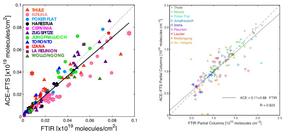
Figure 7. Examples of the validation of new satellite datasets. The left panel is reprinted from [Clerbaux et al., 2008] for lower stratospheric CO measured at 5\mu\text{m} , from 11 instruments, 9 of which are located at NDACC stations. The partial column quantities from the ACE-FTS and the FTIR have very similar characteristics in vertical resolution and analysis providing a precise evaluation of satellite performance. The latitudinal extent of the NDACC sites here from 76^\circ\text{N} to 34^\circ\text{S} help verify the ACE-FTS global coverage. The right panel reprinted from [Wolff et al., 2008] shows the correlation of partial columns for \text{HNO}_3 measured at 10.02\mu\text{m} from 9 NDACC stations from 76^\circ\text{N} to 78^\circ\text{S} .
