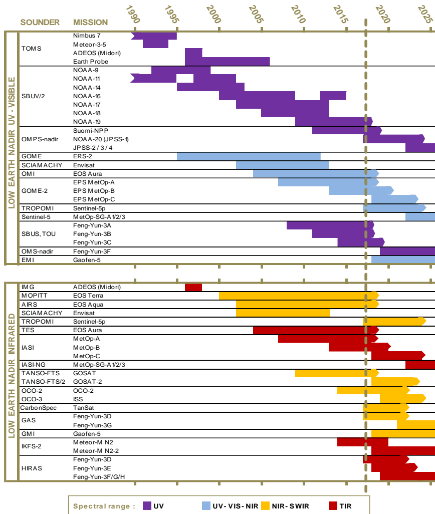
Figure 6a: Low Earth Orbit nadir-viewing satellite sounders supported by NDACC, from the inception of the NDSC through present day and beyond. Upper chart: backscatter UV (O 3 ) and UV / VIS (O 3 , NO 2 , BrO, HCHO...) Lower chart: backscatter NIR / SWIR (typically CH 4 , CO, H 2 O, N 2 O) and MIR / TIR emission (O 3 , CH 4 , CO, N 2 O, H 2 O, HNO 3 , HCl, CFC-11, CFC-12...)
