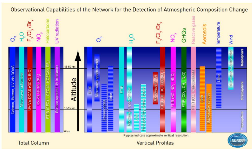
10 Figure 1: NDACC measurement capabilities, including species and parameters measured, instrumental measurement techniques, and each measurements' approximate vertical resolution (indicated by the ripple).
