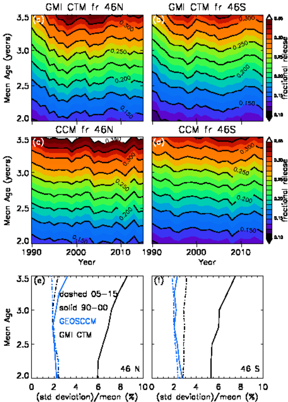
Figure 2: Contours of the evolution of fractional release for N_2O simulated by GMI CTM for 1990 – 2015 as a function of mean age at (a) 46°N and (b) 46°S. Same for the GEOSCCM at (c) 46°N and (d) 46°S. The ratio of the standard deviation of the N_2O fractional release to the mean value from GMI CTM (black) and from GEOSCCM (blue) averaged from 1990 – 2000 (solid) and from 2005 – 2015 at (e) 46°N and (f) 46°S.
