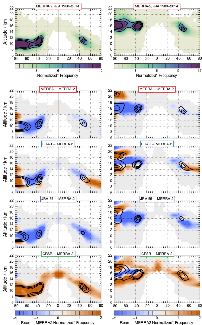
Figure 10. As in Figure 8, but for multiple tropopause frequency distributions. Primary tropopause frequencies are shown on the left and secondary tropopause frequencies on the right. Overlaid contours are frequencies of 6, 9, and 12%.
