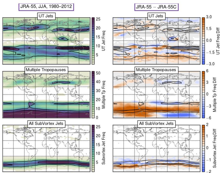
Figure 5. Seasonal maps for JJA in 1980 through 2012 of JRA-55 (left) and the difference between JRA-55 and JRA-55C (right). Layout is as in Figure 1.
