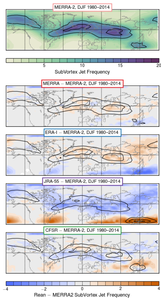
Figure 11. As in Figure 7, but for NH subvortex jet frequency distributions in DJF. The latitude domain shown is north of 30°N. Overlaid contours are frequencies of 10, 15, and 20% for each reanalysis.
