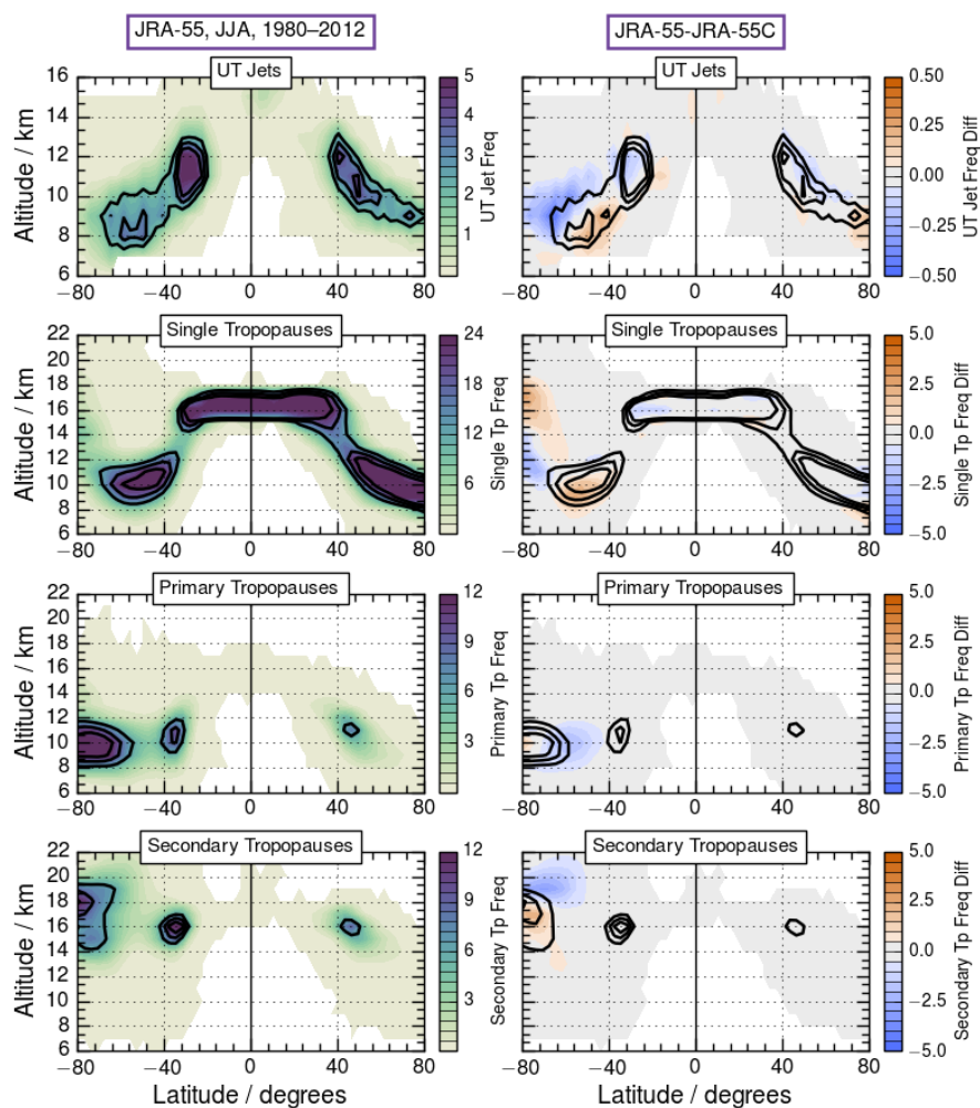
Figure 6. Seasonal cross-sections for JJA in 1980 through 2012 of JRA-55 (left) and the difference between JRA-55 and JRA-55C (right). Layout is as in Figure 2.
