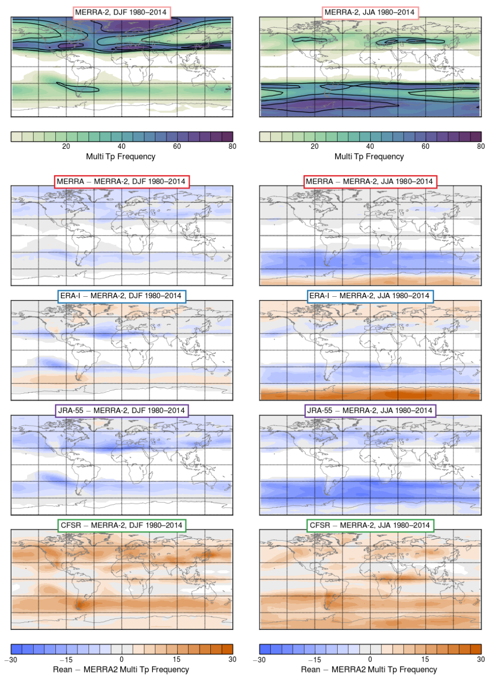
Figure 9. As in Figure 7, but for multiple tropopause frequency distributions. Overlaid contours show frequency values from each reanalysis of 30, 45, and 60%.
