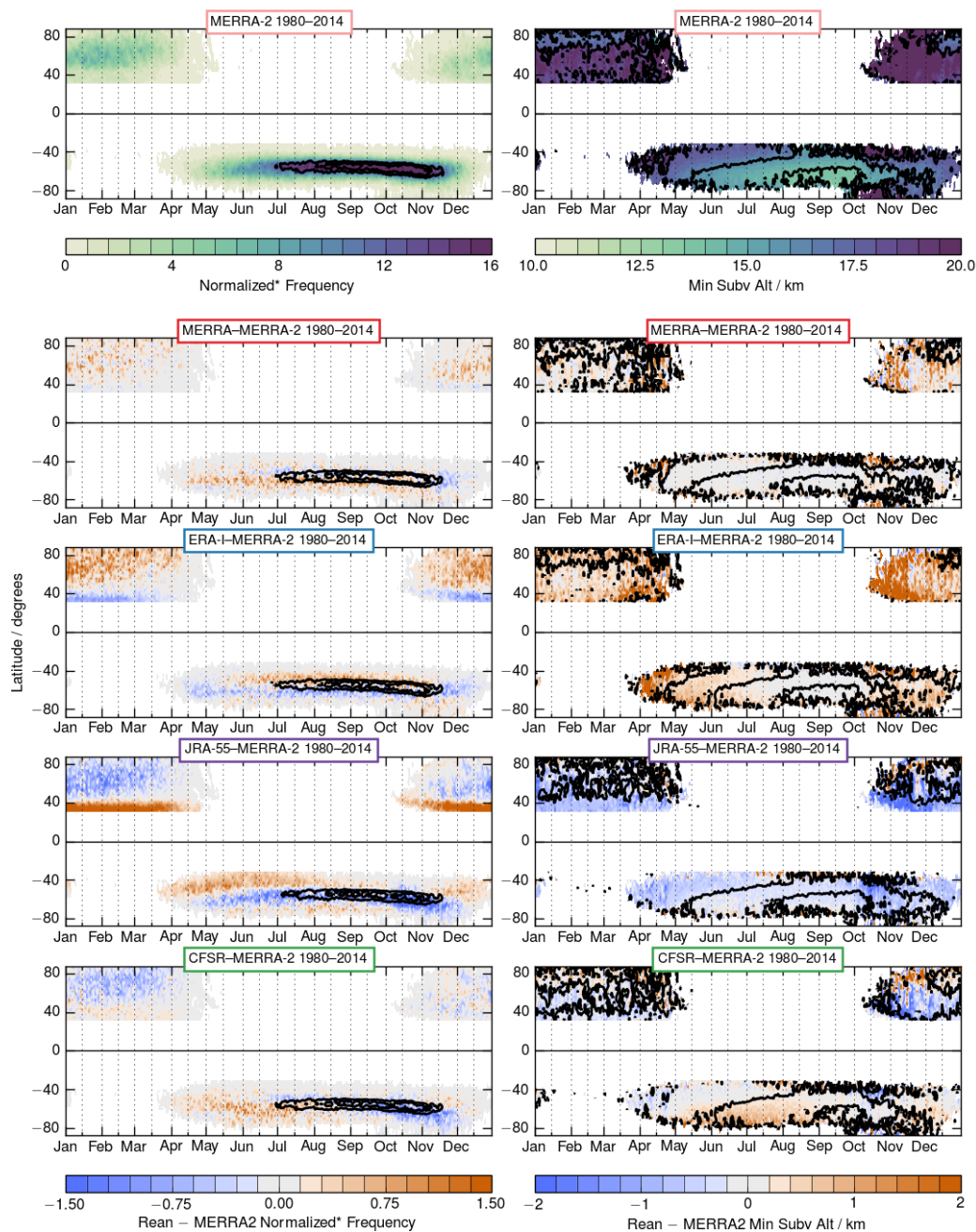
Figure 16. As in Figure 13 but for merged subvortex jets, with merge altitude on the right. Overlaid contours are 12 and 16% for frequencies and 14 and 18 km for merge altitudes.
