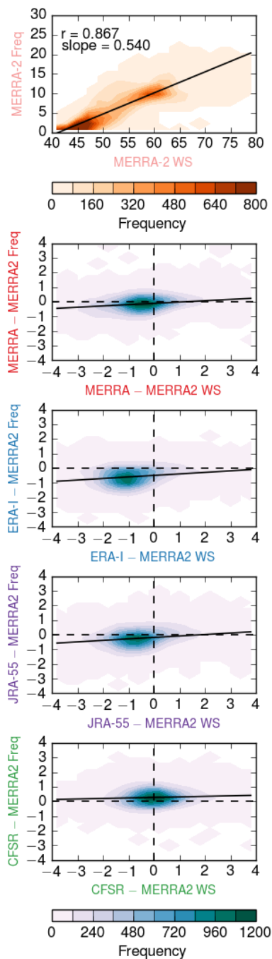
Figure 14. Density plots of (top) MERRA-2 climatological daily jet frequencies versus climatological daily jet windspeeds (values are from Figure 13), and of the corresponding (reanalysis – MERRA-2) frequency differences versus jet windspeed differences for (second to fifth rows) MERRA, ERA-I, JRA-55, and CFSR. Black lines are the linear fit to the distributions.
