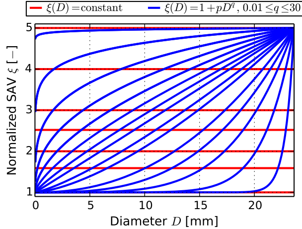
Figure 4. Synthetically generated \xi(D) relationships for deriving normalized snowflake surface-area-to-volume ratio \xi from snowflake diameter D by Eq. (7) with D \leq D_{\max} = 23.6 mm. Shown \xi(D) curves reflect the total range of \xi(D) relationships used for modeling snowfall triple-frequency radar signatures in Sect. 4.2.
