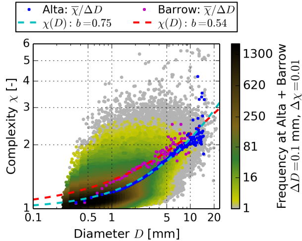
Figure 3. Logarithmic 2D histogram for all MASC data of snowflake diameter D and complexity \chi presented in Fig. 2, with bin sizes of \Delta D = 0.1 mm and \Delta\chi = 0.01 . Mean complexity values per size bin are indicated by \bar{\chi}/\Delta D for snowflake data recorded at Alta and at Barrow separately. Snowflake complexity–diameter relationships \chi(D) for the data sets collected at Alta and at Barrow are determined by the non-linear least squares method for fitting Eq. (2) to the values of \bar{\chi}/\Delta D and characterized by the power-law exponent b .
