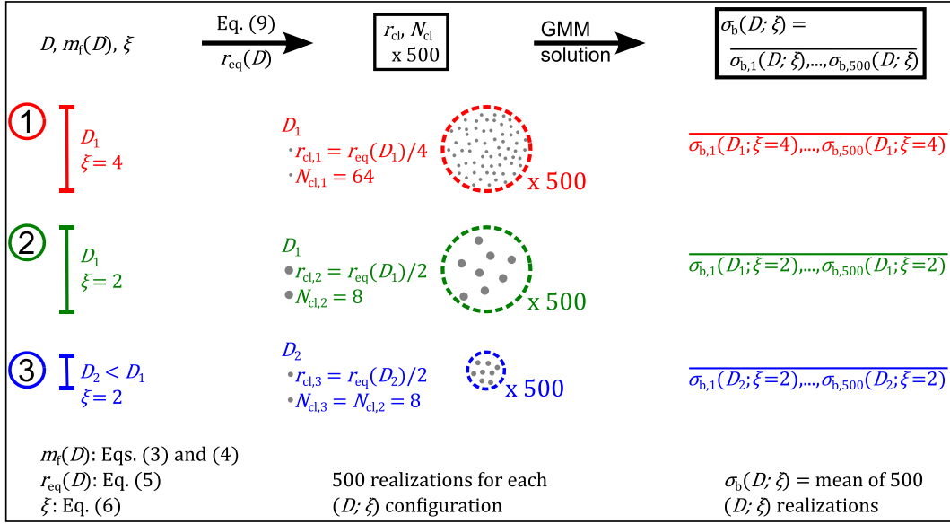
Figure 5. Sketch of the modeling approach described in Sect. 3.3, with three examples highlighted in red, green, and blue. The impact of normalized snowflake surface-area-to-volume ratios of 1 \leq \xi \leq 5 on modeled snowflake backscatter cross sections \sigma_b is investigated by applying the generalized multiparticle Mie (GMM) solution to collections of randomly distributed ice spheres characterized by the radius r_{cl} and the number N_{cl} of the constituent ice spheres and by the snowflake diameter D indicating the spherical bounding volume of the ice sphere collections.
