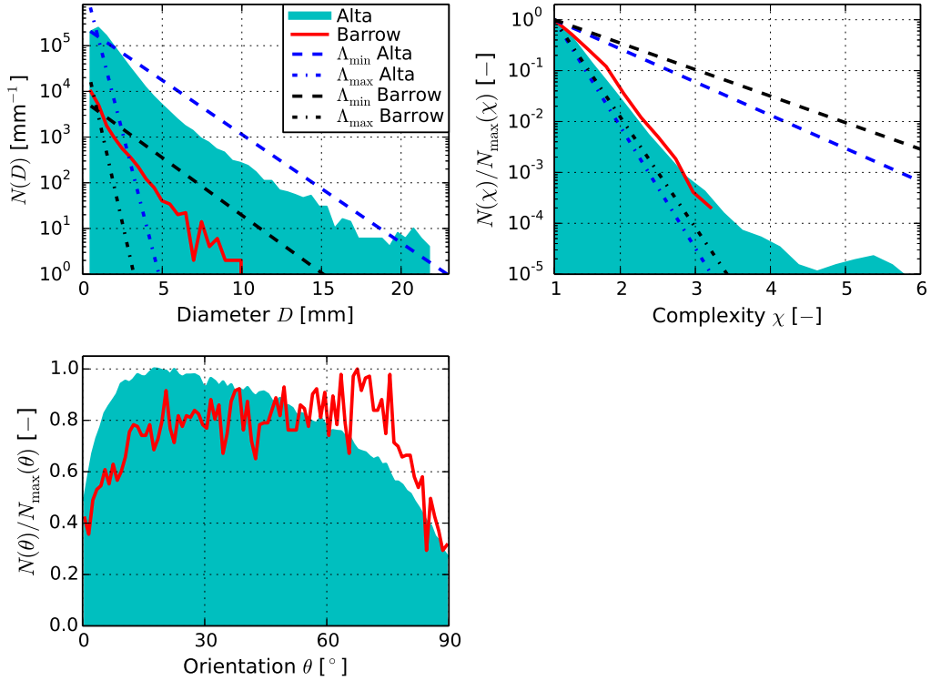
Figure 2. Snowflake (frequency) size distributions N(D) and relative distributions of snowflake complexity \chi and orientation \theta for 4.4 \cdot 10^5 snowflakes sampled by MASC at Alta and Barrow. Dashed lines represent minimum and maximum slope parameters \Lambda_{\min} and \Lambda_{\max} of exponential snowflake size distributions N(D) and exponential complexity distributions N(\chi) fitted to 47 snowstorms at Alta and to 7 snowstorms at Barrow. The number of recorded extreme values outside the plotted range is 33 for D and 43 for \chi . Mean orientation angles at Alta and at Barrow are \bar{\theta} = 40^\circ and \bar{\theta} = 45^\circ , respectively. Numerical values of \Lambda_{\min} , \Lambda_{\max} , and mean \bar{\Lambda} are given in the text.
