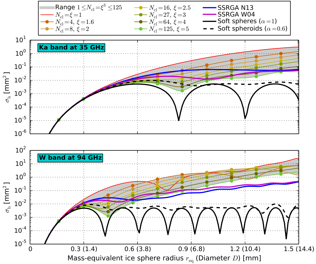
Figure 6. Modeled snowflake backscatter cross sections \sigma_b at 35 and 94 GHz for (i) collections of 1 \leq N_{cl} \leq 125 randomly distributed ice spheres inside a spherical bounding volume of diameter D , corresponding to normalized surface-area-to-volume ratios of 1 \leq \xi \leq 5 , for (ii) the self-similar Rayleigh–Gans approximation (SSRGA) applied to N13 and to W04 snowflake 3D shape models, and for (iii) soft spheres and oblate spheroids with aspect ratios of \alpha = 1 and \alpha = 0.6 , respectively. Results for (single) mass-equivalent ice spheres given by N_{cl} = 1 , for snowflakes modeled according to the SSRGA, and for soft ice spheres and spheroids were calculated at a resolution of \Delta r_{eq} = 0.01 mm. For collections of N_{cl} = 4, 8, 16, 27, 64 , and 125 ice spheres, dots mark values of \sigma_b(D; \xi) that were calculated at a resolution of \Delta r_{eq} \approx 0.14 mm following Sect. 3.3, and lines indicate spline interpolations of the calculated \sigma_b(D; \xi) . Modeled \sigma_b for the full range of considered snowflake diameters D \leq 23.6 mm, for soft spheroids characterized by extreme aspect ratios of \alpha = 0.2 , and for microwave frequencies of 10 and 14 GHz are shown in Fig. S3 in the Supplement.
