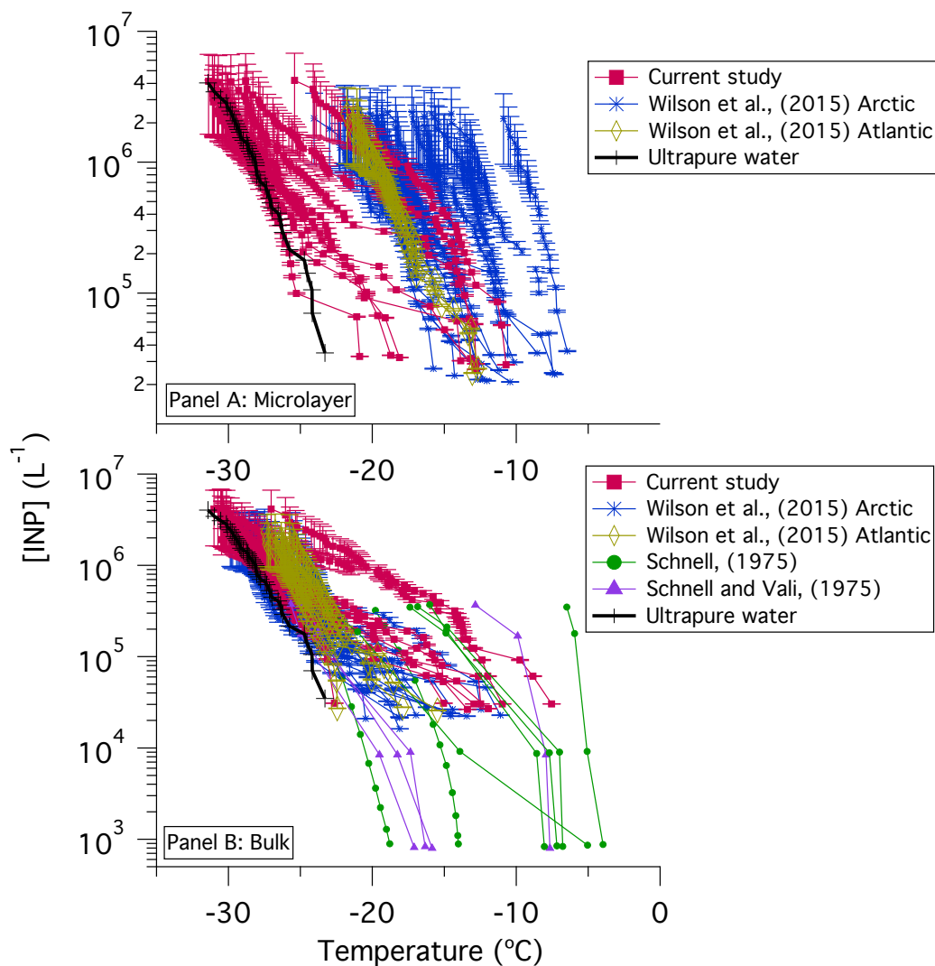
Figure 4 - The concentrations of INPs per volume of sample [INP] in the microlayer (Panel A) and bulk seawater samples (Panel B). All data, including those from other studies, are corrected for freezing point depression.
