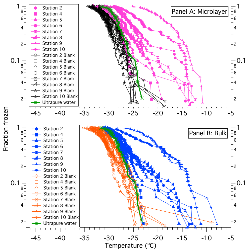
Figure 2 - Fraction of droplets frozen (in the immersion mode) versus temperature. Panel A and Panel B correspond to the microlayer and bulk seawater, respectively. Also included are the respective blank samples and ultrapure water. Each data point corresponds to a single freezing event in the experiments. All microlayer and bulk seawater freezing points have been corrected for freezing point depression to account for dissolved salts in seawater (Section 2.2.4).
