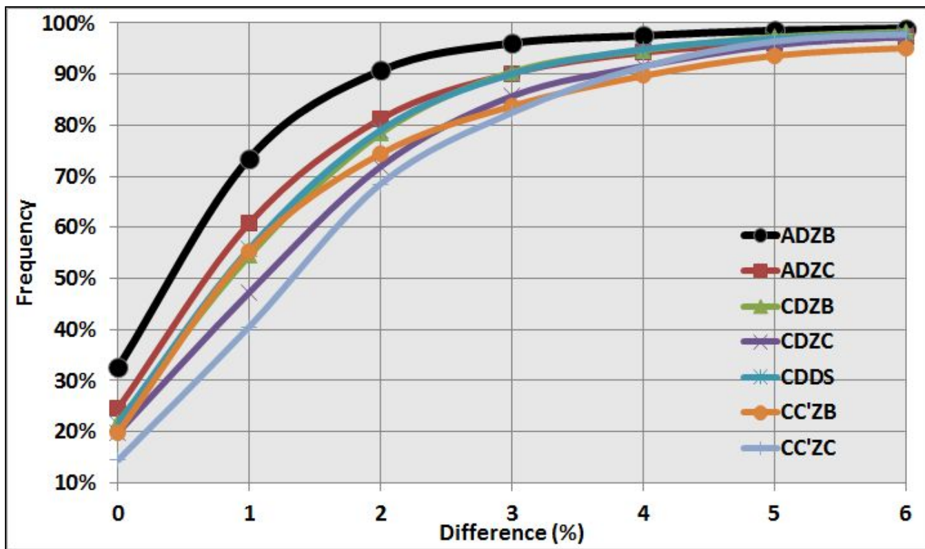
Figure 2. Distribution of cumulative differences between results from direct sun (ADDS) compared to zenith measurements on the same day. The frequency of compared zenith and ADDS total ozone (y-axes) is accumulated between 0 to 6 % (X-axes). Results are shown for other types of zenith sky measurements denoted by colors in the legend. Results are the average of 12 stations in the US network except for the CC' results, which is based on the SPO data record.
