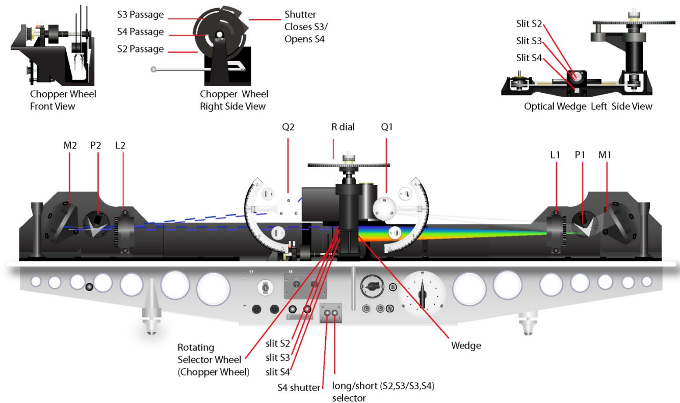
Figure 1: Diagram of Dobson Instrument, with cover omitted from view (some components shown are actually mounted in the cover.)
