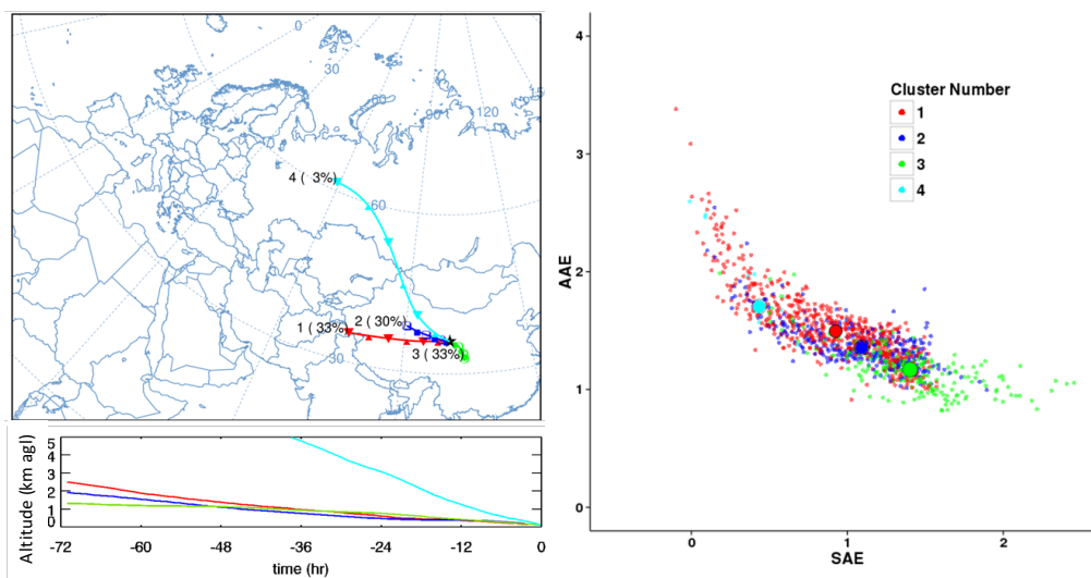
5 Figure 4. Back trajectory map, back trajectory height (in kilometers above ground level) vs. time, and AAE vs. SAE plot space for Mt. Waliguan, China station WLG, all color coded by back trajectory cluster number. The percentage of air-mass back trajectories corresponding to each cluster are also shown next to the mean trajectories.
