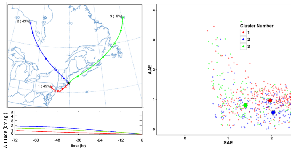
5 Figure 6. Back trajectory map, back trajectory height (in kilometers above ground level) vs. time, and AAE vs. SAE plot space for Cape Cod, Massachusetts, USA station PVC, all color coded by back trajectory cluster number
