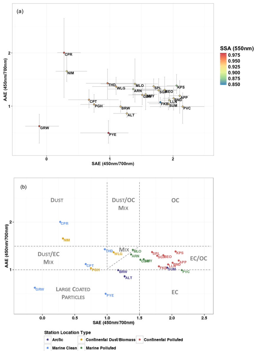
5 Figure 2. AAE vs. SAE medians plotted for 24 in situ monitoring stations in the NOAA/ESRL federated network. (a) Bars represent interquartile values, and points are color coded by median SSA value at the station, (b) Points are color coded by station location type, and plot is overlaid with aerosol classification matrix from Cazorla et al. (2013)
