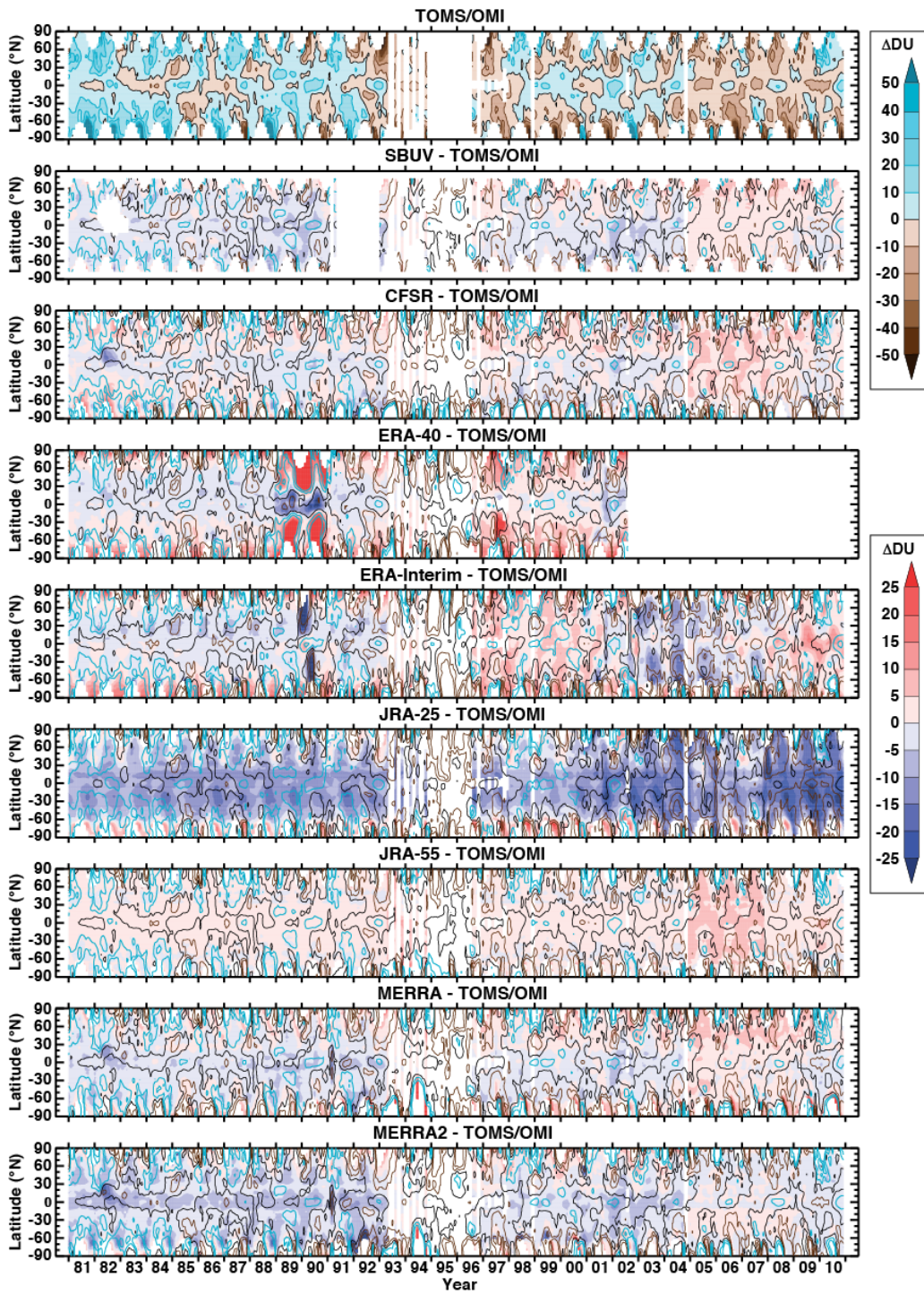
Figure S5: TO latitude vs. time anomalies for TOMS/OMI (top row), differences between SBUV and TOMS/OMI (second from top), and differences between TOMS/OMI and the reanalyses (other rows).
