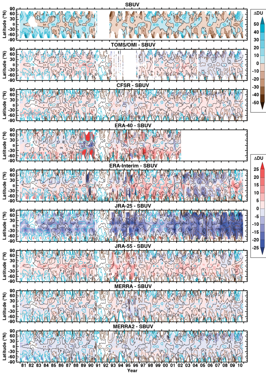
Figure S4: TOC latitude vs. time anomalies for SBUV (top row), differences between TOMS/OMI and SBUV (second from top), and differences between SBUV and the reanalyses (other rows).
